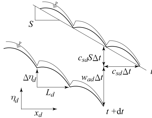
Figure 5. Conceptual diagram for bed erosion in the presence of steps.
