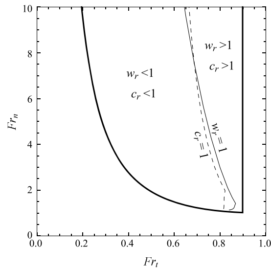
Figure 11. The boundary between the ranges where w_r > 1 and w_r < 1 , and the boundary between the ranges where c_r > 1 and c_r < 1 . L_{mr} = 0.1 and u_c = 0.5 . The range w_r > 1 ( w_r < 1 ) corresponds to an incision rate that is enhanced (suppressed) by the presence of steps, and the range c_r > 1 ( c_r < 1 ) corresponds to an upstream migration rate that is enhanced (suppressed) by the presence of steps.
