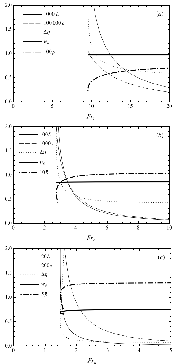
Figure 9. Parameters for cyclic steps as functions of Fr_n for the cases (a) Fr_t = 0.2 , (b) Fr_t = 0.4 , and (c) Fr_t = 0.6 ; L_{mr} = 0.1 , u_c = 0.5 . Note that while values of the vertical axis are constant, the variables are multiplied by different coefficients in the three plots in order to show all the variables in one figure.
