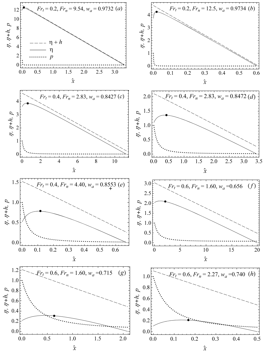
Figure 10. Profiles of the bed elevation \eta , the water surface elevation \eta + h , and the cover fraction p over a single cyclic step for L_{mr} = 0.1 , u_c = 0.5 , and (a) Fr_t = 0.2, Fr_n = 9.54, w_a = 0.9732 ; (b) Fr_t = 0.2, Fr_n = 12.5, w_a = 0.9734 ; (c) Fr_t = 0.4, Fr_n = 2.83, w_a = 0.8427 ; (d) Fr_t = 0.4, Fr_n = 2.83, w_a = 0.8472 ; (e) Fr_t = 0.4, Fr_n = 4.40, w_a = 0.8553 ; (f) Fr_t = 0.6, Fr_n = 1.60, w_a = 0.656 ; (g) Fr_t = 0.6, Fr_n = 1.60, w_a = 0.715 ; (h) Fr_t = 0.6, Fr_n = 2.27, w_a = 0.740 . The solid, dashed and thick dotted lines indicate \eta , \eta + h , and p , respectively, and the dot denotes the point where the Froude-critical condition is achieved. Figures 10a and 10b show cases of relatively small sediment supply, and relatively mild and steep cases, respectively. Figures 10c–10e show cases of medium sediment supply; Figures 10c and 10d are cases of the same mean bed slope but different values of w_a , and Figure 10e is a case of a steeper slope. Figures 10f–10h are cases of large sediment supply; Figures 10f and 10g are cases of the same slope but different values of w_a , and Figure 10h is a case of a relatively steep slope. Note that the vertical scale varies between panels.
