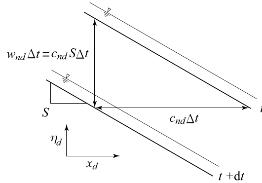
Figure 4. Conceptual diagram for bed erosion in the absence of steps.
