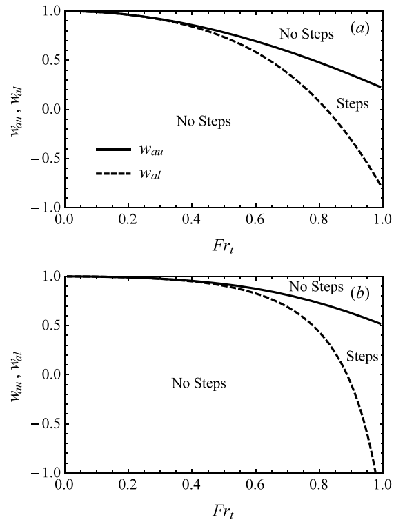
Figure 7. Lower and upper limits w_{au} and w_{al} on w_a as functions of Fr_t for the cases (a) L_{mr} = 0.1 , u_t = 0.2 , and (b) L_{mr} = 0.1 , u_t = 0.8 . The solid and dashed lines correspond to w_{au} and w_{al} , respectively.
