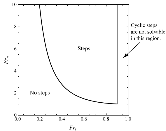
Figure 8. Solution domains on the Fr_t - Fr_n plane for cyclic steps for the case for which L_{mr} = 0.1 and u_c = 0.5 .
