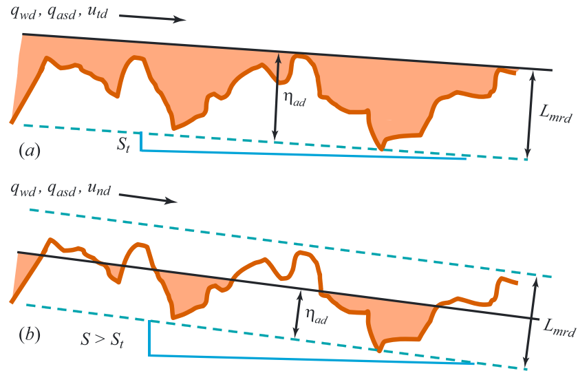
Figure 3. Definition diagram for (a) normal threshold state with bed slope S_t at which the bed is barely alluviated and (b) normal equilibrium state with S > S_t , so that the bedrock is only partially covered with alluvium. All other parameters remain the same for Figures 3a and 3b.
