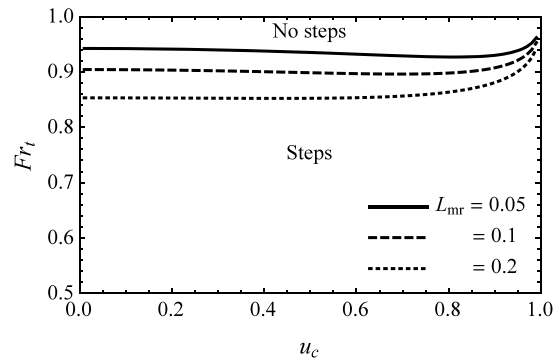
Figure 6. Upper limit of Fr_t as a function of u_c and L_{mr} .
