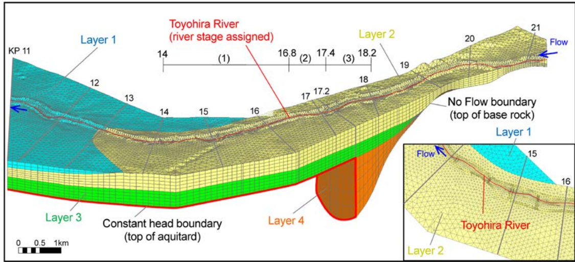
Fig. 6 Numerical groundwater flow model in the Toyohira River alluvial fan.
