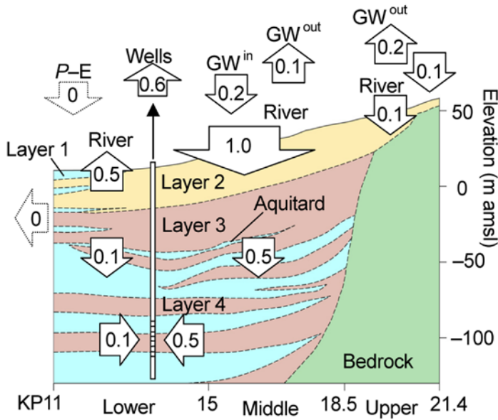
Fig. 10 Schematic subsurface groundwater budgets in the Toyohira River alluvial fan, obtained by modifying the longitudinal and vertical scales in Fig. 2. The values in arrows are rounded to one order of magnitude in cubic meters per second. GW^{in} and GW^{out} denote groundwater recharge from the east side and discharge to the west side, respectively.
