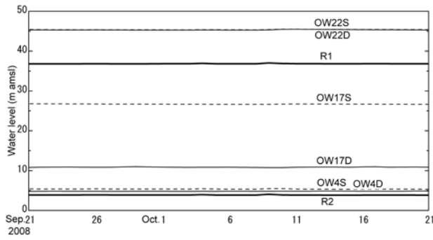
Fig. 4 Observed variations in water levels at gauging stations and observations wells. The locations of gauging stations and monitoring wells are shown in Fig. 1.
