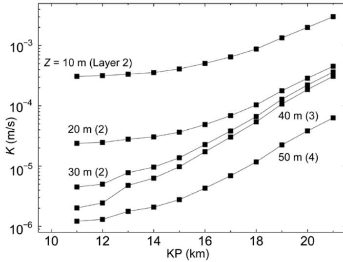
Fig. 7 Longitudinal distributions of hydraulic conductivity at different depths Z per ten meters with layer numbers (Layers 2, 3, and 4).
