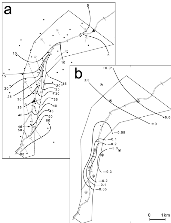
Fig. 5 Contour maps of (a) WTE and (b) VHG during a drought period for analysis. The monitoring wells correspond with those in Fig. 1. WTE contours are illustrated per 5 m amsl. Negative (positive) values of VHG indicate downward (upward) hydraulic gradient (dimensionless).
