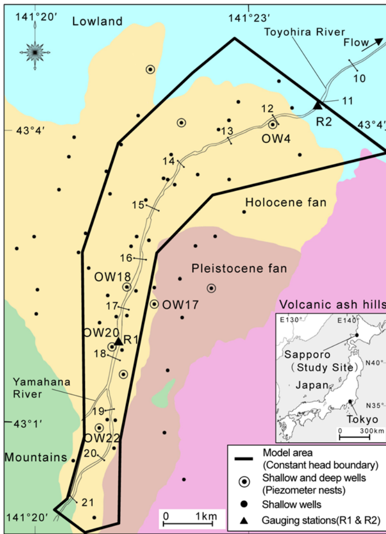
Fig. 1 Location maps and topographic features of the study area, the Toyohira River alluvial fan. The black lines across the river indicate the distance in kilometers, denoted as KP throughout the text. Gauging stations R1 and R2 are located on the river at KP 17.8 and KP 11, respectively. Sky blue, yellow, brown, purple, and green denote topographic features: the low land, Holocene fan, Pleistocene fan, volcanic ash hills, and mountains, respectively.
