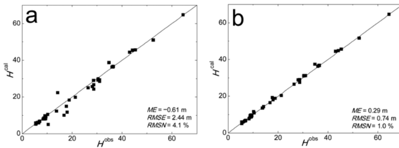
Fig. 8 Relations between simulated heads H^{cal} and observed heads H^{obs} at 43 monitoring wells using (a) the initial model and (b) the optimized model.
