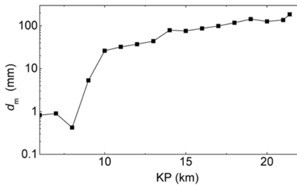
Fig. 3 A longitudinal distribution of the median grain size of the bed material in each kilometer (KP) along the Toyohira River.
