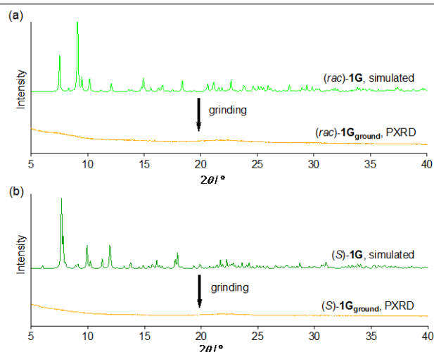
Fig. 3 PXRD pattern changes from (a) (rac) -1G (light green line, simulated pattern) to (rac) -1G ground (orange line) and (b) (S) -1G (green line, simulated pattern) to (S) -1G ground (orange line).
