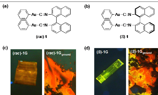
Fig. 1 Structure of (a) ( rac )- 1 and (b) ( S )- 1 . Photographs of (c) ( rac )- 1G and ( rac )- 1G ground and (d) ( S )- 1G and ( S )- 1G ground taken under ultraviolet irradiation ( \lambda_{\text{ex}} = 365 nm).
