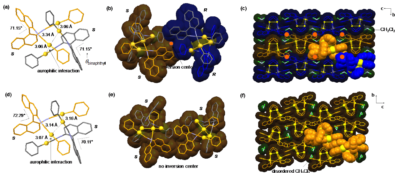
Fig. 2 Single-crystal structures of (a–c) ( rac )- 1G , and (d–f) ( S )- 1G . (a) Dimer, (b) tetramer, and (c) layer structures of ( rac )- 1G . (d) Dimer, (e) tetramer, and (f) layer structures of ( S )- 1G . All H atoms were omitted for clarity.
