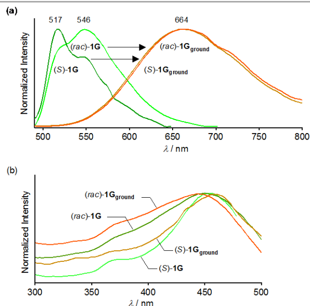
Fig. 4 (a) Emission spectra changes from (rac) -1G to (rac) -1G ground , and from (S) -1G to (S) -1G ground ( \lambda_{\text{ex}} = 365 nm). (b) Excitation spectra of (rac) -1G, (S) -1G, (rac) -1G ground , and (S) -1G ground obtained at each \lambda_{\text{em,max}} .
