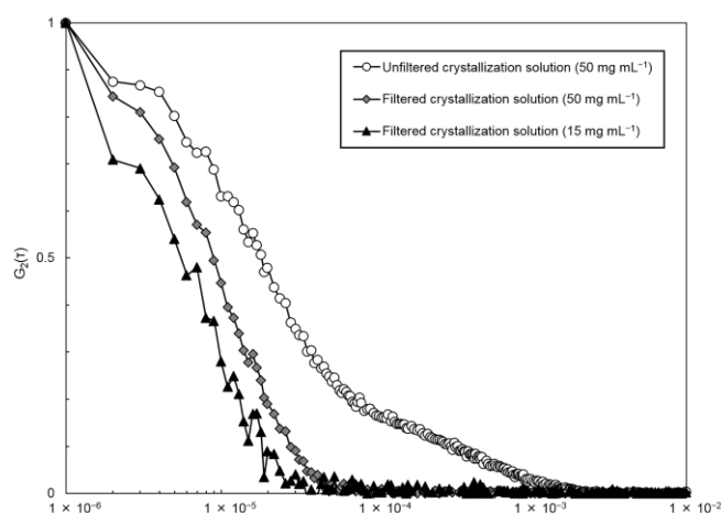
Figure S2. Normalized intensity correlation functions of lysozyme solutions.
