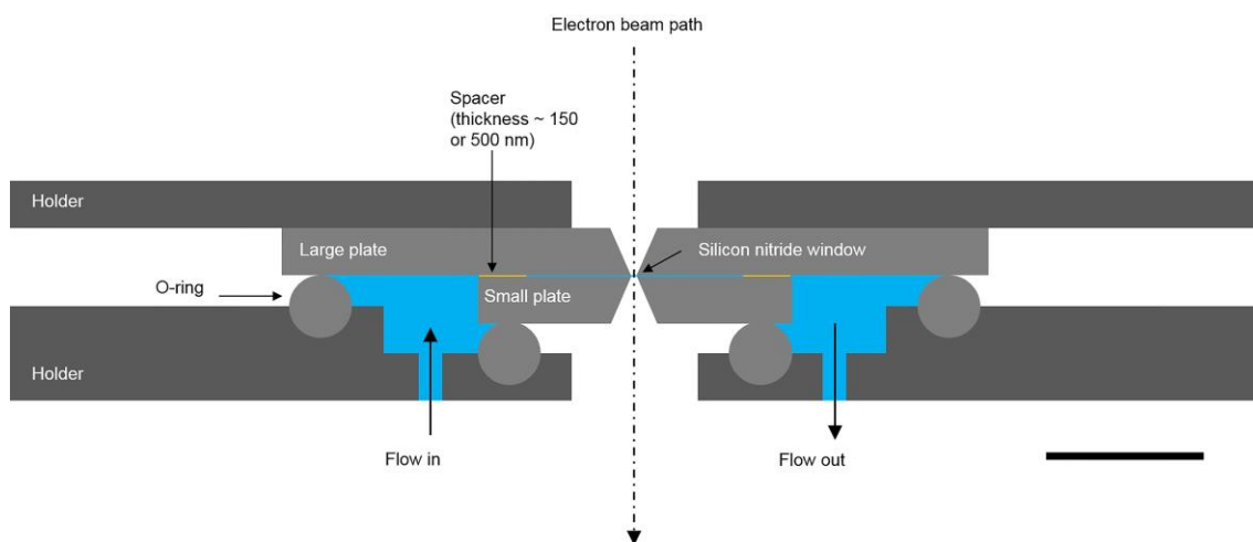
Figure S1. Schematic image of the liquid cell for in situ TEM observations.
