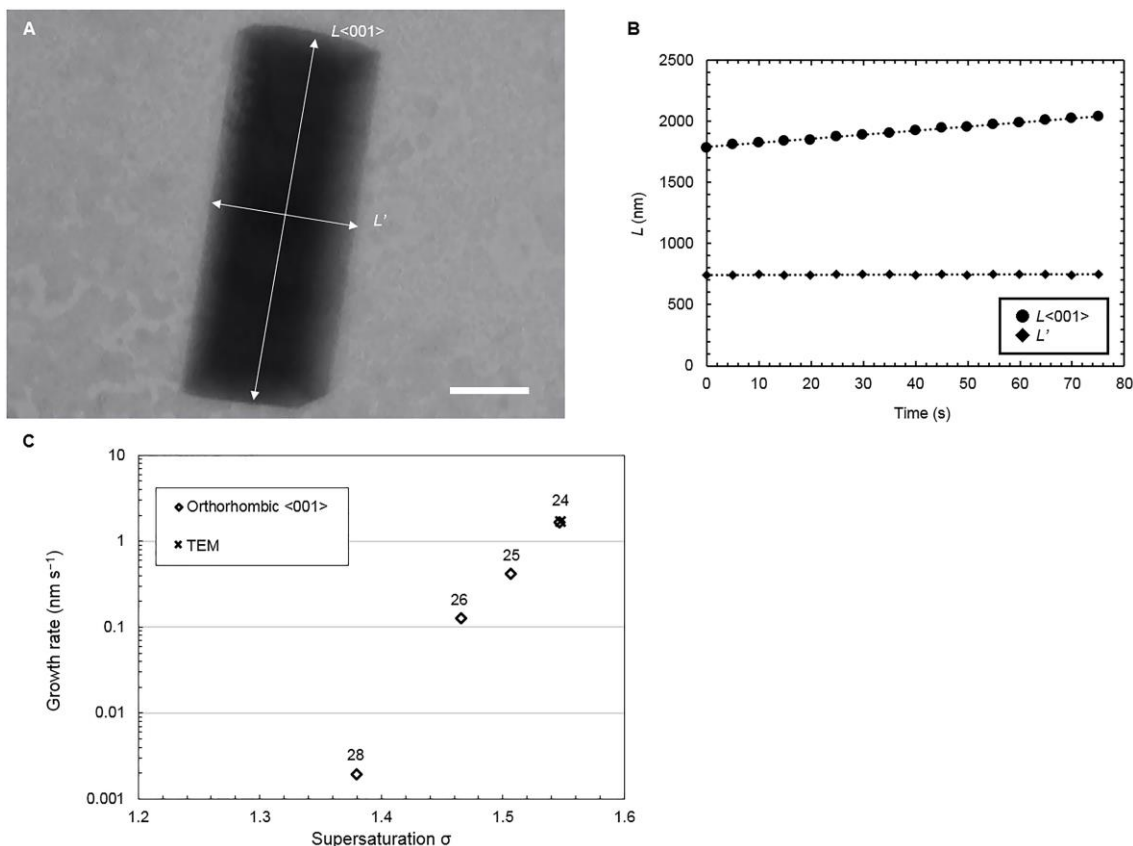
Figure S7. Growth rates of the orthorhombic crystals in the presence of electron irradiation.
