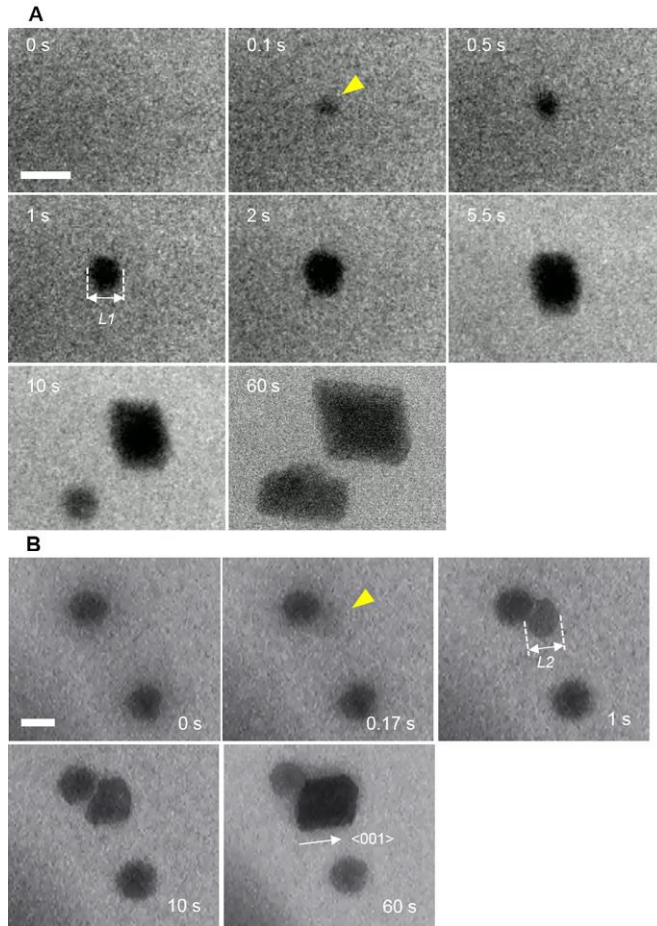
Figure 2. The nucleation of lysozyme crystals monitored by time-resolved in situ TEM.
