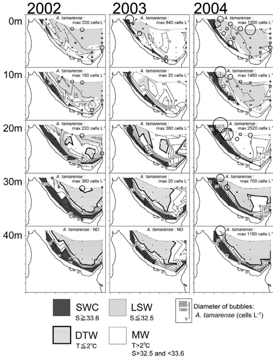
Fig. 25 Spatial distribution of water temperature (contours), water masses (shades) and cell density of Alexandrium tamarense (bubbles) in July 2002–2004 (modified from Shimada et al. 2010). Abbreviations of water masses; SWC: Soya Warm Current (salinity \geq 33.6 ). LSW: Surface low –salinity water (salinity \leq 32.5 ). MW: Mixed water (water temperature > 2^\circ\text{C} , salinity > 32.5 and < 33.6 ). DTW: Dichothermal water (water temperature \leq 2^\circ\text{C} ).
