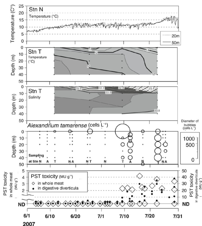
Fig. 42. Temporal changes in water—temperature at Stn N (line), vertical distribution of water temperature and salinity (contours) at Stn T, cell densities of Alexandrium tamarense (bubbles) at each station and PST toxicity of scallop along the coast off Abashiri (two axes scatterplot) during June – July 2007 (modified from Shimada et al. 2012). Toxicity value of “ND” means “not detected (toxicity < 2 \text{ MU g}^{-1} )”
