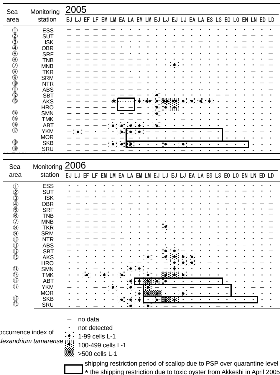
Fig. 17 Diagrams showing occurrences of Alexandrium tamarense (closed circles with shade) and shipment restrictions (rectangular frames) due to detecting PST from scallop (excluding the PST detection from oyster in April 2005) exceeding the quarantine level (4 MU g -1 meat) at the 21 monitoring stations around Hokkaido during 2005–2006 (modified from Shimada et al. 2007).
