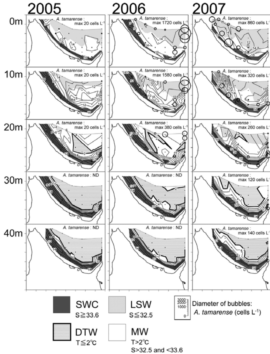
Fig. 26 Spatial distribution of water temperature (contours), water masses (shades) and cell density of Alexandrium tamarense (bubbles) in July 2005–2007 (modified from Shimada et al. 2010). Abbreviations of water masses; SWC: Soya Warm Current (salinity \geq 33.6 ). LSW: Surface low –salinity water (salinity \leq 32.5 ). MW: Mixed water (water temperature > 2^\circ\text{C} , salinity > 32.5 and < 33.6 ). DTW: Dichothermal water (water temperature \leq 2^\circ\text{C} ).
