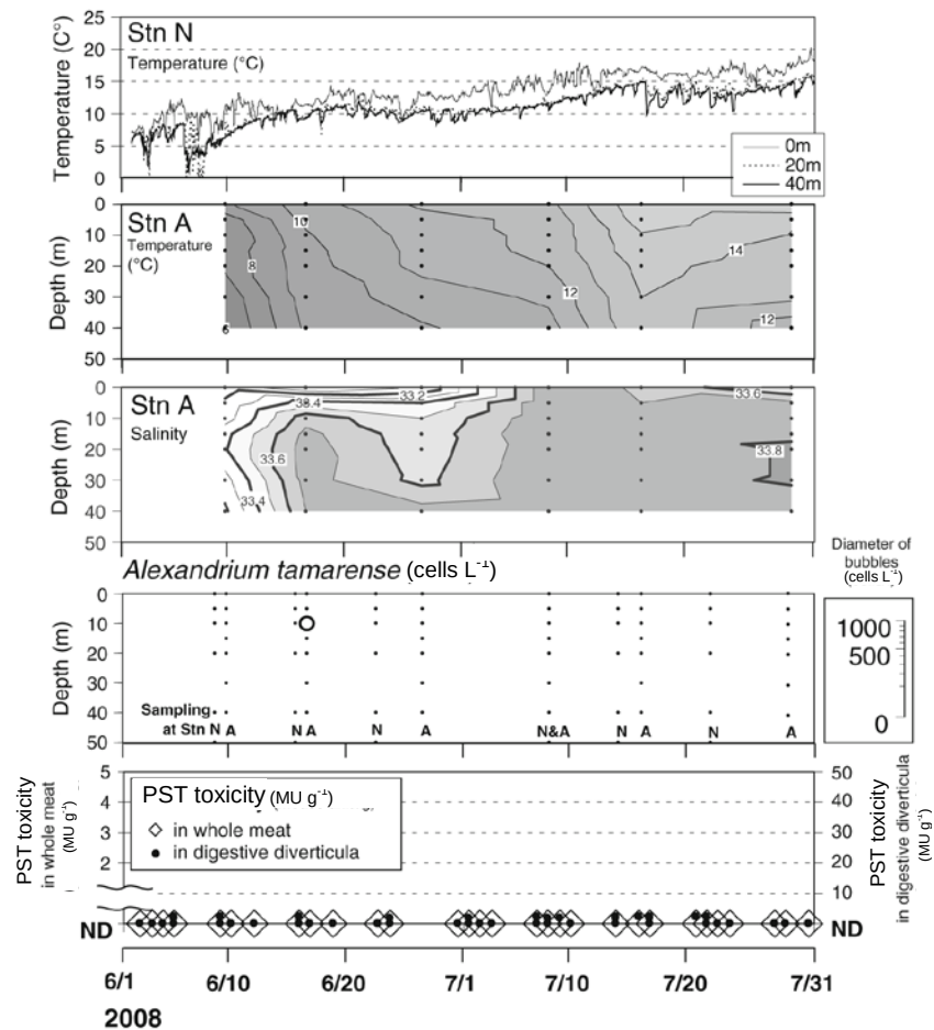
Fig. 43 Temporal changes in water—temperature at Stn N (line), vertical distribution of water temperature and salinity (contours) at Stn A, cell densities of Alexandrium tamarense (bubbles) at each station and PST toxicity of scallop along the coast off Abashiri (two axes scatterplot) during June – July 2008 (modified from Shimada et al. 2012). Toxicity value of “ND” means “not detected (toxicity < 2 MU g -1 )”
