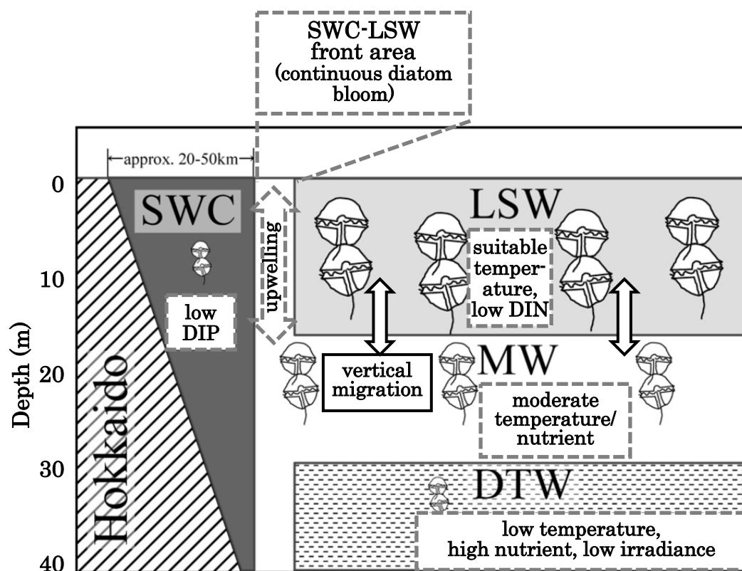
Fig. 31 Schematic diagram of spatial distribution of water masses, front area with upwelling and abundance of Alexandrium tamarense in vertical section in the Okhotsk Sea off Hokkaido. Icon size of A. tamarense indicates relative abundance (modified from Shimada et al. 2010).
