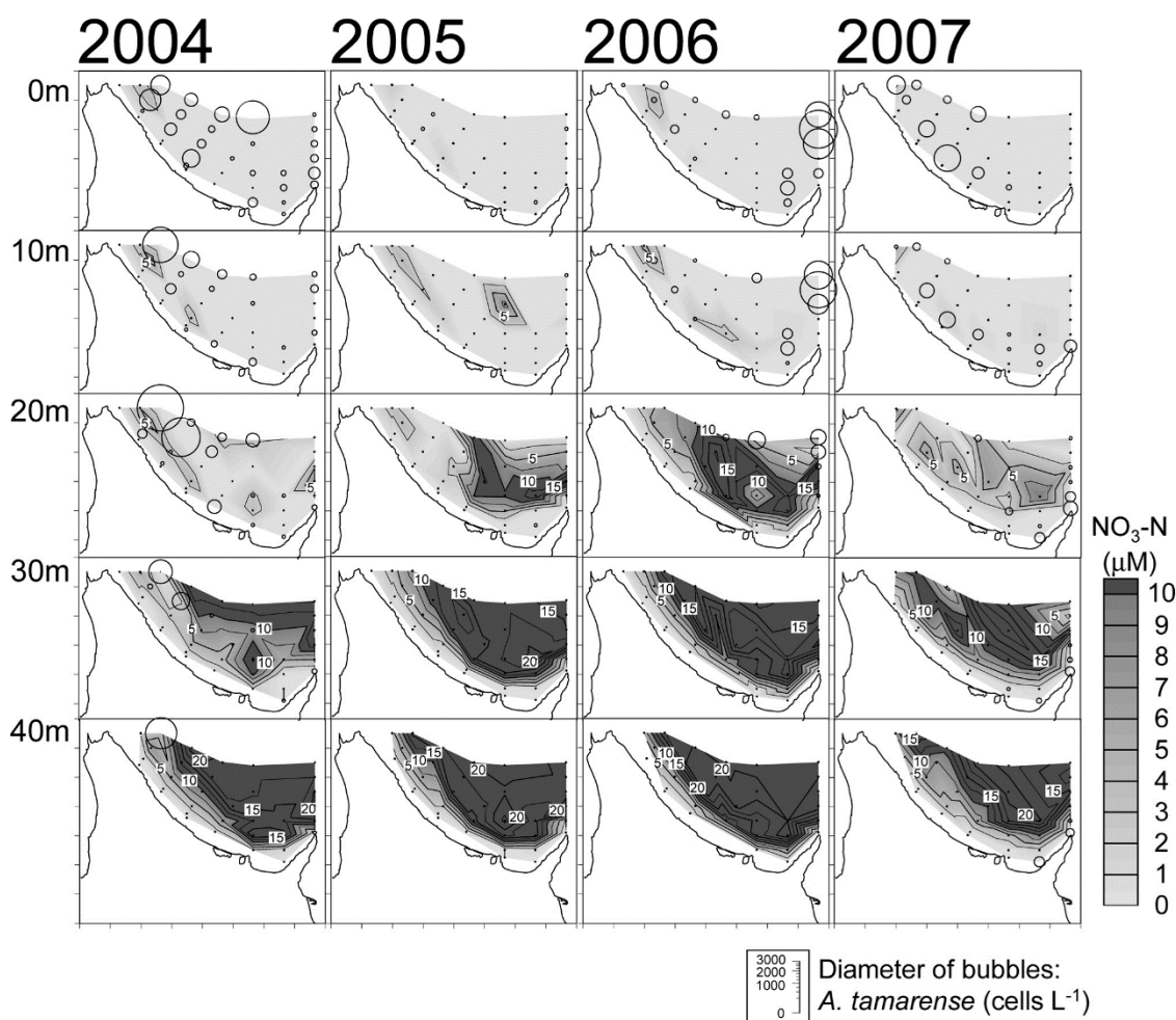
Fig. 28 Spatial and vertical distribution of \text{NO}_3\text{-N} concentration (contours) and cell density of Alexandrium tamarense (bubbles) in July 2004–2007 (modified from Shimada et al. 2010).
