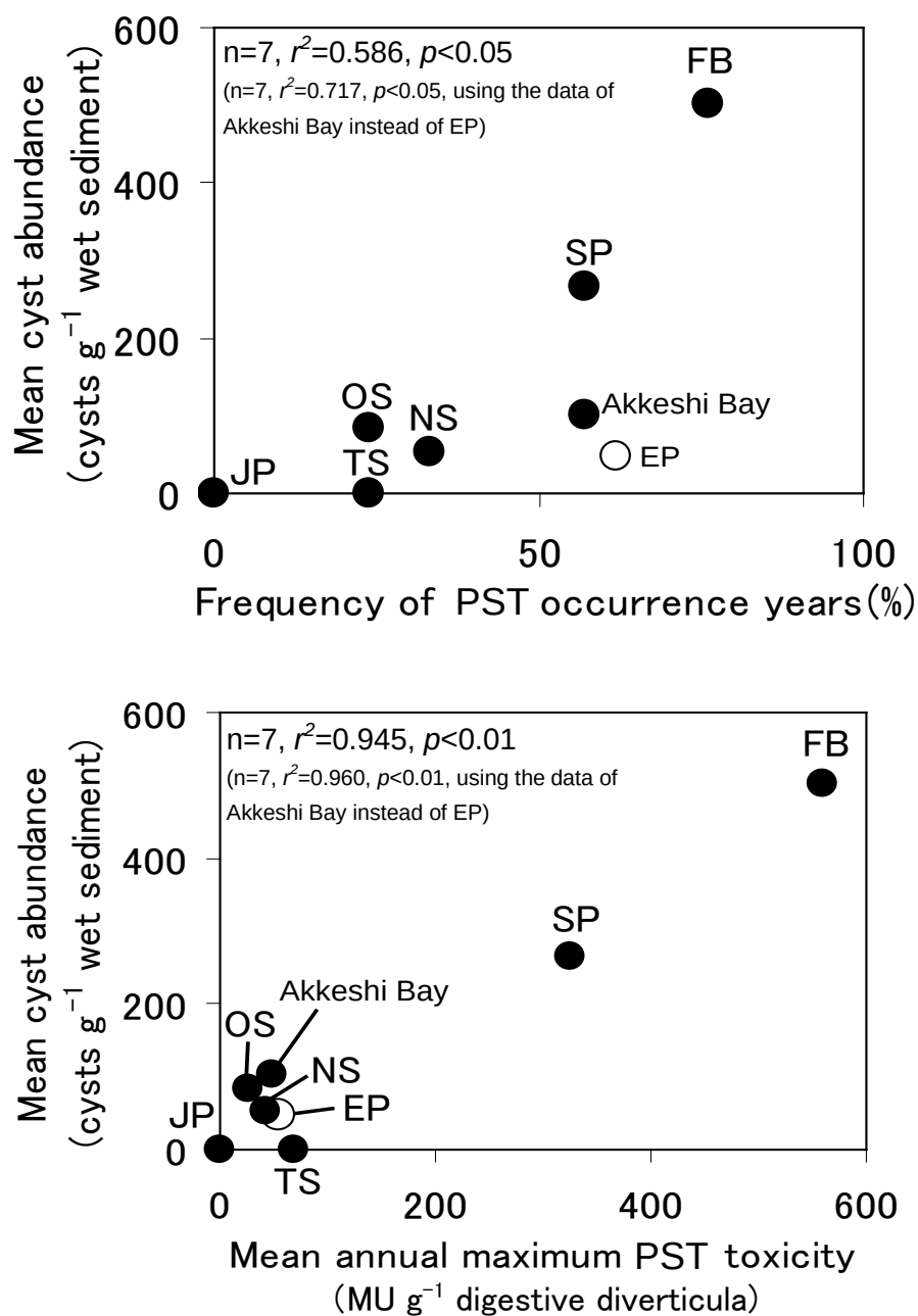
Fig. 23 Relationships among the mean cyst abundance, the frequency of PSP occurrence years (%), above) and the mean annual maximum PST toxicity (MU g -1 digestive diverticula of scallop, below) in 1980–2000 (modified from Shimada and Miyazono 2005).
