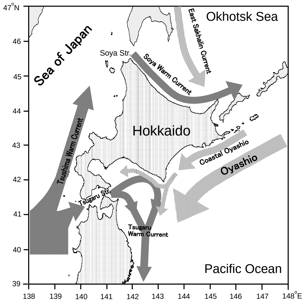
Fig. 5 Schematic paths of the warm currents (Tsushima, Soya and Tsugaru Warm Currents) and the cold currents (East Sakhalin Current, Coastal Oyashio and Oyashio) around Hokkaido (modified from Isoda and Kishi 2003).
