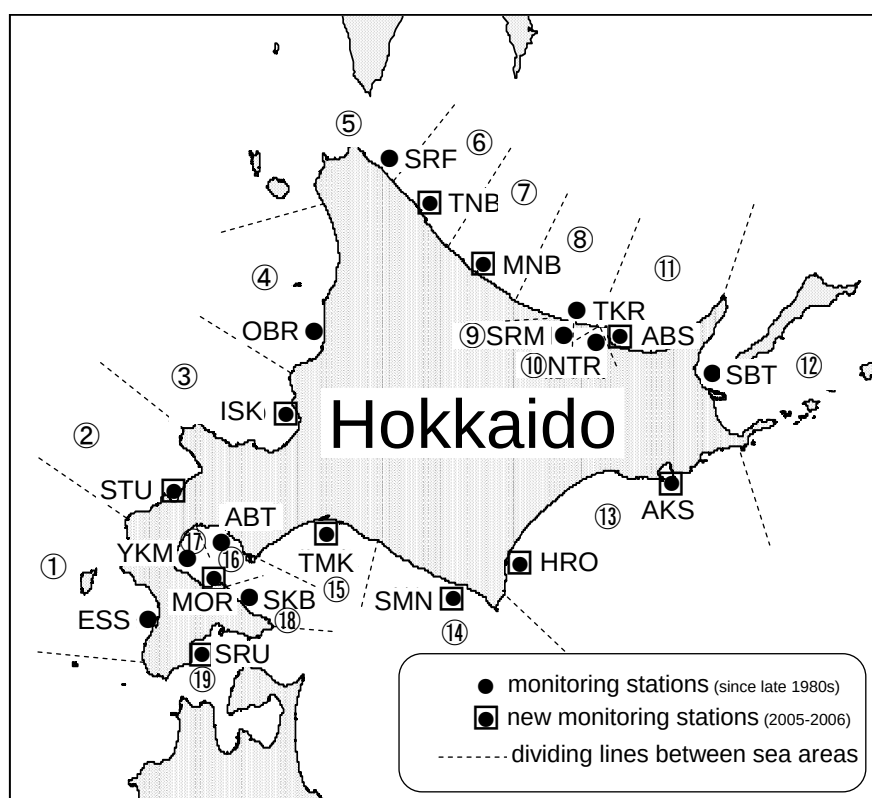
Fig. 14 Map showing location of the 21 stations (closed circles) and 19 sea areas (divided by broken lines) for monitoring of Alexandrium tamarense around Hokkaido during 2005–2006 (modified from Shimada et al. 2007).
