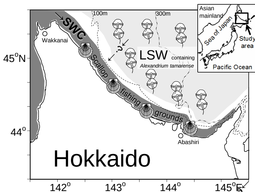
Fig. 8 Schematic path of the Soya Warm Current (SWC, salinity \geq 33.6 ) and location of the scallop fishing grounds and the low salinity water (LSW, salinity \leq 32.5 ) contained Alexandrium tamarense in summer (modified from Shimada et al. 2012). The present study examined the appropriateness of the hypothetical scenario, "PST occurrence is caused by the inflow of LSW to the scallop fishing ground at the temporal weakening of SWC".
