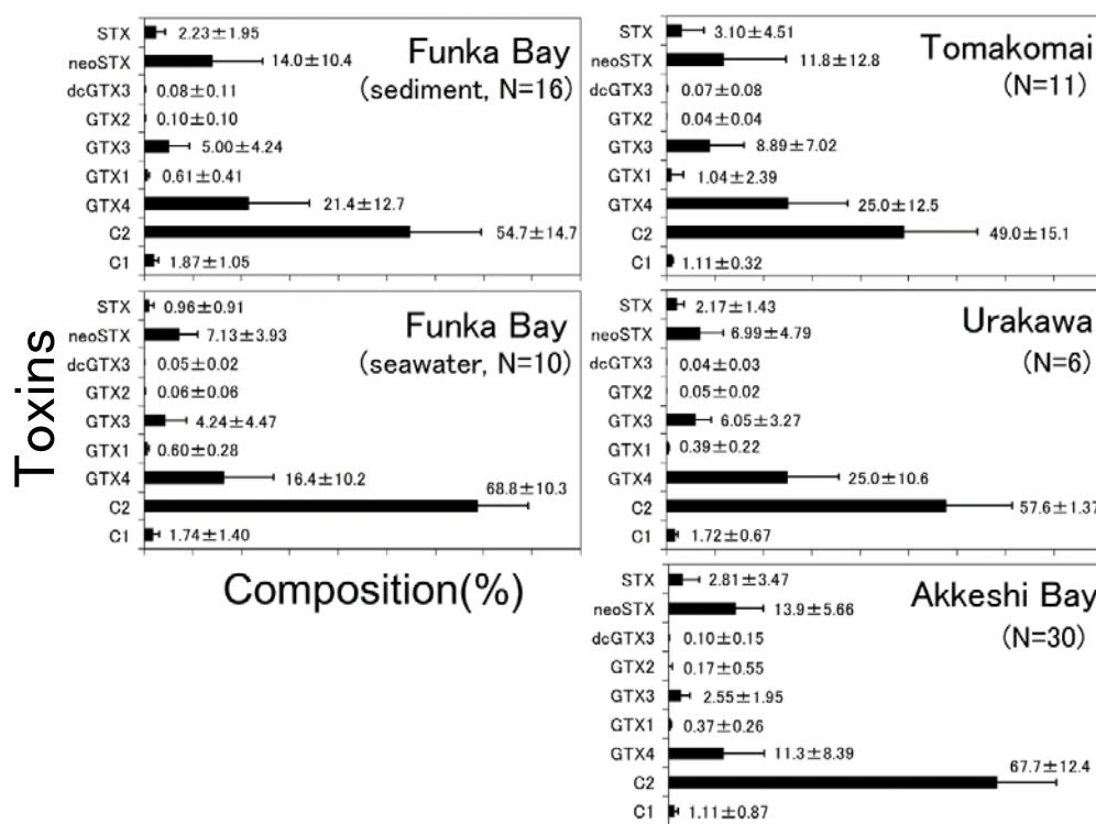
Fig. 34 Average composition of PST (mean ± standard deviation) in the culture strains of Alexandrium tamarense obtained from the four sampling areas (modified from Shimada et al. 2011). Error bars indicate standard deviation, “N” mean number of culture strains. Results of the culture strains obtained from bottom sediment and seawater in Funka Bay are described separately. Abbreviations and specific toxicity of toxin components are shown in Fig. 33.
