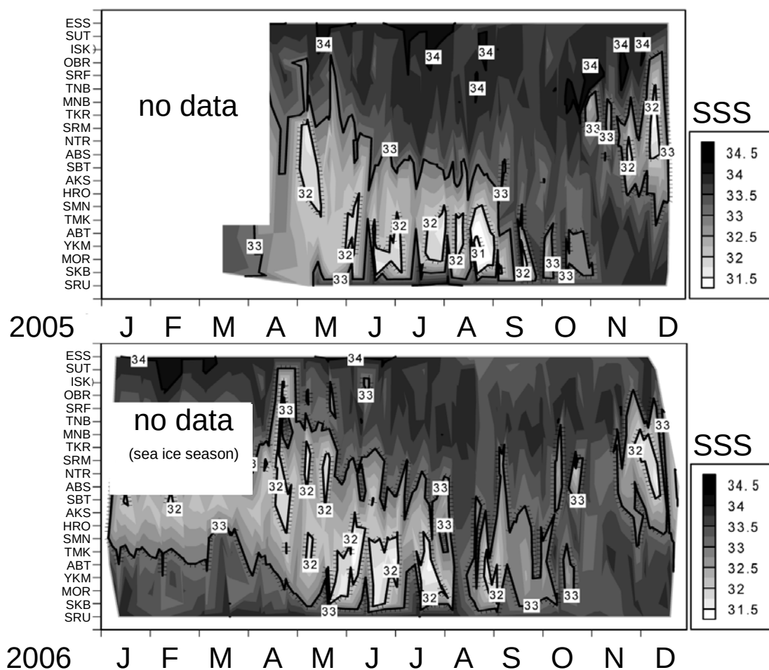
Fig. 16 Isopleths showing seasonal change of sea surface salinity (SSS) at the 21 monitoring stations around Hokkaido during 2005–2006 (modified from Shimada et al 2007). For location of each monitoring station, see Fig. 14.
