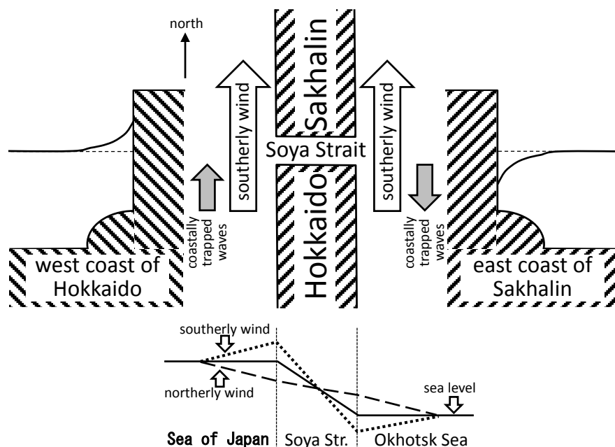
Fig. 51 Diagram showing the generation mechanism of the subinertial variations in the Soya Warm Current by wind – generated coastally trapped waves (modified from Ebuchi et al. (2009)).
