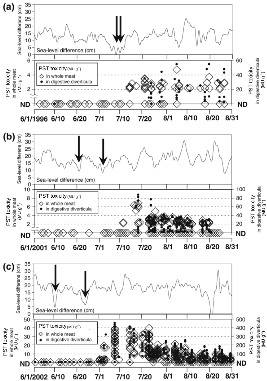
Fig. 47 Temporal changes in of the sea – level difference and PST toxicity during June – August of 1996 (a), 2001 (b) and 2002 (c) (modified from Shimada et al. 2012). The arrows indicate obvious decreases of the sea – level difference. Obvious decrease of the sea – level difference is defined as the minimum and second minimum peaks of the sea – level difference after June before increase of PST toxicity. Toxicity value of “ND” means “not detected (toxicity < 2 MU g -1 )”.
