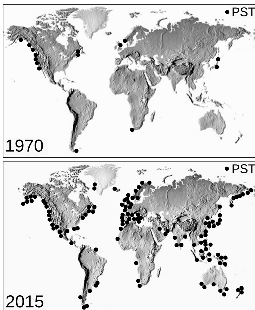
Fig. 1 Global distribution of PST accumulation by shellfish reported in 1970 and 2015 (modified from http://www.who.int/cms/images/PSP_worldmap_1970_2015_422437.jpg , last visited Aug. 24/ 2016).
