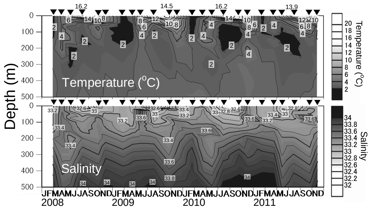
Fig. 10 Seasonal changes in vertical profiles of water temperature (upper) and salinity (lower) at Doto area of the North Pacific (Stn. P15) during 2008–2011 (modified from Shimada et al. 2012).
