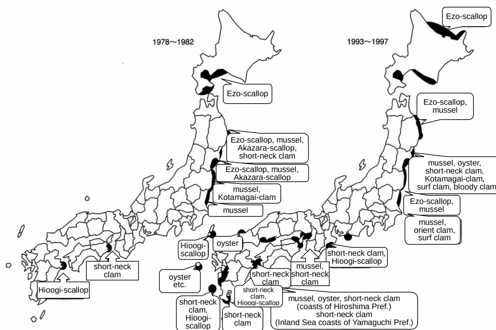
Fig. 2 Occurrence areas of PST accumulation by shellfish in Japan during 1978–1982 (left) and 1993–1997 (right), with the information about shellfish species of PST contamination over the quarantine level ( 4 \text{ MU g}^{-1} meat) (modified from Imai and Itakura 2007).
