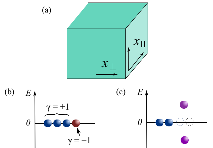
FIG. 1. (a) Schematic image of a semi-infinite nodal superconductor. (b) Fourfold degenerate zero-energy states (ZESs) in the absence of random potential. Three of them belong to the positive chiral eigenvalue (i.e., N_+ = 3 ). One remaining ZES belongs to the negative chiral eigenvalue (i.e., N_- = 1 ). The fourfold degeneracy is protected by translational symmetry. (c) In the presence of random potential, a positive and a negative chiral ZES form a pair and departs from zero energy. However, two positive chiral ZESs remain at zero energy. The index N_{\text{ZES}} = N_+ - N_- = 2 represents the number of ZESs remaining at zero energy in the presence of random potential.
