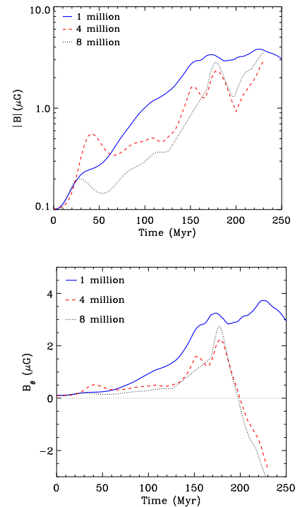
Figure 10. Time evolution of |B| (top) and B_\theta (lower) for simulations at different resolution (MHDN1, our fiducial model, MHDN4 and MHDN8). The evolution is shown for a ring located at a radius of 4 kpc in all the above plots. In all cases, there is much better agreement between the simulations with 4 and 8 million particles compared to the simulation with 1 million particles.
