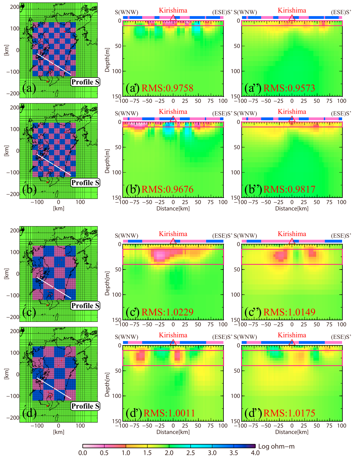
Figure A1. (a–d) Plan views of four checkerboard patterns used in resolution tests in this study, and (a'–d') cross sections along profile S of eight resolution test models obtained by using (a''–d'') the actual measurement configuration provided by the 136 geomagnetic TFs obtained using the configuration of the 72 Network-MT RFs. The four checkerboards (Figures A1a–A1d) were used to obtain the synthetic data, to which 5% Gaussian noise was added before the inversion. Patterns in Figures A1a and A1c are opposite those of Figures A1b and A1d, respectively. The resistivity values of the conductive and resistive blocks in all checkerboard patterns are 3 \Omega\text{m} and 3000 \Omega\text{m} , respectively. All checkerboard patterns have dimensions of 250 \times 200 km in the X and Y directions. The patterns of Figures A1a and A1b and those of Figures A1c and A1d consist of 80 blocks (25 \times 25 km alternately in the horizontal direction) and 20 blocks (50 \times 50 km alternately in the horizontal direction), respectively. The thicknesses of inserted checkerboard patterns are set to 0–10 km (Figures A1a and A1b) and 10–40 km (Figures A1c and A1d) in the vertical direction, which are represented with red boxes on the cross sections. Respective checkerboard patterns along the profile are expressed by bars over the cross sections. The red triangles represent Kirishima volcano.
