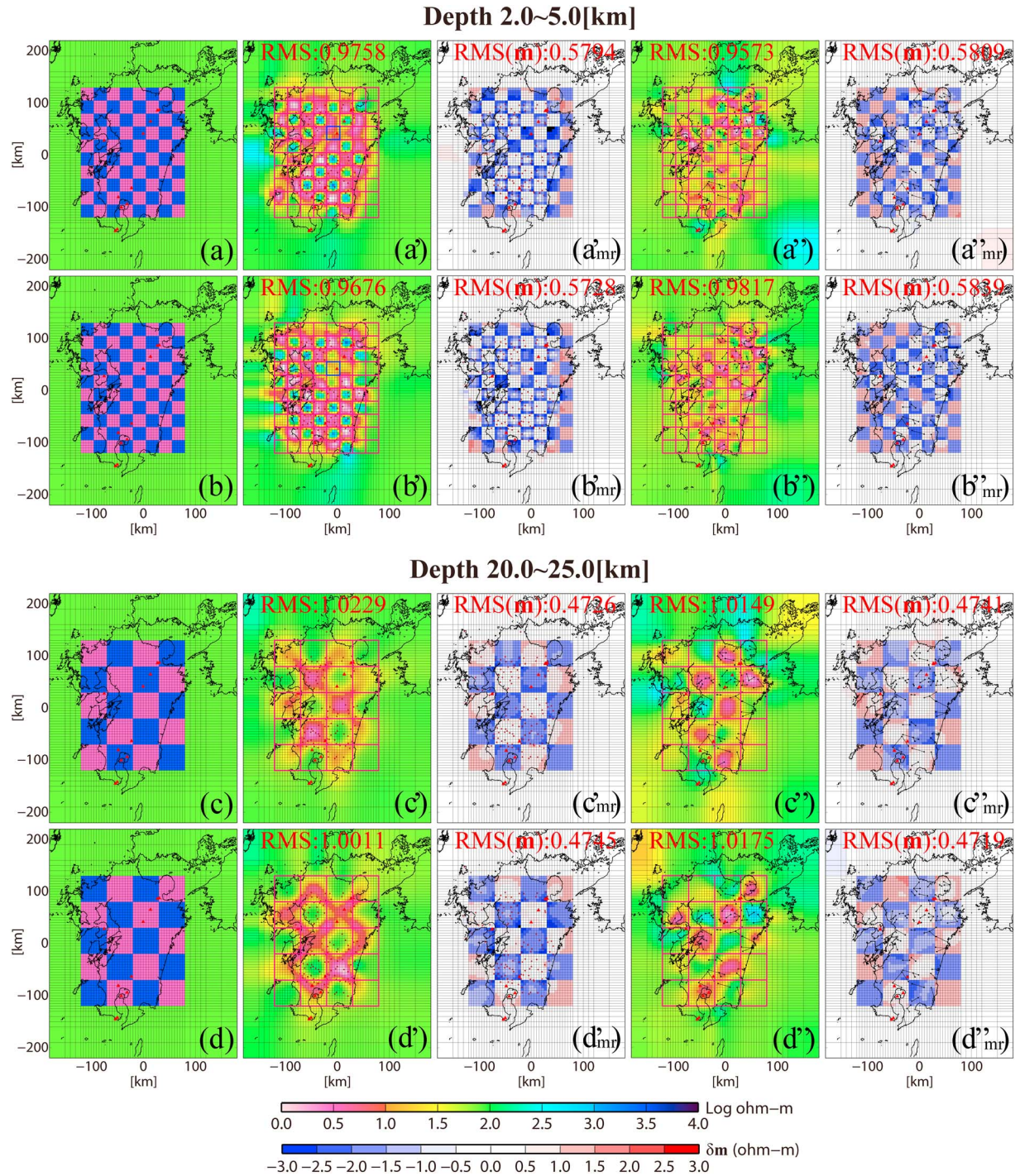
Figure 7. (a–d) Plan views of four checkerboard patterns used in resolution tests in this study, and (a'–d') views of eight resolution test models obtained using (a"–d") the actual measurement configuration provided by the 136 geomagnetic TFs obtained using the configuration of the 72 Network-MT RFs. The other eight plan views (Figures 7a'_mr–7d'_mr and 7a''_mr–7d''_mr) are images of model recovery for the eight resolution test models. The four checkerboards (Figures 7a–7d) were used to obtain the synthetic data to which 5% Gaussian noise was added before the inversion. Patterns in Figures 7a and 7c are opposite those of Figures 7b and 7d, respectively. The resistivity values of the conductive and resistive blocks in all checkerboard patterns are 3 \Omega m and 3000 \Omega m, respectively. All checkerboard patterns have dimensions of 250 \times 200 km in the X and Y directions. The patterns of Figures 7a and 7b and those of Figures 7c and 7d consist of 80 blocks (25 \times 25 km alternately in the horizontal direction) and 20 blocks (50 \times 50 km alternately in the horizontal direction), respectively. The thicknesses of inserted checkerboard patterns are set to 0–10 km (Figures 7a and 7b) and 10–40 km (Figures 7c and 7d) in the vertical direction. Eight plan view sections (Figures 7a'–7d' and 7a''–7d''), of the inverted models show sections 2–5 km in depth (Figures 7a' and 7b' and 7a'' and 7b'') and 20–25 km in depth (Figures 7c' and 7d' and 7c'' and 7d''). Volcanoes (red triangles) are shown in each section, while the 136 geomagnetic observation sites (red dots) are shown in the four sections (Figures 7a'–7d'), and the 72 dipoles (black lines with endpoints) are shown in the other four sections (Figures 7a''–7d'').
