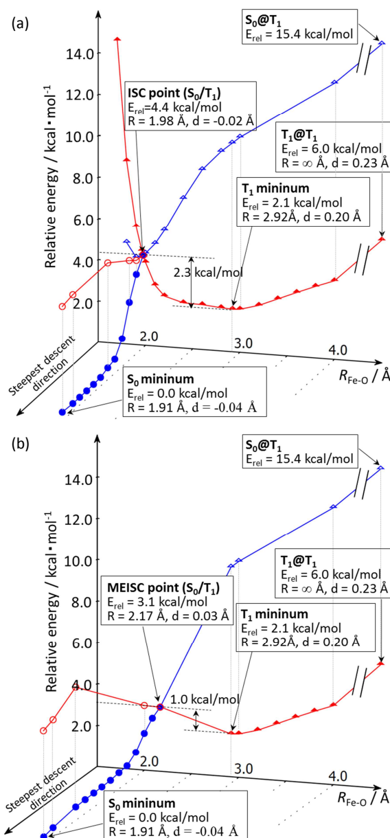
Figure 5. Two dimensional potential energy curves for O_2 binding calculated at the B97D level. (a) Intersystem crossing pathway along the Fe-O fixed coordinate and (b) that via the MEISC. Triangle denotes that the calculations were performed with fixed Fe-O distances. Filled triangles denote that the structure was optimized with this triplet state, while open triangles denote single-point energy. Filled circles denote that the steepest decent reaction pathway on the S_0 surface starting with the ISC point, while open circles denote single-point calculations.
