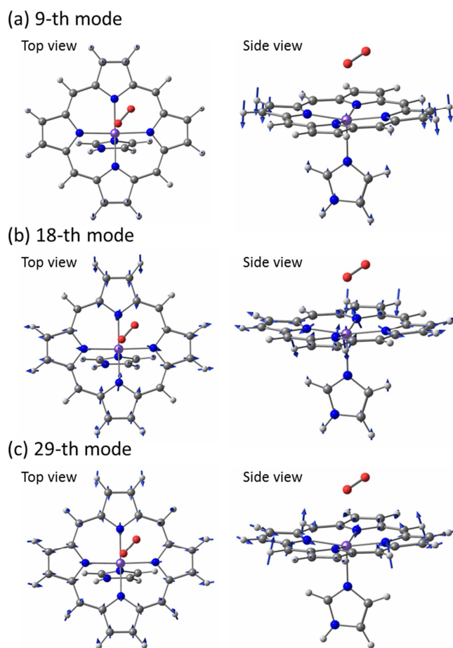
Figure 10 Ninth, eighteenth, and twenty-ninth normal mode at the T_1 minimum.
