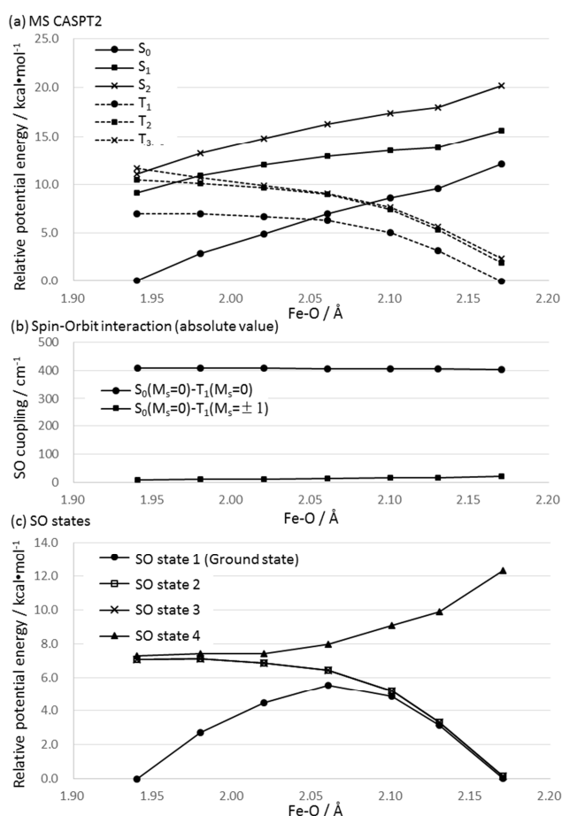
Figure 8 (a) MS-CASPT2 potential energy curves around the MEISCP between the lowest singlet and triplet states. (b) Magnitude of the spin-orbit interaction between the lowest singlet and triplet states around the MEISCP. (c) Eigenstates of the SO Hamiltonian described with the MS-CASPT2 states.
