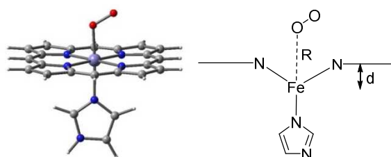
Figure 1 Computational model of oxyheme, the Fe(O 2 )PorIm complex. "R" and "d" denote the Fe-O distance and out-of-displacement of Fe atom. The latter was defined as distance between Fe and the mass-centre of four N atoms.
