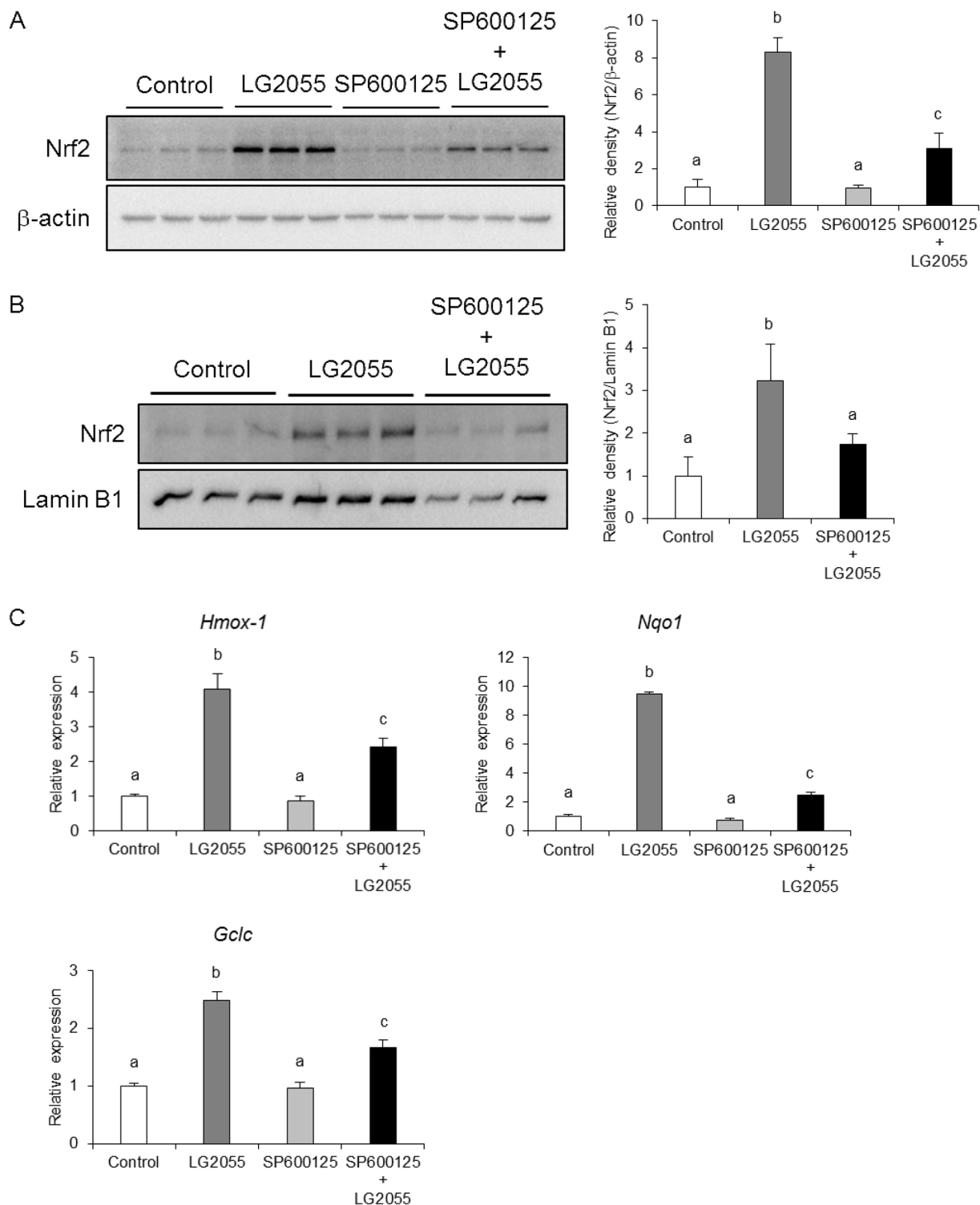
Fig 5. LG2055 activates the Nrf2-ARE signaling pathway by activating the JNK signaling pathway. MEF cells were preincubated with 20 \mu M SP600125 for 1 h and treated with LG2055 for 24 h. (A) The total cell lysates were analyzed by western blotting to compare the Nrf2 protein levels. The relative expression level of Nrf2 normalized by \beta -actin protein expression was quantitated. (B) The cells were fractionated into cytosolic and nuclear fractions using the Focus SubCell kit. The nuclear fraction was analyzed by western blotting to compare Nrf2 protein levels. The relative expression level of Nrf2 normalized by Lamin B1 protein expression was quantitated. (C) The mRNA expression levels of Nrf2 target genes were determined by quantitative real time-PCR analysis. (A-C) Each experiment was performed in triplicate; the data are shown as the means \pm SD. Values not sharing a common letter are significantly different according to one-way ANOVA and Tukey-Kramer post-test analysis; p < 0.05 .
