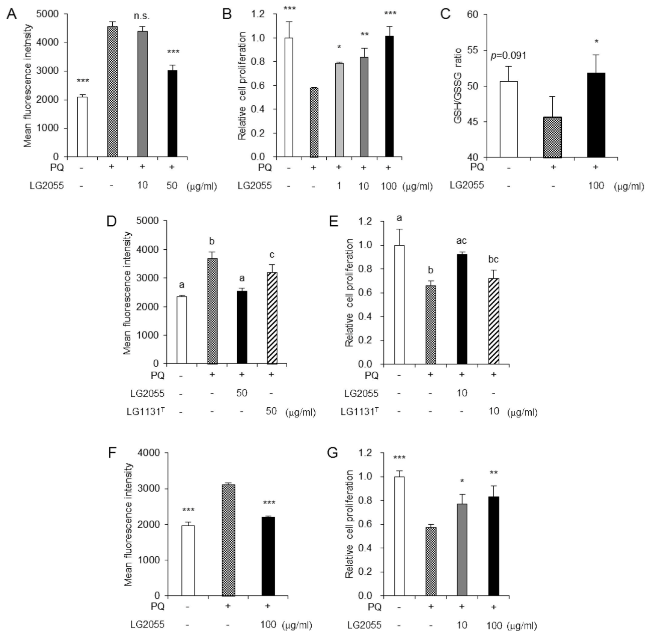
Fig 1. LG2055 strengthens the resistance of murine cells to oxidative stress. (A–E) NIH-3T3 cells were treated with 0.5 mM paraquat (PQ) with or without lactic acid bacteria (LG2055 or LG1131 T ) for 24 h. After incubation, (A, D) the ROS levels were measured as fluorescence intensity by DHE staining, (B, E) the cell proliferation rates were determined using a Cell Counting Kit-8 and (C) the GSH/GSSG ratios were measured by using GSH/GSSG-Glo™ Assay. (F, G) MEF cells were treated with 0.5 mM PQ with or without LG2055 for 24 h. After incubation, (F) the ROS levels were measured and (G) the cell proliferation rates were determined as described in Fig 1A, B. Each experiment was performed in triplicate; the data are shown as the means ± SD. (A, B, C, F, G) * p < 0.05, ** p < 0.01, *** p < 0.001 compared with the control treated with PQ alone using one-way ANOVA and Dunnett's post-test analysis. (D, E) Values not sharing a common letter are significantly different ( p < 0.05) according to one-way ANOVA and Tukey-Kramer post-test analysis.
