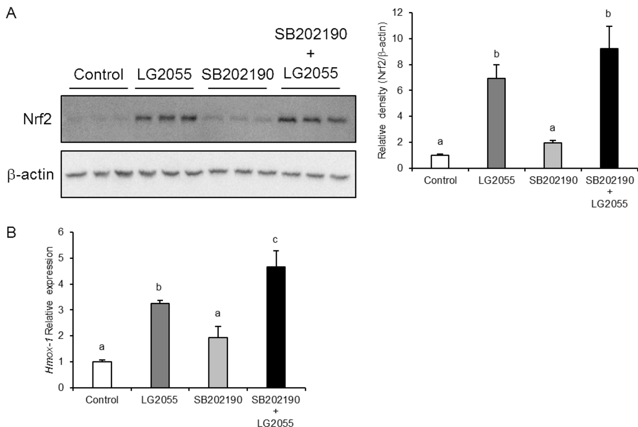
Fig 4. Activation of the Nrf2-ARE signaling pathway induced by LG2055 treatment is not suppressed by inhibition of p38 MAPK. MEF cells were preincubated with 10 \mu M SB202190 for 2 h and treated with LG2055 for 24 h. (A) The total cell lysates were analyzed by western blotting to compare the Nrf2 protein levels. The relative expression level of Nrf2 normalized by \beta -actin protein expression was quantitated. (B) The mRNA expression level of HO-1 was determined by quantitative real time-PCR analysis. (A, B) Each experiment was performed in triplicate; the data are shown as the means \pm SD. Values not sharing a common letter are significantly different according to one-way ANOVA and Tukey-Kramer post-test analysis; p < 0.05 .
