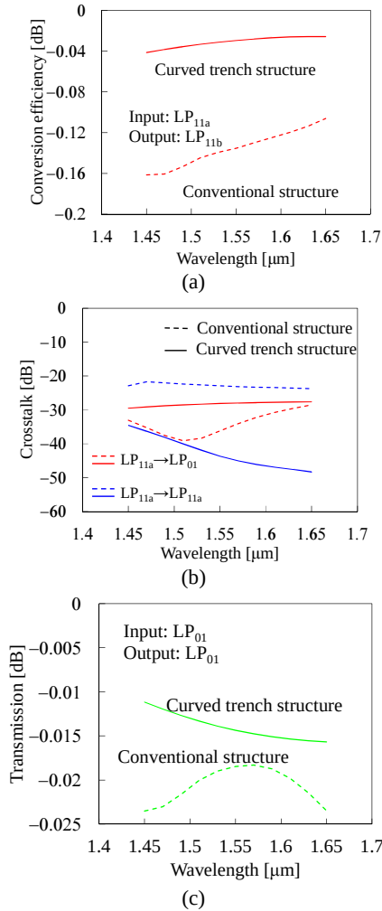
Fig. 9 Transmission spectra of (a) the mode conversion from the LP_{11a} mode to the LP_{11b} mode, (b) the unintentional mode crosstalk, and (c) the transmission from the LP_{01} mode to the LP_{01} mode.
