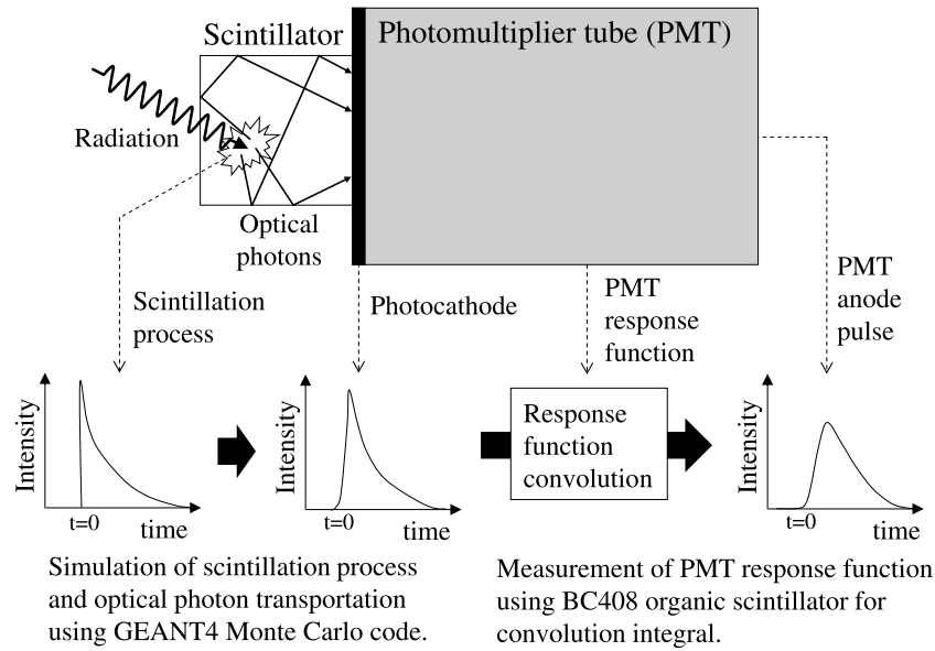
FIG. 1. Schematic diagram of the present pulse emulation method.
