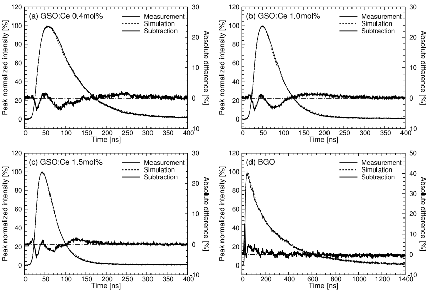
FIG. 8. The measured pulse and the simulated pulse of GSO:Ce (a) 0.4 mol%, (b) 1.0 mol%, (c) 1.5 mol%, (d) BGO scintillators with the estimated decay constant.
