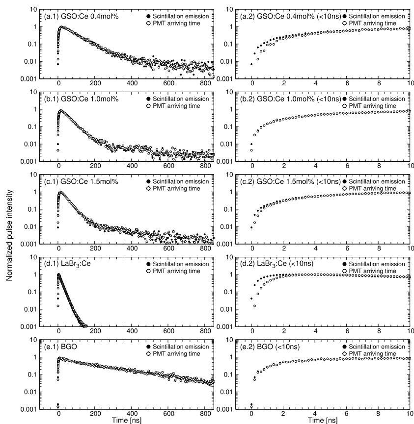
FIG. 3. Emission decay curve and PMT photocathode arriving time simulated by Geant4 Monte Carlo code using GSO:Ce (a.1) 0.4 mol%, (b.1) 1.0 mol%, (c.1) 1.5 mol%, (d.1) LaBr 3 :Ce, and (e.1) BGO scintillators. (a.2)–(e.2) shown an expansion of the rising edge ( <10 ns) in each scintillator.
