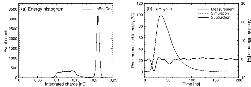
FIG. 6. (a) Energy spectrum using LaBr 3 :Ce scintillator with external radiation source 137 Cs. (b) Difference between the measured and simulated pulses using the present method with a LaBr 3 :Ce scintillator.
