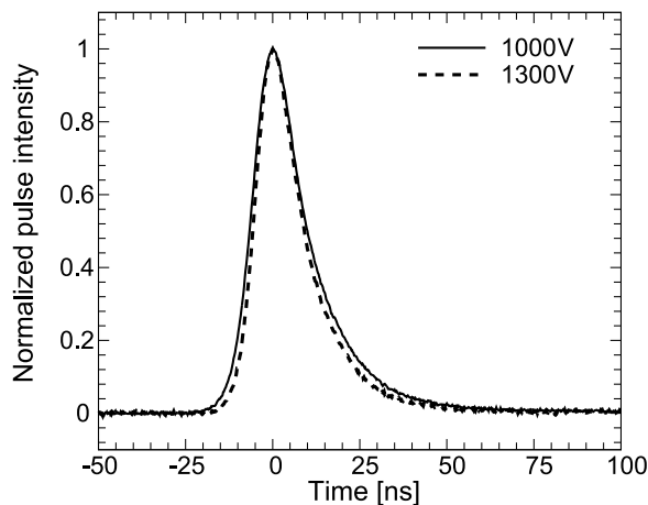
FIG. 4. Response function of the R6231-100 PMT measured by BC408 organic scintillator at supplied voltage of 1300 V and 1000 V.
