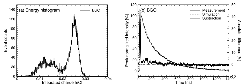
FIG. 7. (a) Energy spectrum using BGO scintillator with 137 Cs external radiation source. (b) Difference between the measured and simulated pulses using the present method with a BGO scintillator.
