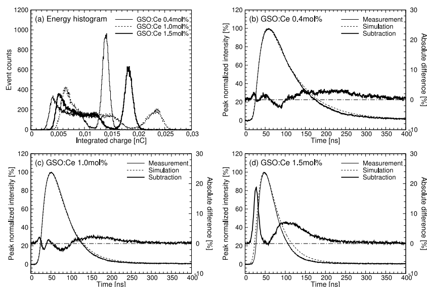
FIG. 5. (a) Energy spectra using GSO:Ce (0.4, 1.0, 1.5 mol%) scintillators with external radiation source 137 Cs. Difference between the measured and simulated pulses using the present method with GSO:Ce scintillators with Ce concentration of (b) 0.4 mol%, (c) 1.0 mol%, (d) 1.5 mol%.
