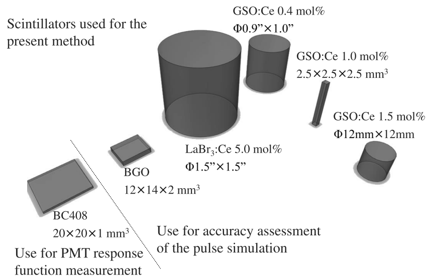
FIG. 2. Structures of GSO:Ce (0.4, 1.0, 1.5 mol%), LaBr 3 :Ce, BGO, and BC408 scintillators.
