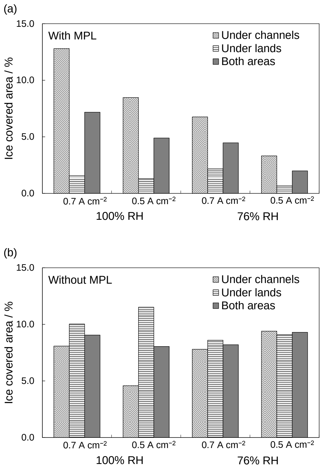
Fig. 10. Average percentages of ice covered areas on the cathode CL surface, calculated using the subtracted images, under the channels, under the lands, and for the total of the areas for cells (a) with and (b) without an MPL.
