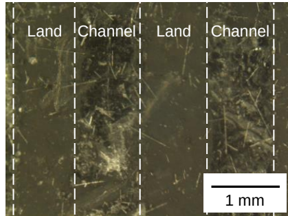
(a) Micrograph
