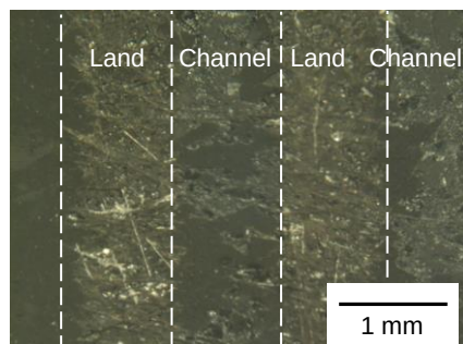
(a) Micrograph
