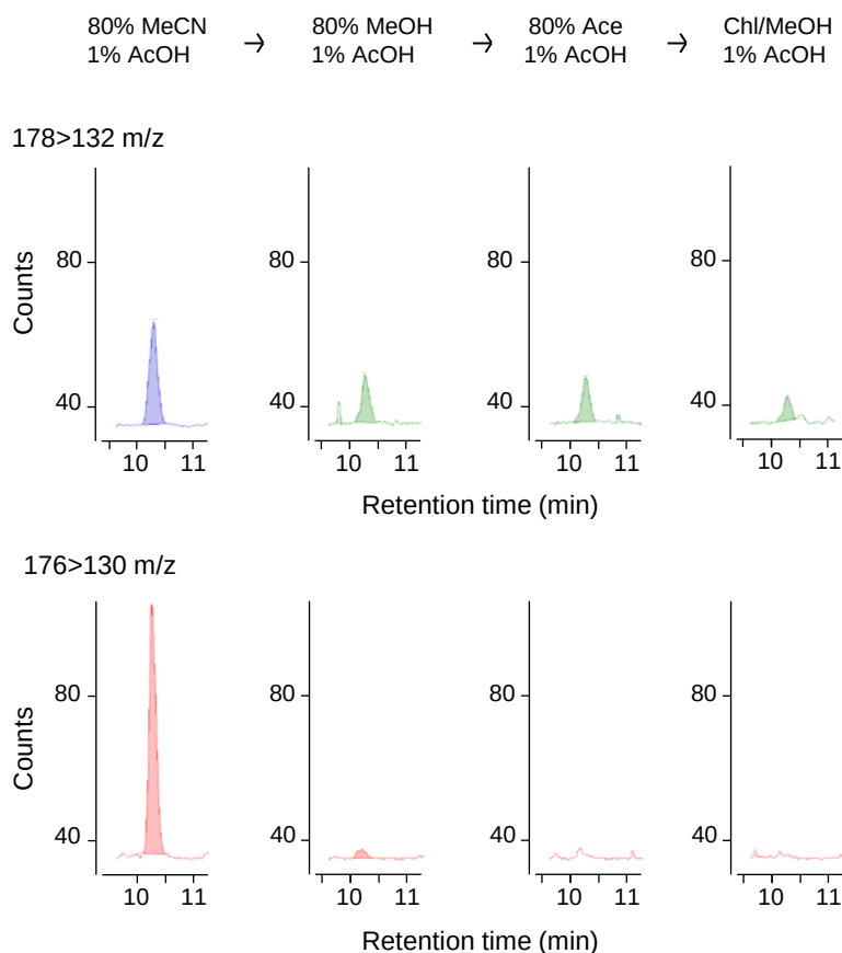
Figure S1. Presence of a cellular substance preventing quantitative analysis of IAA. Sequential stepwise extraction of plant hormones was performed to examine the efficiency of extraction procedure. Ground samples were treated with solvents in the order of 80% acetonitrile containing 1% acetic acid, 80% methanol containing 1% acetic acid, 80% acetone containing 1% acetic acid and chloroform/methanol (1:1) containing 1% acetic acid. Each extract was examined by LC-MS/MS, for which monitoring was done by a MRM chromatogram at 178>132 m/z for IAA (upper) and 176>130 m/z for D 2 -IAA (lower) and. IAA was completely extracted by the second step, whereas an unidentified cellular substance, which has an MRM transition overlapping that of D 2 -IAA, appeared in all extraction steps.
