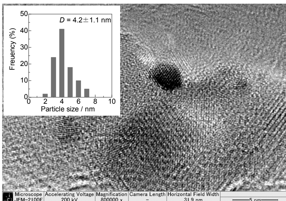
Fig. 4. A representative TEM image and Re metal particle size distribution of Re/Al 2 O 3 (reduced at 500 °C). The mean diameter (nm) of Re particle was 4.2 \pm 1.1 nm, corresponding to the volume-area mean diameter of 5.2 \pm 1.1 nm.
