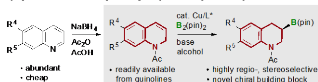
Scheme 1. Dearomatization/enantioselective borylation stepwise strategy for the synthesis of chiral N -heterocyclic organoboron compounds.
