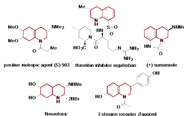
Figure 1. Representative bioactive tetrahydroquinolines.
