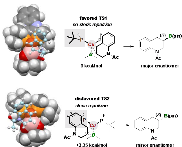
Figure 2. DFT calculations (B3PW91/cc-pVDZ) of the transition states for the ( R,R )-QuinoxP*/copper(I)-catalyzed enantioselective borylation of 1,2-dihydroquinoline 2a . Relative G values (kcal/mol) were obtained at 263 K and 1.0 atm in the gas phase.
