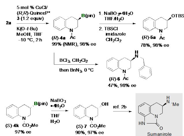
Scheme 2. Synthesis of functionalized chiral tetrahydroquinolines through the derivatizations of the borylation products.
