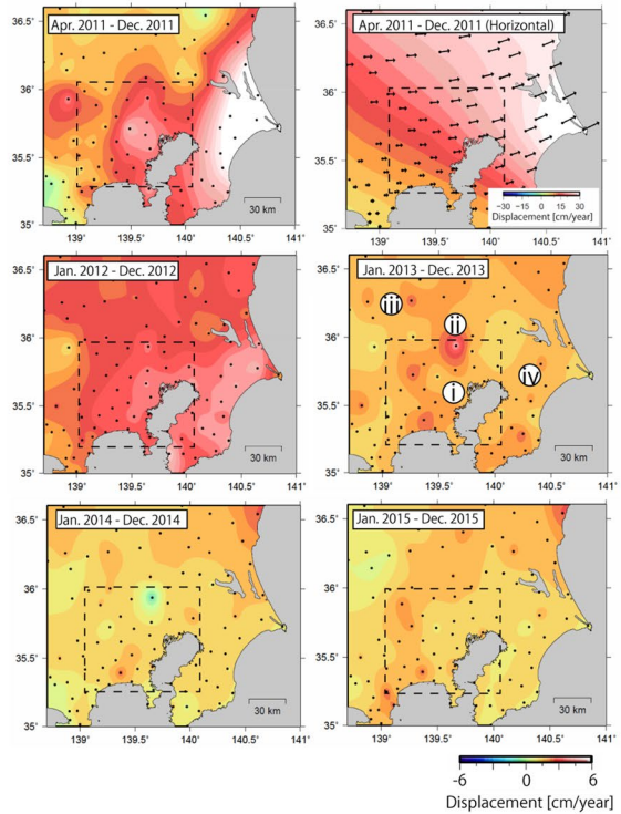
b2 Displacements at the center – south of the Kanto plain (2011–2015)
