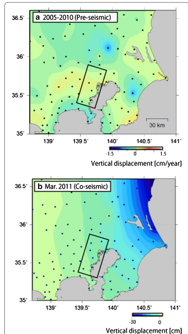
Fig. 2 a Annual vertical surface displacement velocity from January 2005 to December 2010 (the period before the 2011 Tohoku earthquake), derived from the GPS network. b Vertical surface displacement from March 10, 2011, to March 12, 2011 (co-seismic period), derived from the GPS network. Black rectangles are the covered areas of TerraSAR-X images
