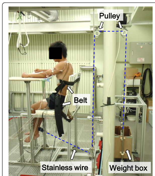
Fig. 1 Scheme of the knee extension device
