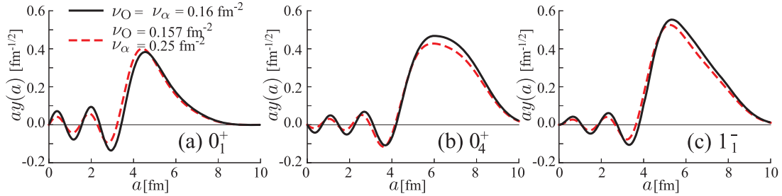
Fig. 2. The ^{16}\text{O} + \alpha cluster RWAs of (a) the 0_1^+ state, (b) the 0_4^+ state, and (c) the 1_1^- state. The solid lines show the RWAs obtained by using the reference states with common oscillator lengths \nu_O = \nu_\alpha = 0.16 \text{ fm}^{-2} , while the dashed lines show those obtained by using the different oscillator parameters \nu_O = 0.157 \text{ fm}^{-2} and \nu_\alpha = 0.25 \text{ fm}^{-2} .
