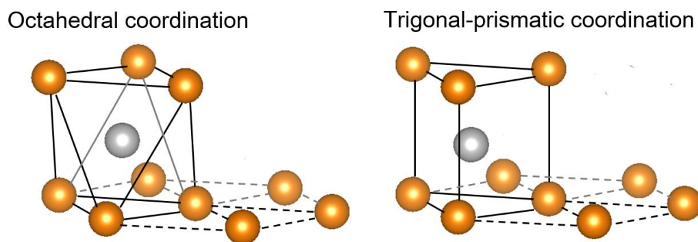
Figure 1 Scheme of octahedral and trigonal coordination.
