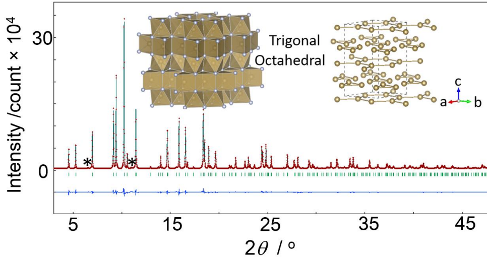
Figure 6 Crystal structure and Rietveld refinement profile of \text{Ta}_{5-x}(\text{O,N})_6 ( x \approx 0.18 ). The structure shows a Ta–(O,N) trigonal-prismatic layer and octahedral layer with ordered vacancies. The small spheres represent oxygen/nitrogen atoms. Synchrotron XRD was measured at a wavelength of 0.41365 Å. The tick marks and line below the pattern represent the positions of the allowed reflections for \text{Ta}_{5-x}(\text{O,N})_6 and difference between the observed and calculated profiles, respectively. The asterisk indicates an impurity phase(s).
