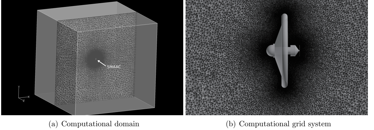
Figure 6: Computational domain and grid system for SMAAC at altitude of 10 km (FFR).
