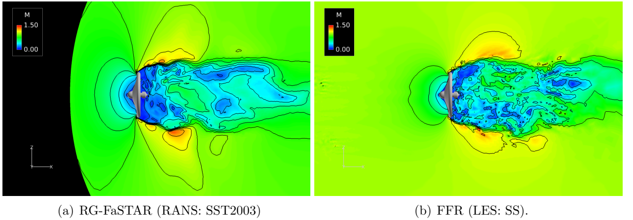
Figure 12: Mach number distribution around SMAAC in the transonic region at an altitude of 39 km ( Re = 1.03 \times 10^5 and M = 0.871 ).
