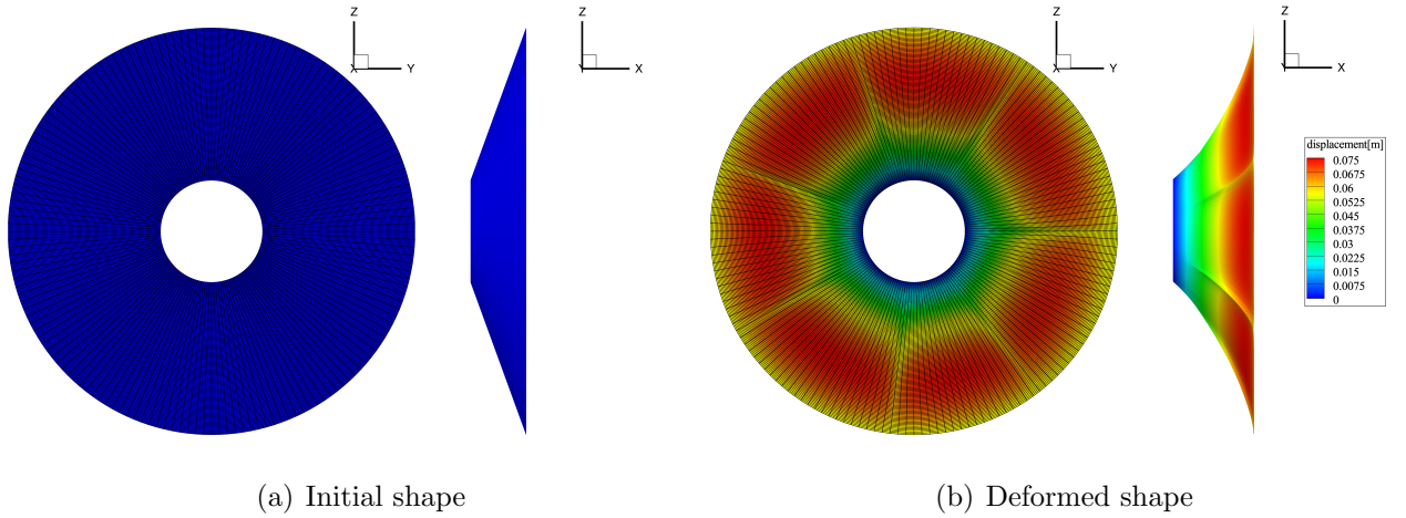
Figure 18: Example of membrane deformation of SMAAC by the aerodynamic force.
