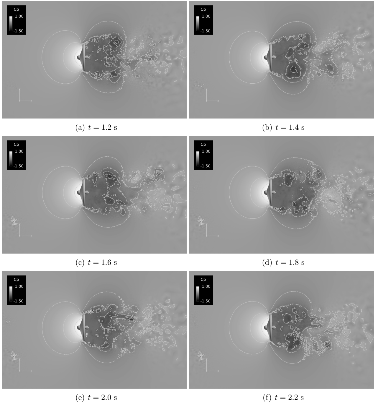
Figure 16: Time series of the instantaneous pressure coefficient around SMAAC at an altitude of 3 km ( \text{Re} = 1.08 \times 10^6 and M = 0.0543 ).
