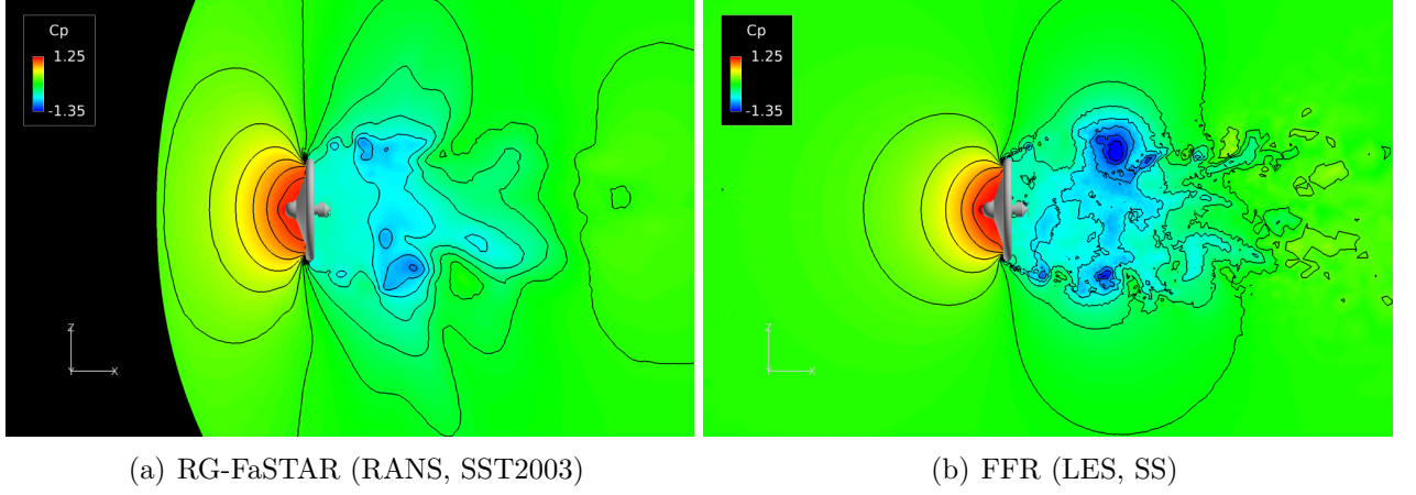
Figure 11: Pressure coefficient distribution around SMAAC in the transonic region at an altitude of 39 km ( Re = 1.03 \times 10^5 and M = 0.871 ).
