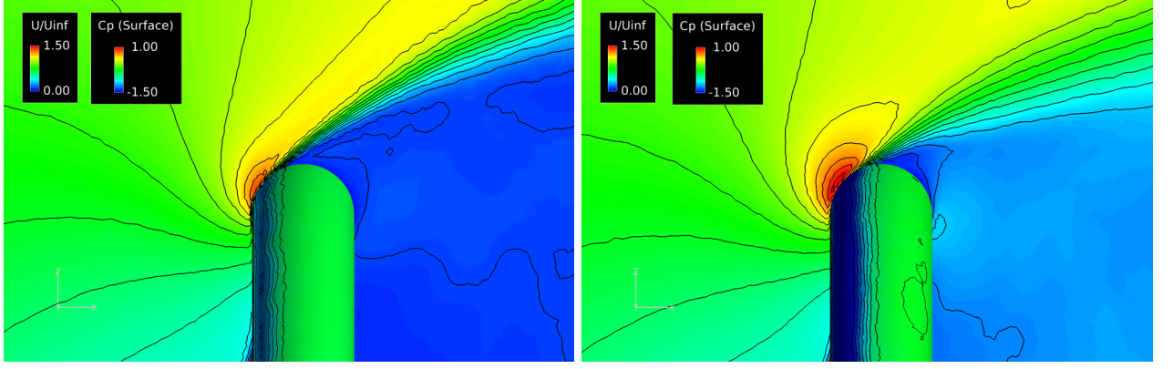
(a) Altitude of 30 km ( Re = 1.87 \times 10^5 and M = 0.402 )(b) Altitude of 10 km ( Re = 8.18 \times 10^5 and M = 0.0820 )
