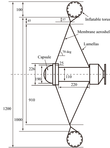
Figure 1: SMAAC configuration. (All dimensions are in millimeters.)
