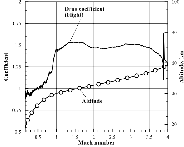
Figure 3: Drag coefficient profile obtained in the flight experiment versus Mach number.
