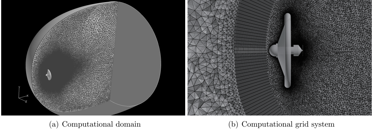
Figure 5: Computational domain and grid system for SMAAC at altitude of 54 km (RG-FaSTAR).
