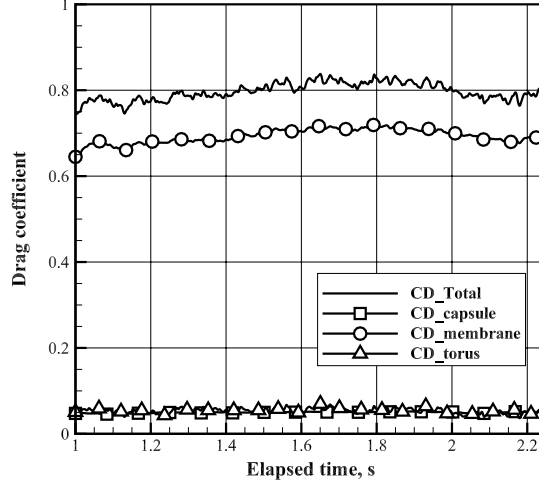
Figure 17: Time history of the drag coefficients at an altitude of 3 km ( Re = 1.08 \times 10^6 and M = 0.0543 ).
