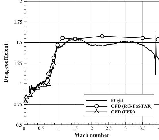
Figure 8: Comparison of drag coefficient between flight data and CFD results.
