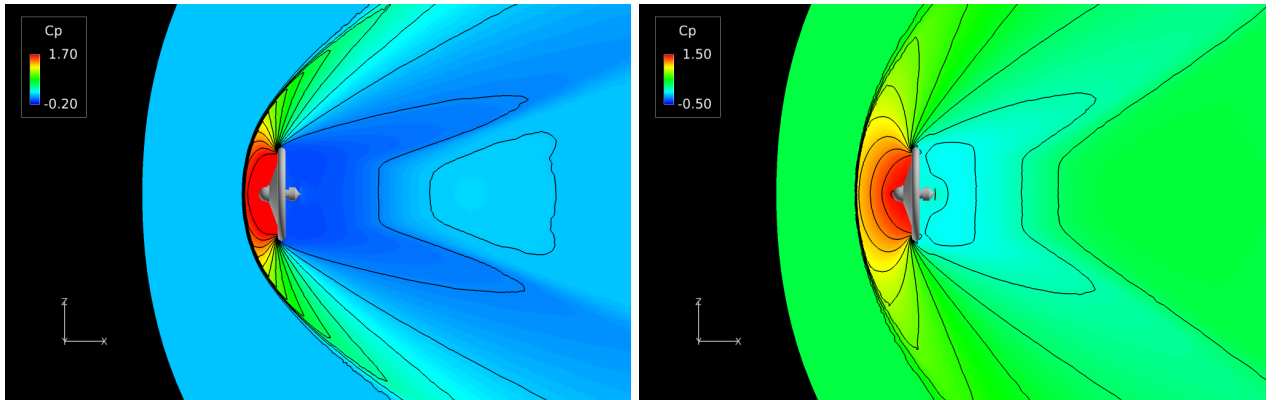
(a) Altitude of 47 km ( Re = 9.01 \times 10^4 and M = 2.30 )(b) Altitude of 43 km ( Re = 1.00 \times 10^5 and M = 1.51 ).
