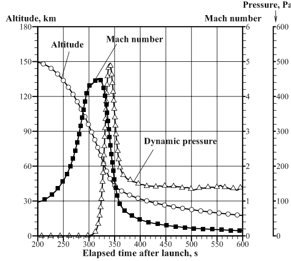
Figure 2: Trajectory profile of SMAAC.
