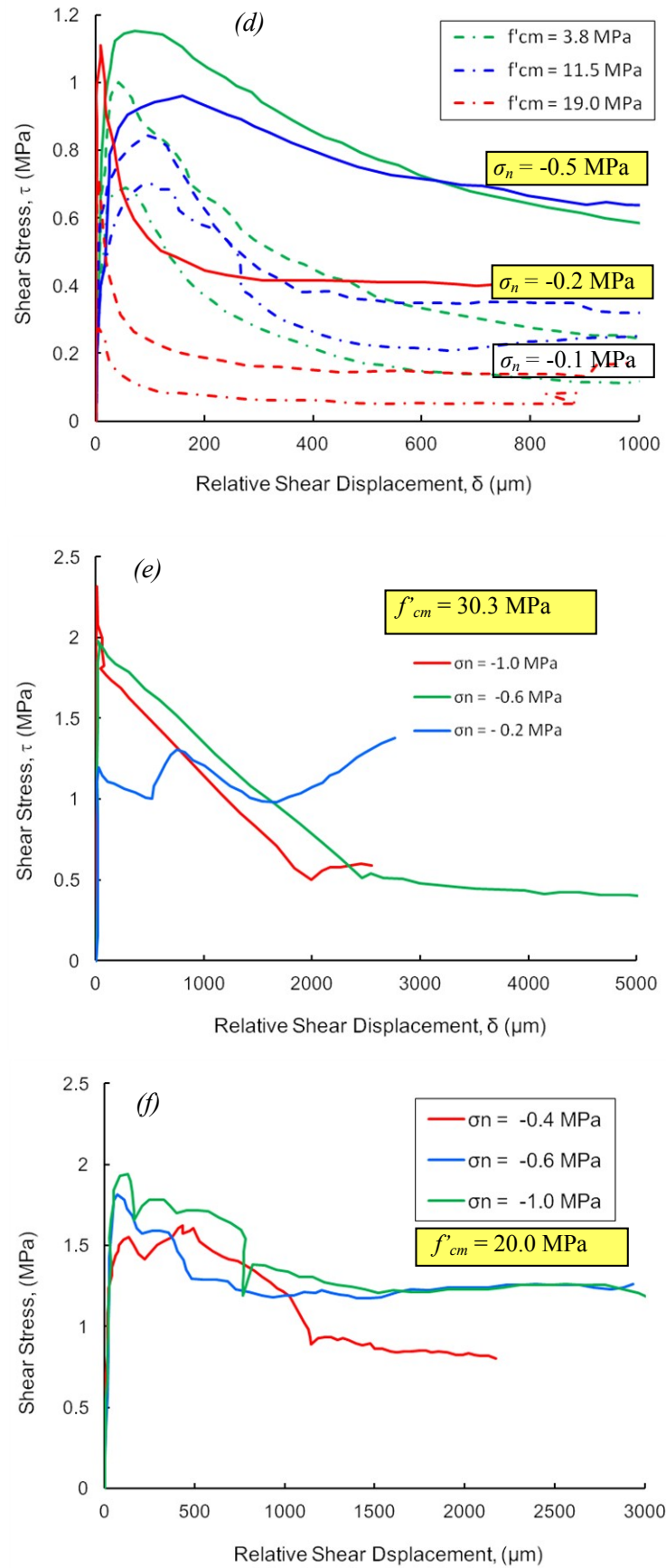
Fig. 3.2. Shear-slip relationship from different experimental results (d) Hansen (1999); (e) Lourenco et al. (2004); (f) Abdou et al. (2006) for perforated clay bricks
