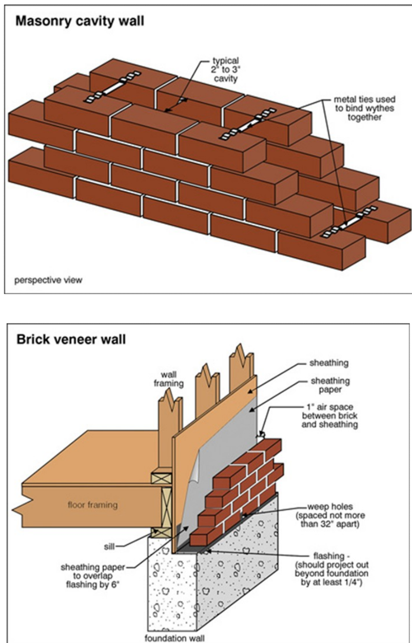
Fig.2.5. Construction process of masonry cavity wall and veneer wall (Carson Dunlop 2014)
