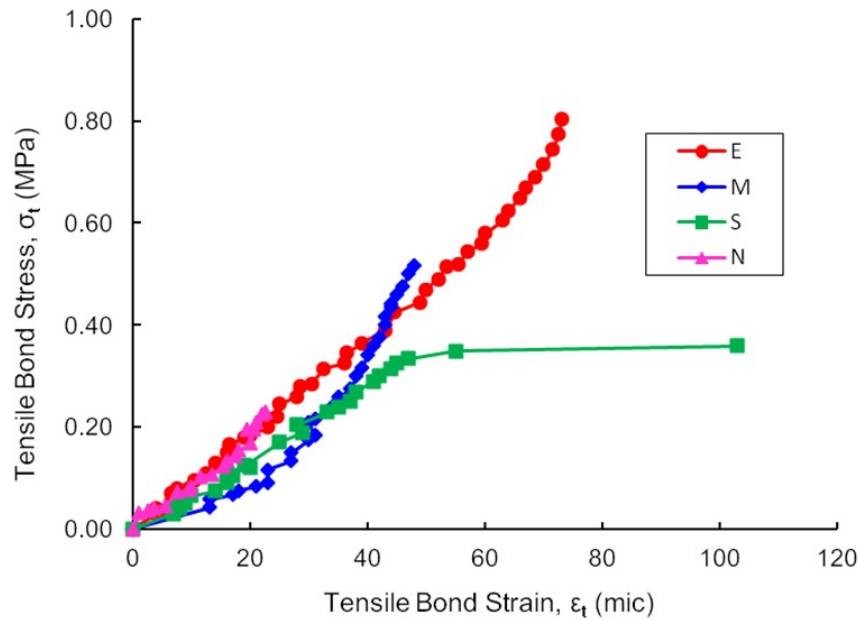
Fig. 3.16. Tensile stress-strain relationship of brick-mortar interface from cross-bond test specimens
