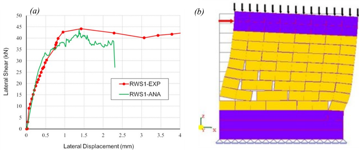
Fig. 4.13. a) Comparison between experimental and numerical results of load-displacement response of URM wall; b) Simulated fracture pattern in the wall
