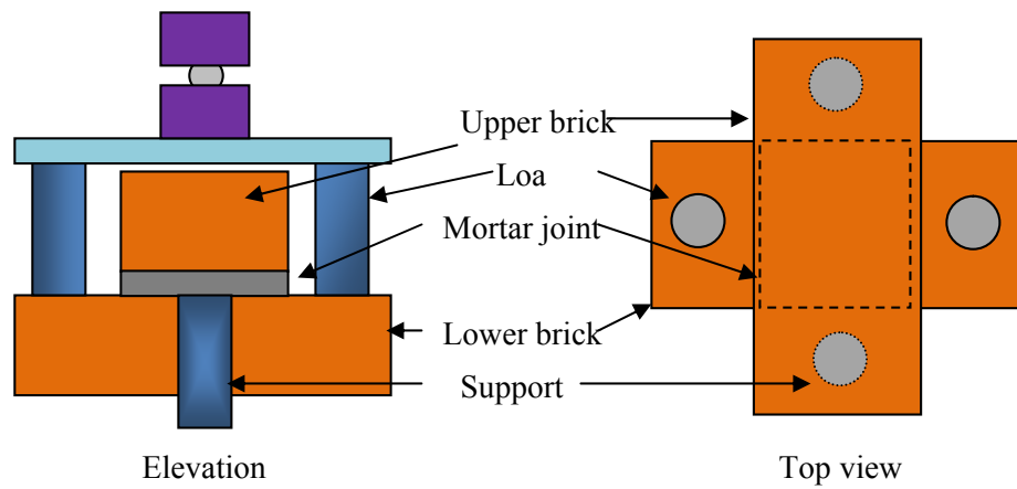
Fig. 3.13. Crossed-brick test assembly (ASTM C 952)
