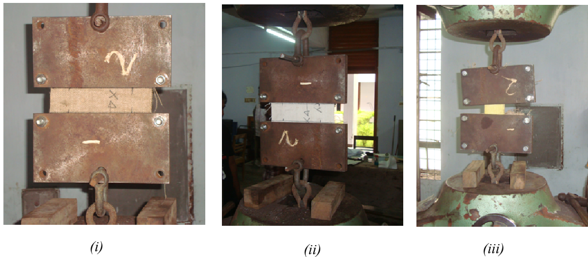
Fig. 5.8b. Uniaxial tension test of fiber sheet, (i) Jute, (ii) Cotton and (iii) Nylon
