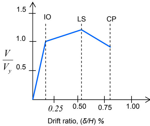
Fig. 5.26. Performance indices
