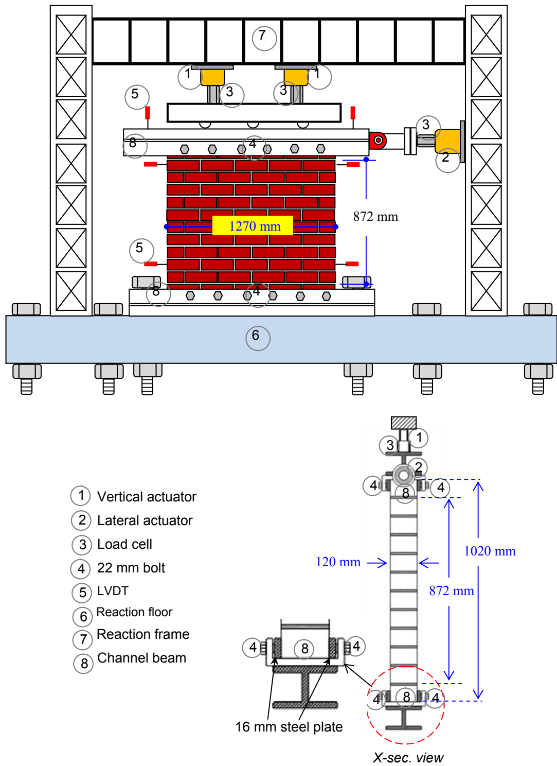
Fig. 5.11. Schematic diagram of experimental setup of shear wall
