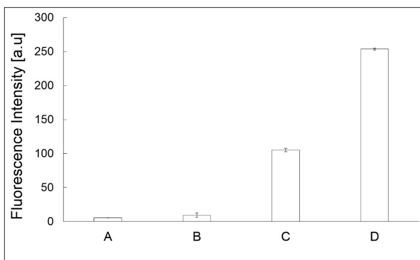
Figure 3. 3 Immobilization of capture antibody. Description of X axis results: A is the demonstration of intensity using bare chromatography paper, B is the demonstration using non-coated paper with chitosan, C is the demonstration using chitosan-coated paper, D is the demonstration using chitosan-coated paper and glutaraldehyde activation. Fluorescein-labeled antibody was introduced to the sample zones at the end of each demonstration and washed out using 200 \mu L of 1% tween 20/PBS.
