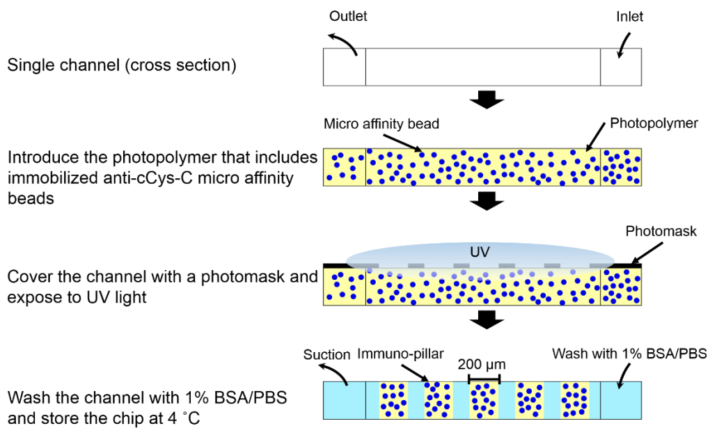
Figure 4. 1 Illustration of fabrication of immuno-pillars
