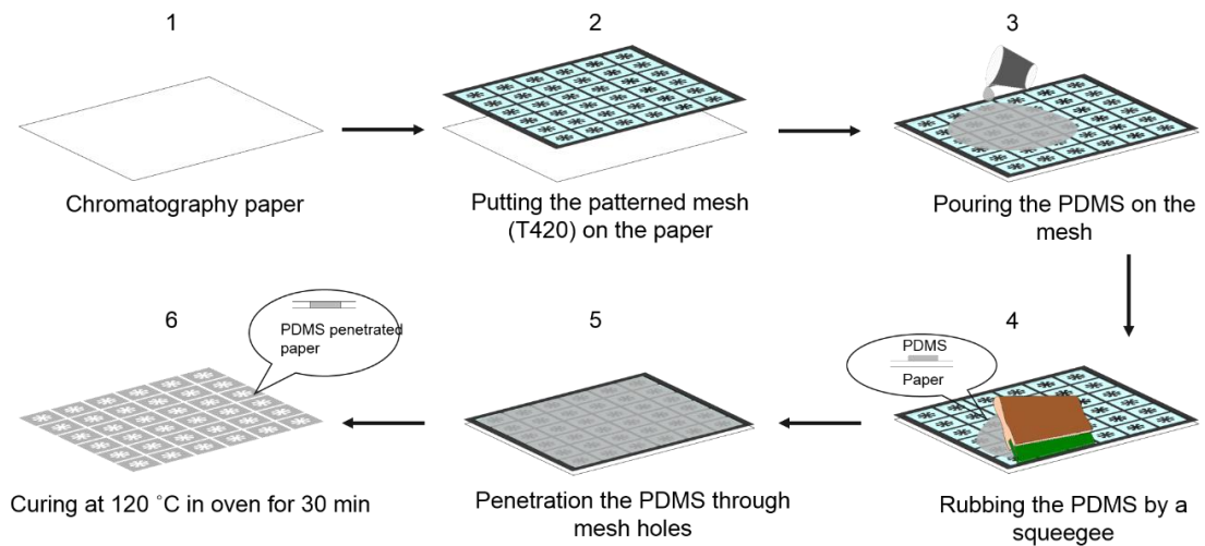
Figure 2.1 Schematic representation of PDMS-screen-printing for fabrication of the \mu PADs. (1), (2) Putting the screen directly on the chromatography paper surface; (3), (4) covering the screen with PDMS using a squeegee; (5) penetrating of the PDMS into the paper; (6) curing the PDMS-screen-printed paper in an oven set at 120 °C for 30 min.
