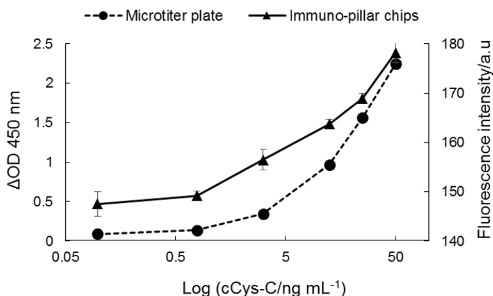
Figure 4. 4 Standard curves for cCys-C using the immuno-pillar chips (solid line with right Y-axis) and microtiter plate (dashed line with left Y-axis).
