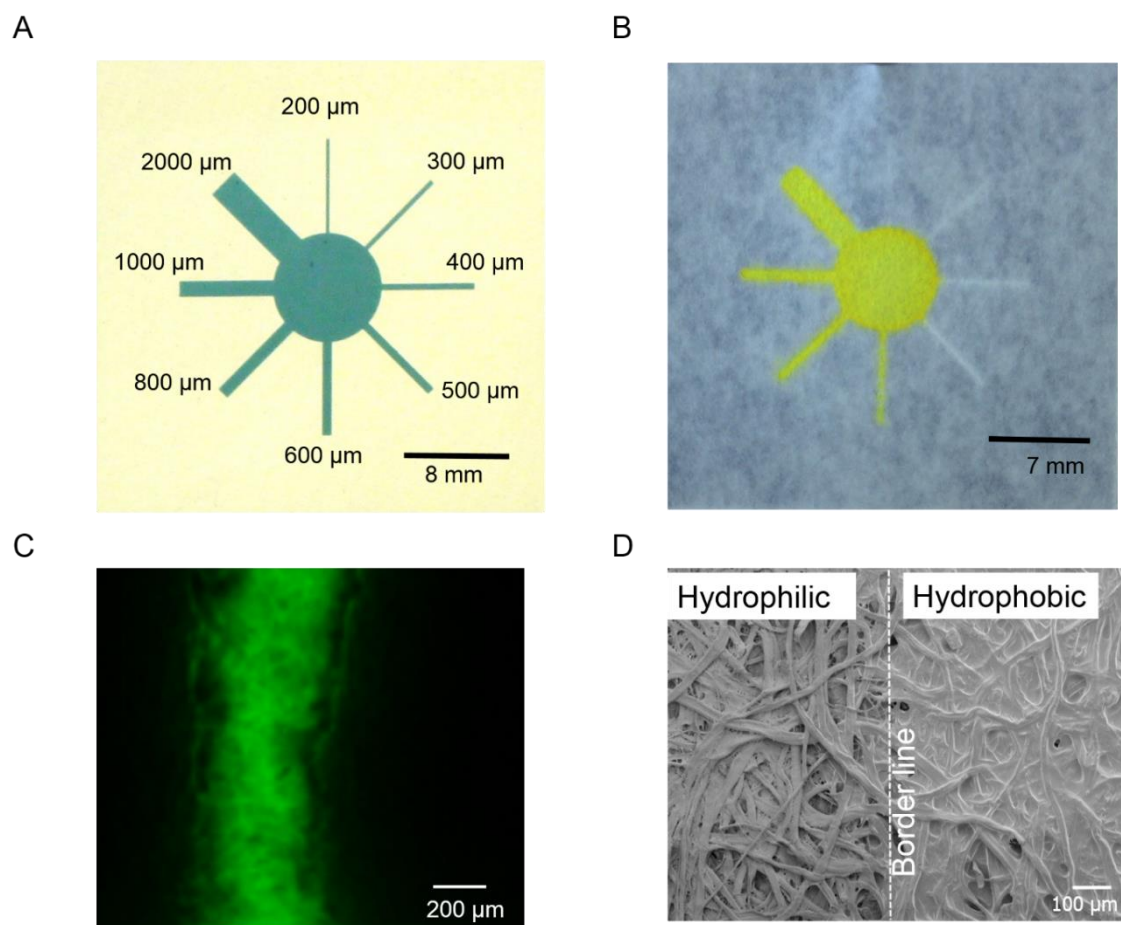
Figure 2.2 Evaluation of different channel widths. A) Patterned screen mesh for printing of different channel widths, B,C) comparison of the printed feature with the patterned screen and tracing the wicking property of them, D) SEM image of the bare (left) and PDMS printed paper (right).
