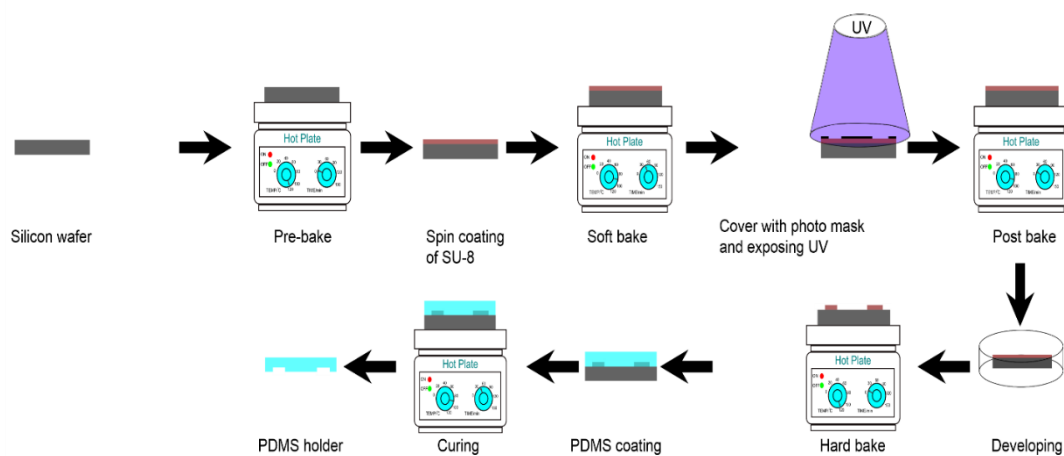
Figure 3. 1 Schematic of PDMS holder fabrication.
