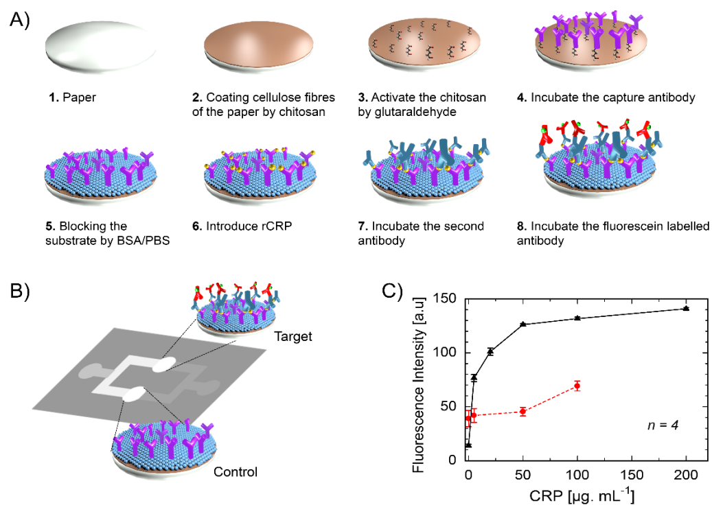
Figure 3. 6 A, B) Schematic drawings of CRP immunoassay. C) Standard curves for CRP assay. Black is the standard curve obtained by this study for the novel washing technique and red is the standard curve obtained by the conventional technique of washing the paper substrate.
