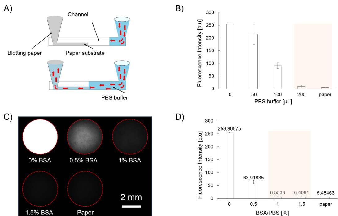
Figure 3. 5 Experiment to confirm washing and blocking of the paper substrate. A) Illustration of behaviour of solution in one channel after coming into contact with the paper substrate. B) Optimization of washing procedure (proper volumes of washing solution to remove unbound agents are highlighted). C) Fluorescence images of sample zones after applying different concentrations from 0 to 1.5% of BSA in PBS. D) Demonstration of proper amount of BSA in PBS to block the sample zones in order to prevent non-specific bonding of agents (recommended amount of BSA in PBS: 1 to 1.5 %).
