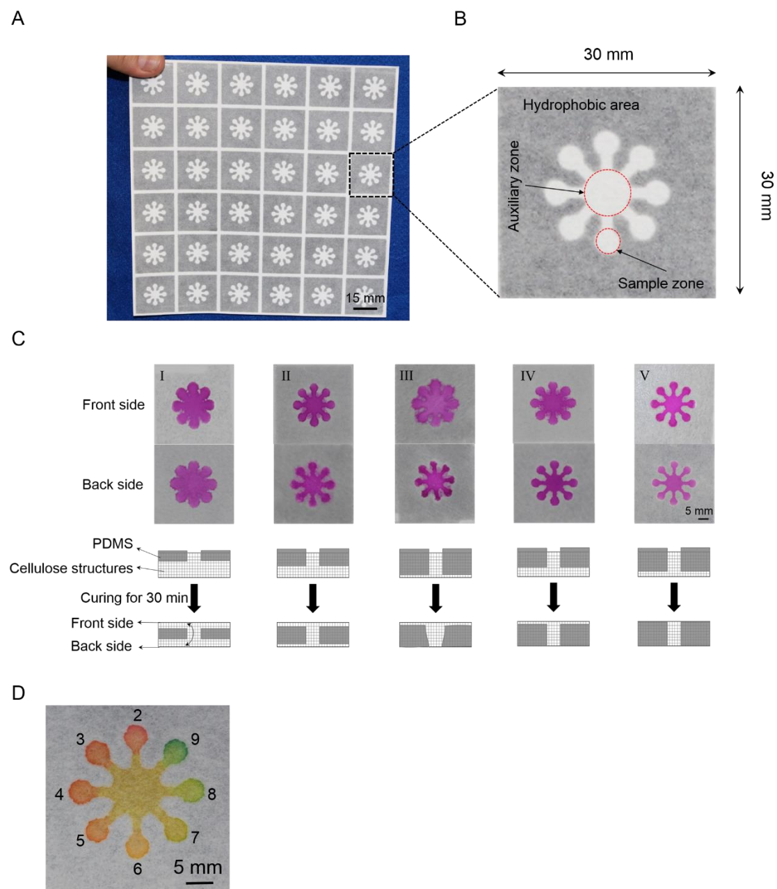
Figure 2.3 PDMS-screen-printing on a paper. A) Designing a new pattern (36 \mu PAD production one screen-printing). B) Details of each device. C) Optimising the printing procedures (All of devices were cured in an oven set at 120 °C for 30 min). I) Applying 15 g PDMS and rubbing once, II) applying 15 g PDMS and rubbing twice, III) applying 15 g PDMS and rubbing thrice, IV) applying 10 g PDMS and rubbing twice, V) applying 7 g PDMS and rubbing thrice. D) Results for different pH values (2 – 9). The colour of the sample zones changed from red at pH 2 to green at pH 9.
