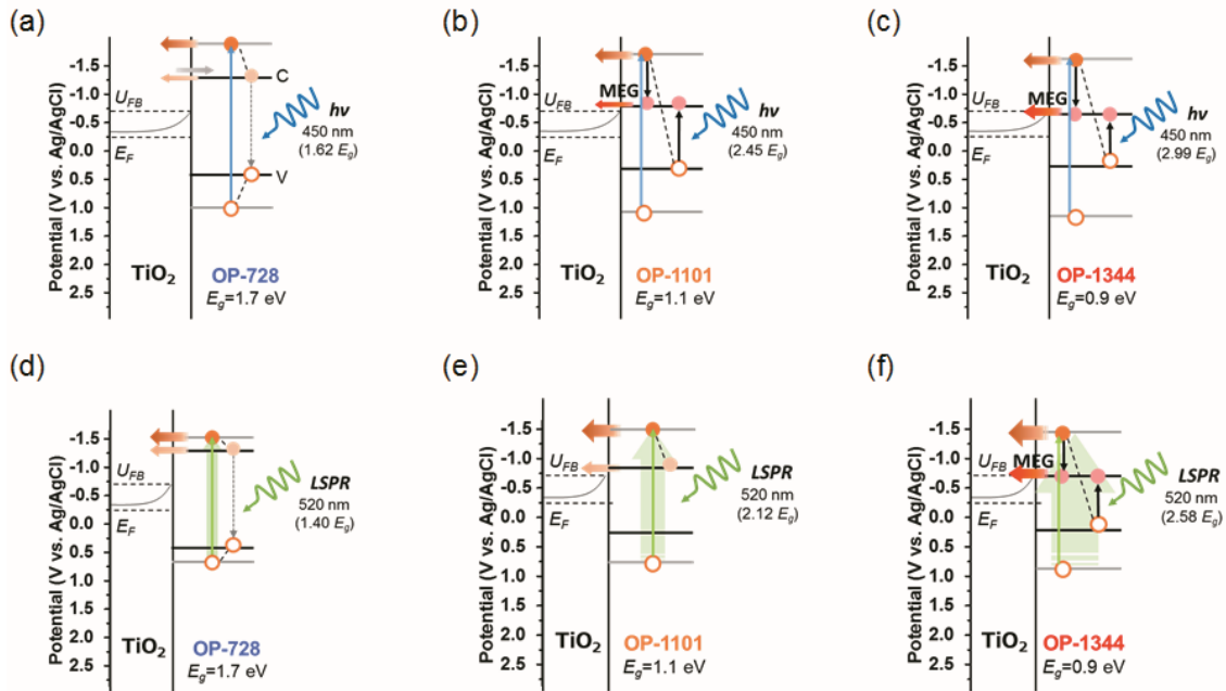
Figure 6.5. Schematic illustration of size-dependent PbS QDs sensitized bare \text{TiO}_2 under excitation of 450 nm (a, b and c) and \text{TiO}_2/\text{Au}/\text{TiO}_2 under LSPR excitation of 520 nm (d, e and f). Excitation by blue (450 nm, 2.76 eV, blue solid arrows) or green (520 nm, 2.38 eV, green solid arrows) visible light generated hot electrons (filled orange circles) and holes (empty orange circles) at higher energy levels (grey lines) than conduction band (labeled C) or valence band (labeled V). Cooled electrons (filled light orange circles) or holes relaxed to CB or VB via intraband relaxation (dashed lines) and a fraction undergo MEG (b, OP-1101 at 450 nm; c and f, OP-1344 at 450 and 520 nm; black arrows) to create biexciton (filled pink circles). Hot electron injection into \text{TiO}_2 from higher energy level without
