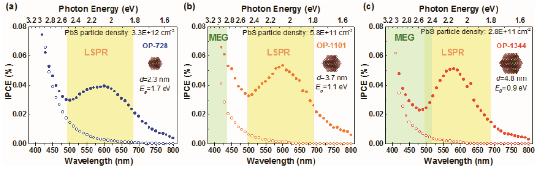
Figure 6.1. IPCE comparison of (a) OP-728, (b) OP-1101 and (c) OP-1344 PbS QDs sensitized \text{TiO}_2 and \text{TiO}_2/\text{Au}/\text{TiO}_2 substrates measured at -0.1 V in electrolyte of 0.05 M \text{Na}_2\text{S} +0.1 M NaOH. PbS particle densities within a single layer domain are 3.3 \times 10^{12} , 5.8 \times 10^{11} and 2.8 \times 10^{11} \text{ cm}^{-2} , respectively. The mole number density of PbS is around 0.5 \text{ nmol}/\text{cm}^2 for all.
