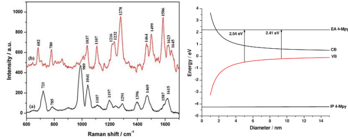
Figure 1.14. (Left) Comparison of the Raman spectrum of (a) 4-Mpy powder with that of (b) 4-Mpy adsorbed on 8.9 nm PbS quantum dot. Excitation is at 514.5 nm. . (Right) CT from size-dependent VB of PbS QDs to LUMO of 4-Mpy.
