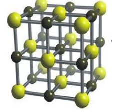
Figure 1.1 Rock salt
