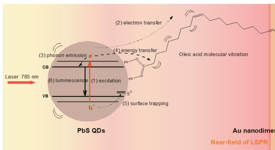
Figure 3.5. Scheme of possible processes of excited OA-capped PbS QDs/Au-NSL system by NIR of
