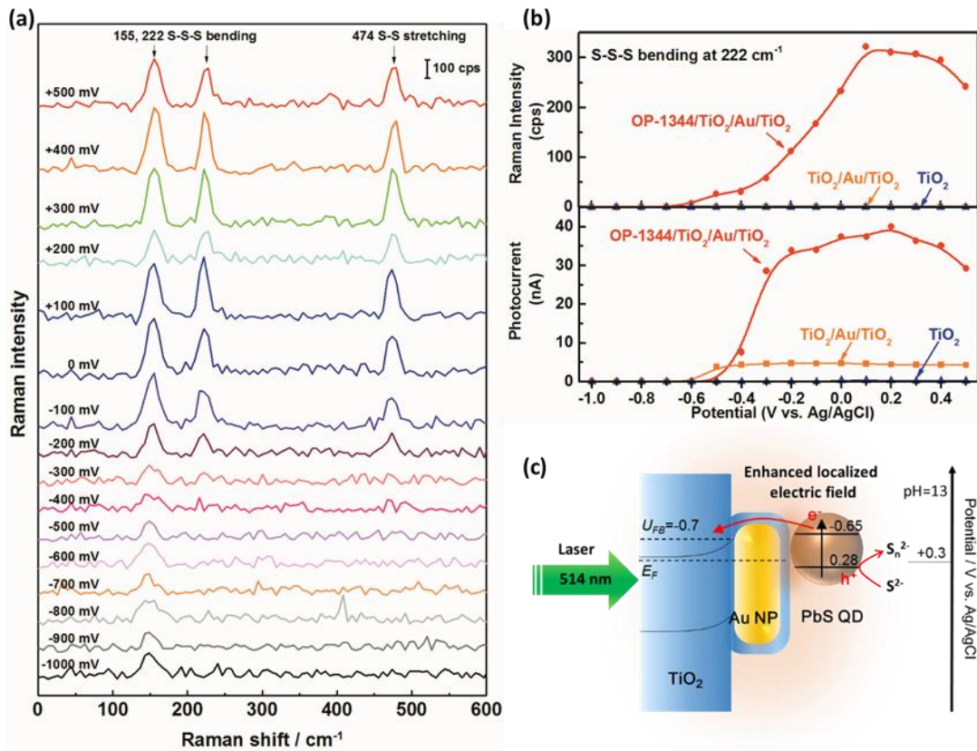
Figure 4.2. (a) EC-SERS spectrum of OP-1344/TiO 2 /Au/TiO 2 scanned potential from -1 V to +0.5 V
