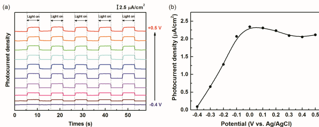
Figure A5.3. Potential-dependent (a) on-off action response of OA-capped PbS QDs/TiO 2 substrate, and (b) photocurrent density. Potential range: -0.4 ~ +0.5 V with 0.1 V interval (vs. Ag/AgCl sat.KCl), electrolyte: 0.05 M Na 2 S+0.1 M NaOH, irradiation wavelength range: 540~800 nm, light intensity: 1.7 mW/cm 2 , PbS particle density: 6 \times 10^{15} \text{ cm}^{-2} , PbS mole number density: 1.38 \mu\text{mol}/\text{cm}^2 .
