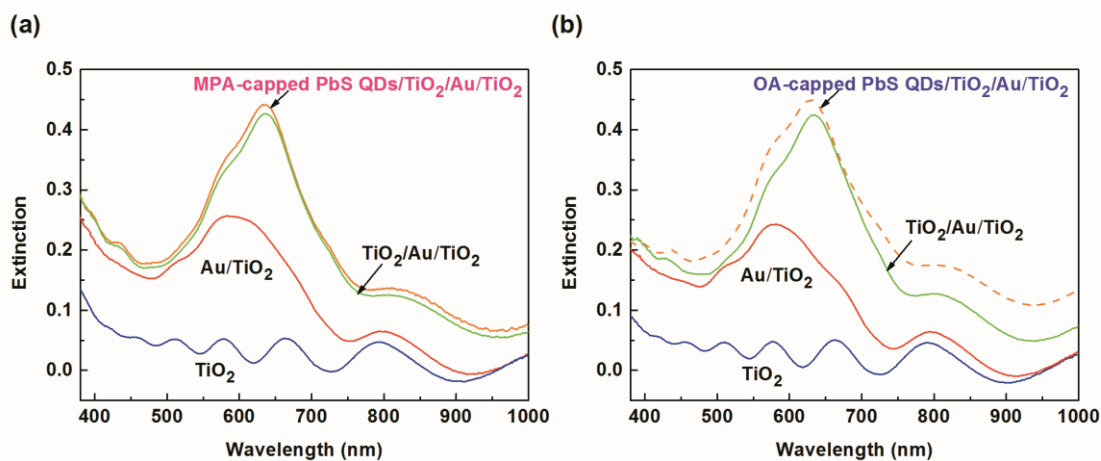
Figure A5.2. Extinction spectrum of (a) MPA- and (b) OA-capped PbS QDs sensitized substrate (PbS particle density: 1.2 \times 10^{13} \text{ cm}^{-2} ; PbS mole number density: 0.82 and 2.77 nmol/cm 2 for MPA- and OA-capped PbS QDs, respectively).
