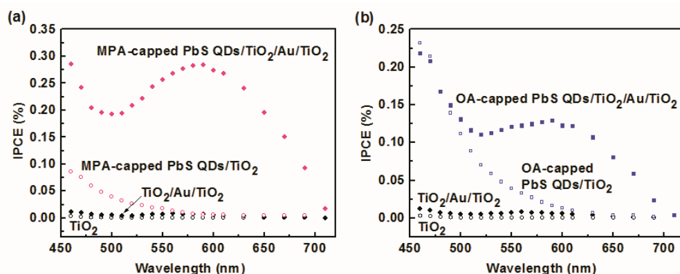
Figure 5.4. IPCE comparison of (A) MPA- and (B) OA- capped PbS QDs sensitized \text{TiO}_2 and \text{TiO}_2/\text{Au}/\text{TiO}_2 substrates. Measured at -0.1 V in electrolyte of 0.05 \text{ M Na}_2\text{S} + 0.1 \text{ M NaOH} . PbS particle densities are 7.2 \times 10^{12} \text{ cm}^{-2} and 4.8 \times 10^{12} \text{ cm}^{-2} , respectively for MPA- and OA-capped PbS QDs.
