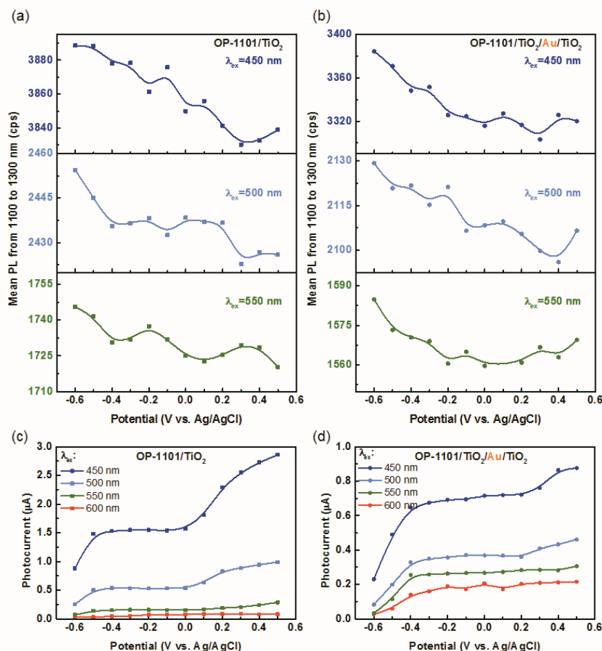
Figure 2.7. Potential-dependent (a, b) average photoluminescence from 1100 to 1300 nm and (c, d) simultaneous photocurrent for OP-1101 sensitized TiO 2 (square) and TiO 2 /Au/TiO 2 (circle) under excitation of 450 (blue), 500 (cyan), 550 (green) and 600 nm (red). The particle density of OP-1101: 1.2 \times 10^{12} \text{ cm}^{-2} .
