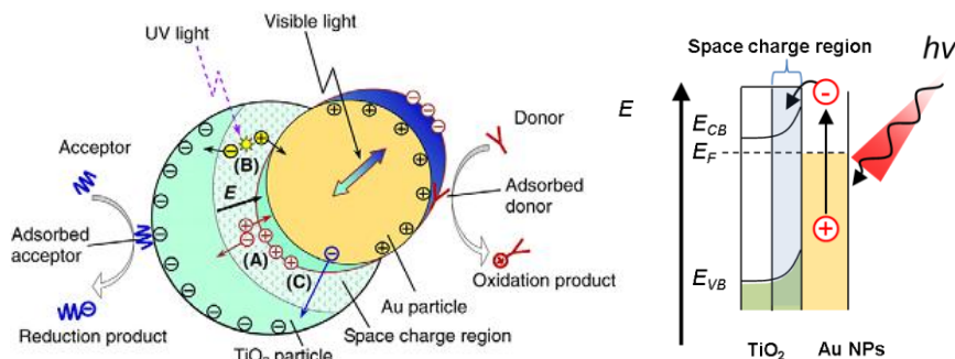
Figure 1.11. (Left) Schematic presentation of the major mechanisms 63 and (right) energy diagrams of plasmonic Au/TiO 2 solar cell.
