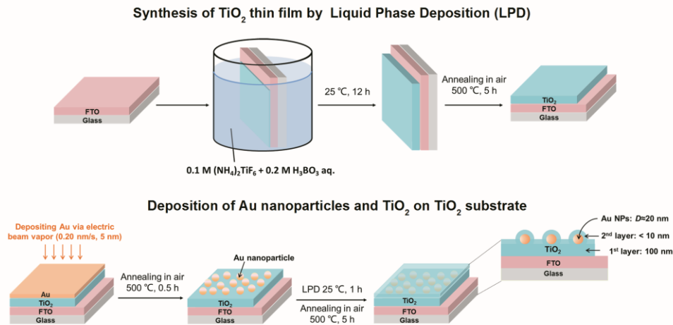
Figure 2.1. Schematic presentation of the preparation of TiO 2 /Au/TiO 2 electrode.
