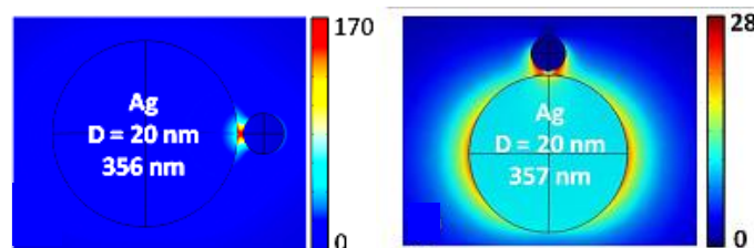
Figure 1.12. Electric field in the gap between a PbS QD ( D = 4.4 nm) placed 0.6 nm away from an Ag NP ( D = 20 nm) with the light polarization parallel (left) and perpendicular (right) to the dimer axis.
