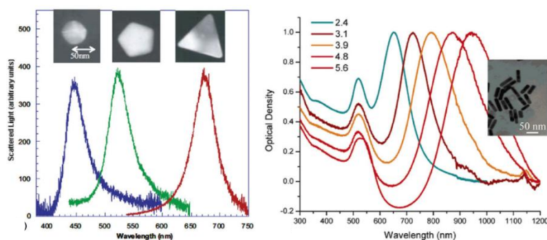
Figure 1.10. (Left) Scattering spectra of single Ag NPs in different shapes. 58 (Right) Absorption spectra of gold nanorods of different aspect ratios with longitudinal and transverse polar modes. 59
