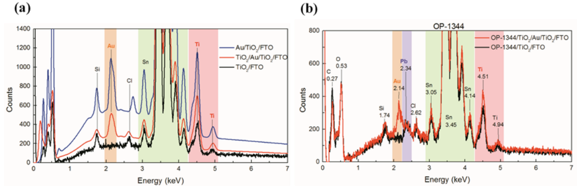
Figure A2.2. EDS spectrum of bare titanium dioxide and plasmonic electrode (a) before and (b) after sensitized by OP-1344 QDs (PbS particle density: 5.5 \times 10^{12} \text{ cm}^{-2} ).
