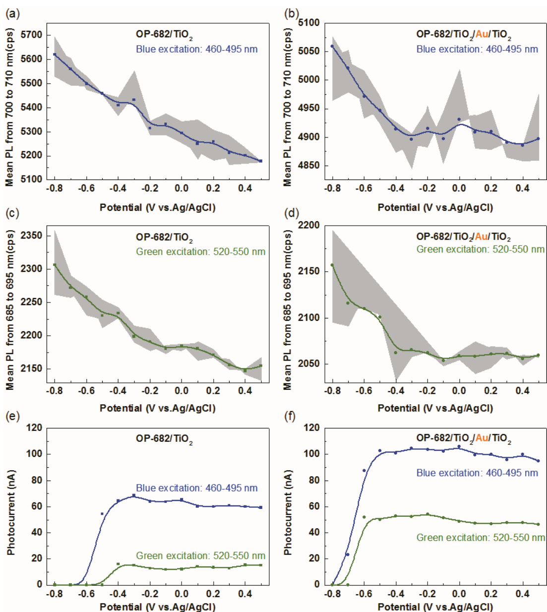
Figure 2.9. Potential-dependent average photoluminescence of OP-682 sensitized \text{TiO}_2 (left column) and \text{TiO}_2/\text{Au}/\text{TiO}_2 (right column) from 700 to 710 nm for the blue excitation (a, b) and from 685 to 695 nm for the green excitation (c, d) with the simultaneous photocurrent (e, f). Grey areas present the photoluminescence of three measurements under each potential.
