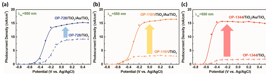
Figure 6.3. Comparison of J - V characteristics of (a, d) OP-728, (b, e) OP-1101 and (c, f) OP-1344 PbS QDs sensitized \text{TiO}_2 (dashed line and hollow symbols) and \text{TiO}_2/\text{Au}/\text{TiO}_2 (solid line and solid symbols) substrates scanned from negative to positive potential in electrolyte of 0.05 M \text{Na}_2\text{S} +0.1 M \text{NaOH} at irradiation of 550 nm. PbS particle densities within a single layer domain are 1.7 \times 10^{12} , 2.9 \times 10^{11} and 1.3 \times 10^{11} \text{ cm}^{-2} , respectively. The mole number density of PbS is all around 0.25 \text{ nmol}/\text{cm}^2 . Photocurrent density was normalized according to irradiating light intensity.
