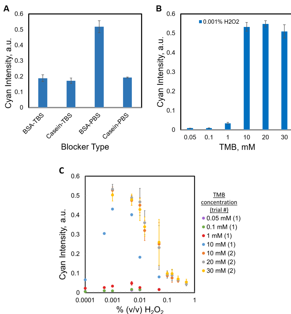
Figure 2-8 (A) Comparison of intensities produced during the HRP-TMB reaction using different blocking conditions ( n=2 ). (B) Signal intensities for TMB analysis with the optimum intensity at TMB concentration of 10 mM ( n=2 for 0.05 to 1 mM of TMB concentrations, and n=4 for 10 to 30 mM of TMB concentrations). (C) Signal intensities for 100 ng mL -1 of HRP in PBST containing an increasing amount of H 2 O 2 upon reaction with different concentrations of TMB: (1) from 0.05 to 10 mM of TMB ( n=2 ); and (2) from 10 to 30 mM of TMB ( n=4 ). The measured cyan intensity at 10 mM of TMB in trial (1) was slightly different from the cyan intensity at 10 mM of TMB
