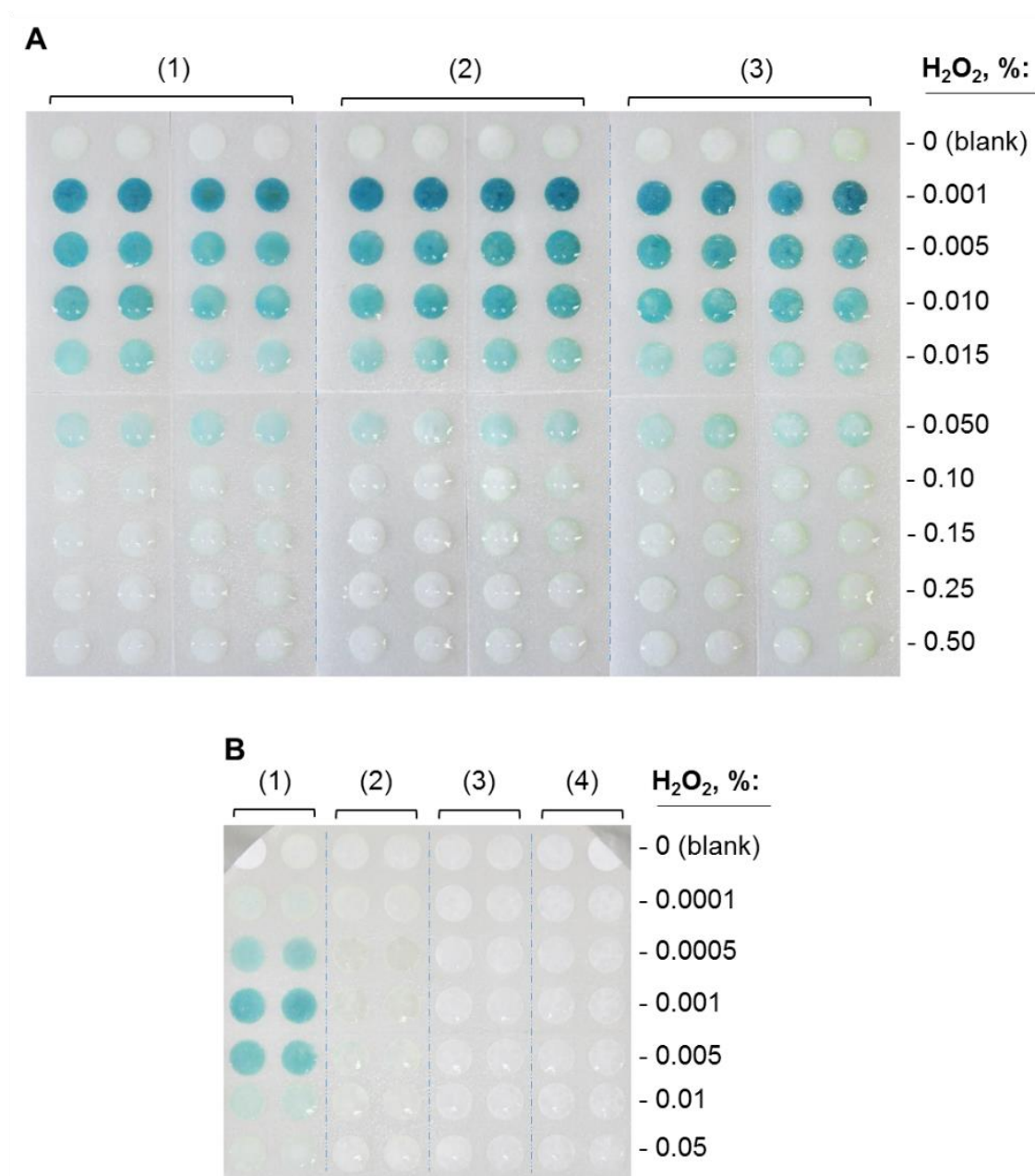
Figure 2-17 Digitally captured images of the \mu\text{PADs} used for simultaneous investigation of optimum TMB and \text{H}_2\text{O}_2 compositions. (A) The \mu\text{PAD} image showing intensities with TMB concentrations of (1) 10, (2) 20, and (3) 30 mM. (B)
