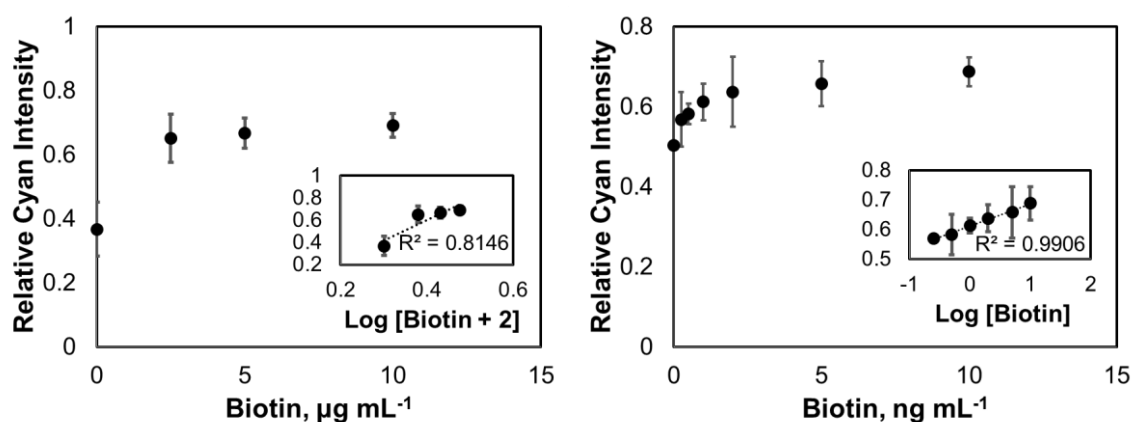
Figure 3-6 Biotin immunoassay on FP41 \mu PAD.
