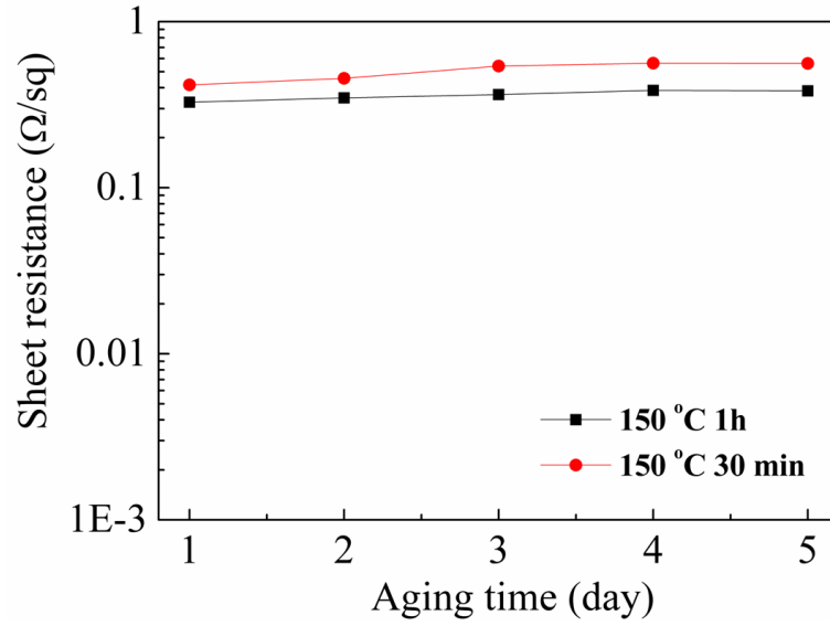
Fig. 3.5 Corresponding sheet resistance shifts of copper films using Cu/CuA-IPA-EtOH inks sintered at 150 °C at various time with time aging at room temperature in air.
