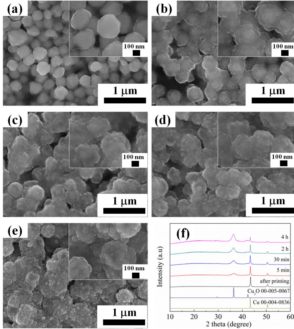
Fig. 2.6 Morphological images of copper A films after oxidative preheating at for various periods 200 °C: (a) 0 min, (b) 5 min, (c) 30 min, (d) 2 h, and (e) 4 h. (f) X-ray diffraction patterns.
