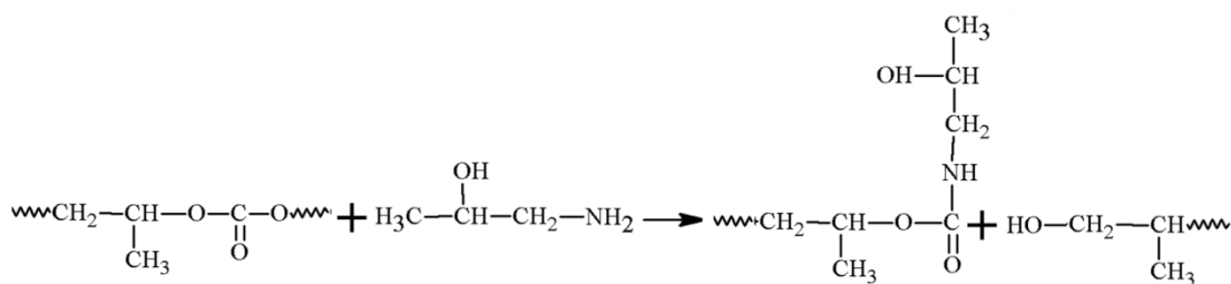
Fig. 4.8 The aminolysis reaction of PPC with IPA.
