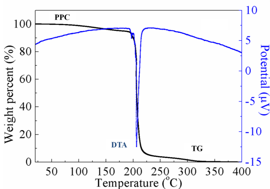
Fig. 4.7 DTA/TGA of PPC under a He gas flow.
