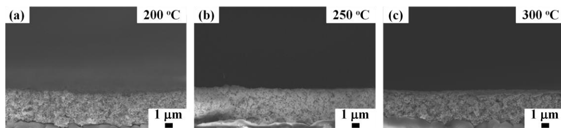
Fig. 2.3 The thicknesses of copper A films after annealing at various temperatures through a two-step process.
