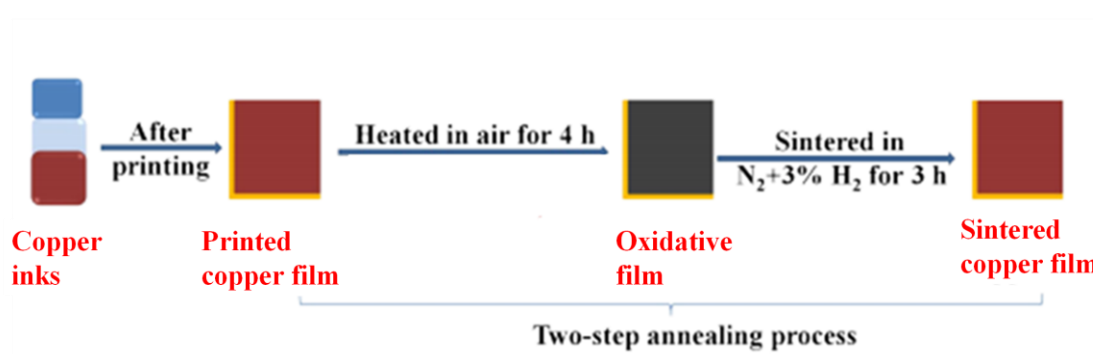
Fig. 2.4 Schematic illustration of two-step annealing process consisting of oxidative preheating process in air for 4 h (to enhance particle coalescence by generating convex surfaces, nanorods or nanoparticles) and sintering with a reductive gas containing 3% hydrogen-containing nitrogen gas for 3 h. The temperature in this two-step annealing process was kept for 200 °C, 250 °C or 300 °C.
