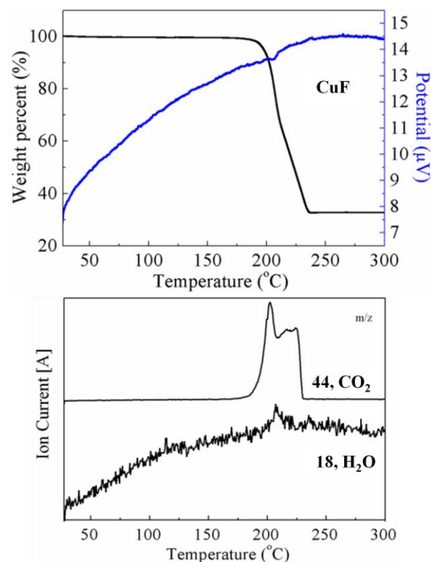
Fig. 4.6 DTA/TGA-MS of CuF. The mass to charge ratio ( m/z ) detected as decomposition product were CO 2 ( \text{amu}=44 ) and H 2 O ( \text{amu}=18 ).
