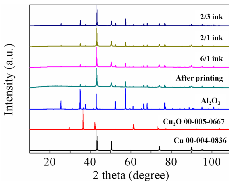
Fig. 4.10 XRD results of conductive copper films obtained following sintering process for 1 h at 100 °C by using PPC-Cu/CuF-IPA 6/1, 2/1 and 2/3 inks.
