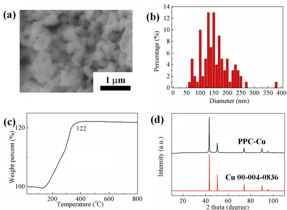
Fig. 4.1 (a) SEM image, (b) particle size distribution, (c) TG in air, and (d) XRD of the synthesized PPC-Cu particles.
