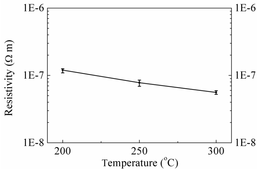
Fig. 2.13 Resistivity as a function of the two-step annealing temperature of copper A films after a two-step annealing process.
