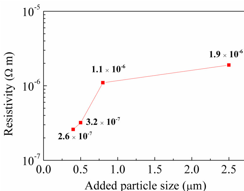
Fig. 3.7 Resistivities of the obtained copper films using Cu/CuF-IPA inks (CuF : IPA = 1 : 2 (mol/mol) inks after sintering at 120 ^{\circ}\text{C} for 30 min under a \text{N}_2 gas. The sizes of added commercial copper particles were 0.4, 0.5, 0.8, and 2.5 \mu\text{m} , respectively.
