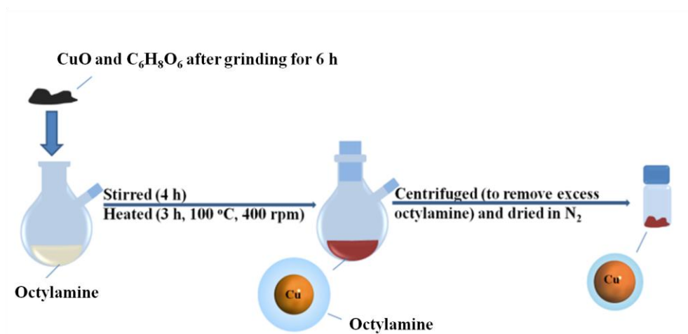
Fig. 2.1 Schematic illustration of one-pot synthesis of copper fine particles.
