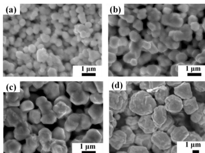
Fig. 3.8 Morphological images of the conductive copper films following sintering at 120 °C by using the Cu/CuF-IPA inks with added copper particles with various sizes: (a) 0.4, (b) 0.5, (c) 0.8, and (d) 2.5 \mu\text{m} . In the prepared ink, the molar ratio of CuF to IPA was 1 to 2 and the weight amount of added copper particles was 50 wt%.
