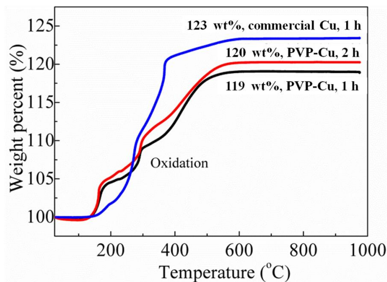
Fig. 3.12 TG curves of conductive copper films following sintering at 100 °C by using Cu (0.4 \mu\text{m}\phi , commercial particles)/CuF-IPA inks for 1 h (CuF : IPA = 1 : 2 (mol/mol), 50 wt% Cu) (blue) and PVP-Cu/CuF-IPA inks for 1 h (black) and 2 h (red).
