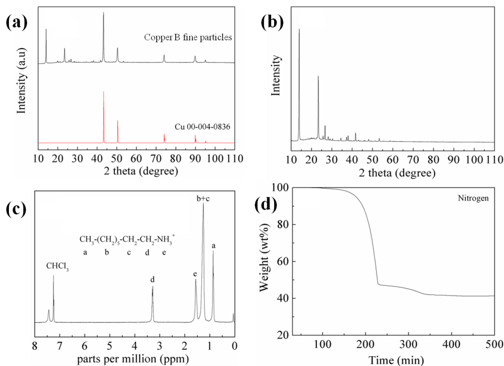
Fig. 2.2 XRD patterns of (a) copper B fine particles which contain much protonated octylamine and (b) Protonated octylamine. (c) NMR spectra of protonated octylamine. (d) TG curves of copper B fine particles in nitrogen.
