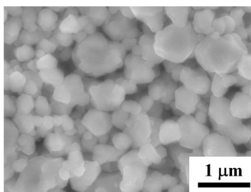
Fig. 4.12 Morphological image of copper films obtained following sintering process at 100 °C for 2 h, by using the PPC-Cu/CuF-IPA 2/3 ink.
