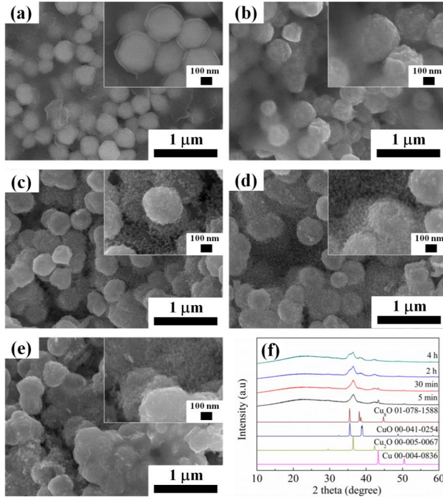
Fig. 2.9 SEM of copper B films after oxidative preheating process at 250 °C for various heating periods: (a) 0 min, (b) 5 min, (c) 30 min, (d) 2 h, and (e) 4 h. (f) Corresponding XRD patterns.
