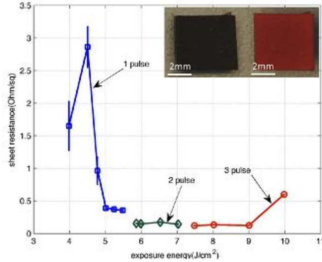
Fig. 1.10 Sheet resistance of Cu layer after IPL sintering vs. energy exposure and number of pulses. The pulse duration is 6 ms and the frequency for multi pulses is 10 Hz. The as-printed CuO (left) and IPL-sintered Cu (right) were also shown in the figure. 31
