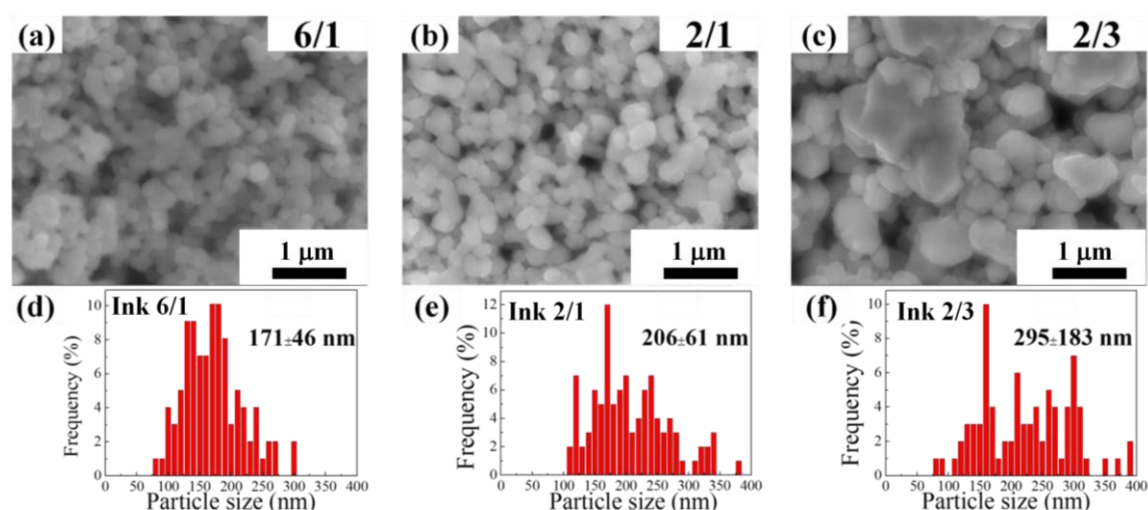
Fig. 4.11 Surface morphologies (a, b, and c) and relevant size distributions (d, e, and f) of the obtained copper films following sintering process at 100 °C for 1 h, by using PPC-Cu/CuF-IPA 6/1, 2/1 and 2/3 mixed inks, respectively.
