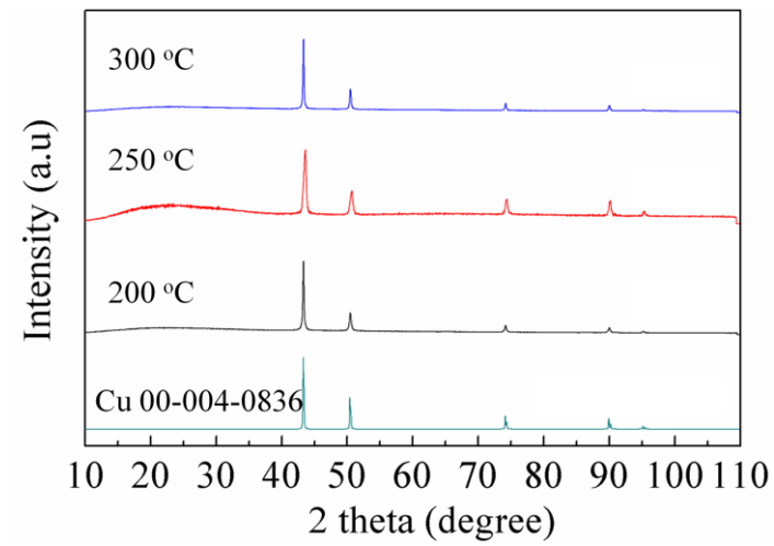
Fig. 2.12 XRD patterns of copper A films after two-step annealing process at 200 °C, 250 °C and 300 °C, respectively.
