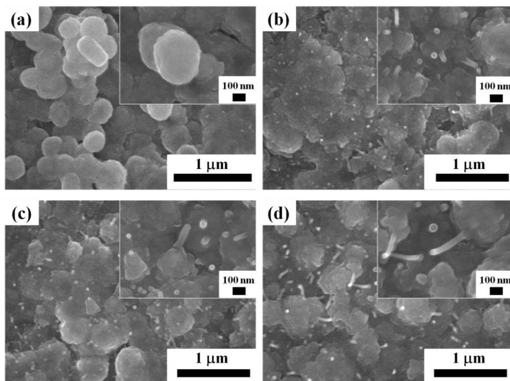
Fig. 2.7 Morphological images of copper A films after oxidative preheating at 250 °C for various periods: (a) 5 min, (b) 30 min, (c) 2 h, and (d) 4 h.
