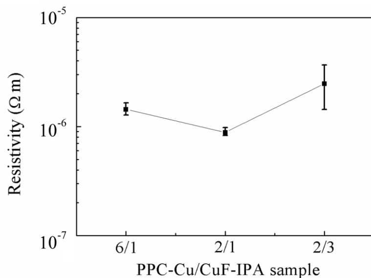
Fig. 4.9 Resistivities of the conductive copper films obtained using various copper inks shown in Table 4.1, after sintering process under a N 2 atmosphere at 100 °C for 1 h.
