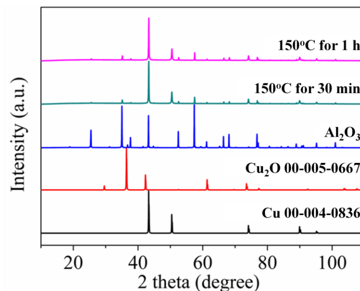
Fig. 3.4 XRD of the sintered copper films using Cu/CuA-IPA-EOH inks after sintering under a N 2 flow at 150 °C for various periods.
