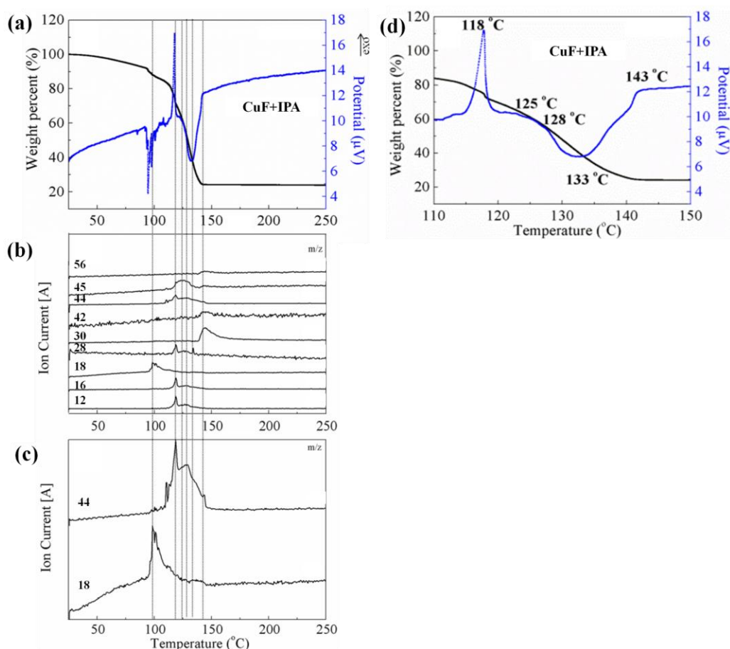
Fig. 4.5 DTA/TGA-MS of CuF-IPA complex (CuF:IPA=1:1, mol/mol) under a He gas flow: (a) DTA/TGA, (b) fragments obtained during the decomposition and corresponding MS results (mass to charge ratio ( m/z ) versus temperature), (c) magnification of MS spectra presented in (b) for m/z of 18 and 44, (d) DTA/TGA of CuF-IPA complex from 110 to 150 °C. The mass to charge ratios ( m/z ), obtained as the main decomposition products and their fragments, were C ( \text{amu}=12 ), \text{CH}_4 ( \text{amu}=16 ), \text{H}_2\text{O} ( \text{amu}=18 ), (CO or \text{CH}_2\text{CH}_2 ) ( \text{amu}=28 ), (\text{CH}_4\text{N}) ( \text{amu}=30 ), (\text{CH}_3\text{CHCH}_2) ( \text{amu}=42 ), \text{CO}_2 ( \text{amu}=44 ), \text{HCOO} ( \text{amu}=45 ), and ((\text{CH}_2)_2\text{CO}) ( \text{amu}=56 ).
