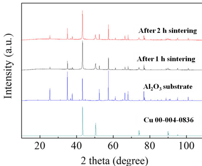
Fig. 3.13 XRD of conductive copper films got by using PVP-Cu/CuF-IPA inks after sintering process for 1 and 2 h at 100 °C (CuF : IPA = 1 : 1 (mol/mol), 30 wt% PVP-Cu).
