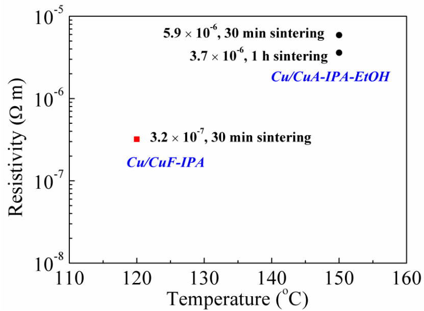
Fig. 3.6 Resistivities of obtained copper films using Cu/CuF-IPA and Cu/CuA-IPA-EtOH inks after sintering process at various temperatures.
