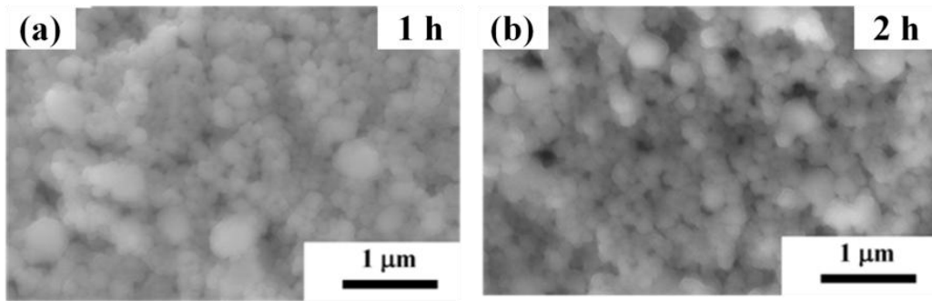
Fig. 3.11 Morphological images of copper films obtained using PVP-Cu/CuF-IPA inks after sintering at 100 °C for 1 and 2 h. (CuF : IPA = 1 : 2 (mol/mol), 50 wt% Cu).
