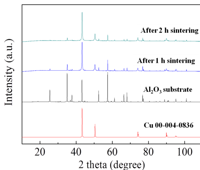
Fig. 3.10 XRD of copper films obtained from PVP-Cu/CuF-IPA inks (CuF : IPA = 1 : 2 (mol/mol), 50 wt% PVP-Cu) following sintering process under a \text{N}_2 flow at 100^\circ\text{C} for 1 and 2 h.
