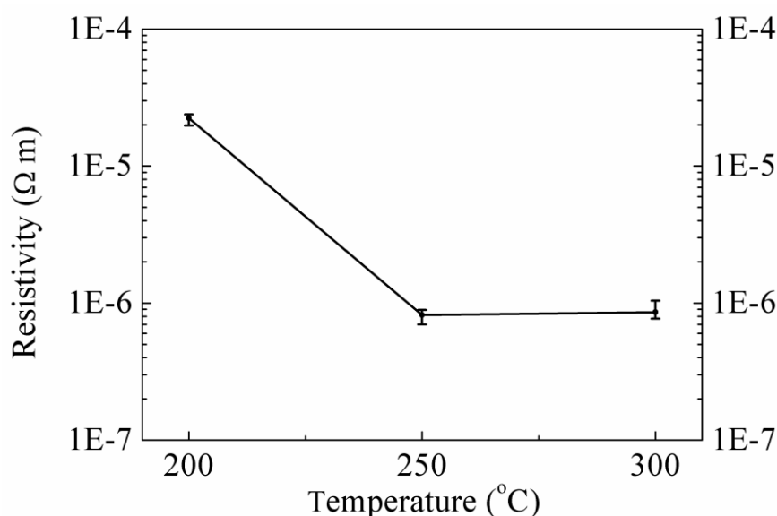
Fig. 2.14 Resistivity as a function of the two-step annealing temperature of copper B films after a two-step annealing process.
