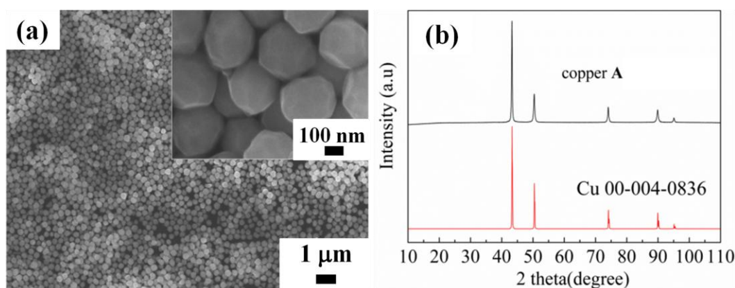
Fig. 2.5 (a) Morphologies and (b) XRD pattern of copper A fine particles.
