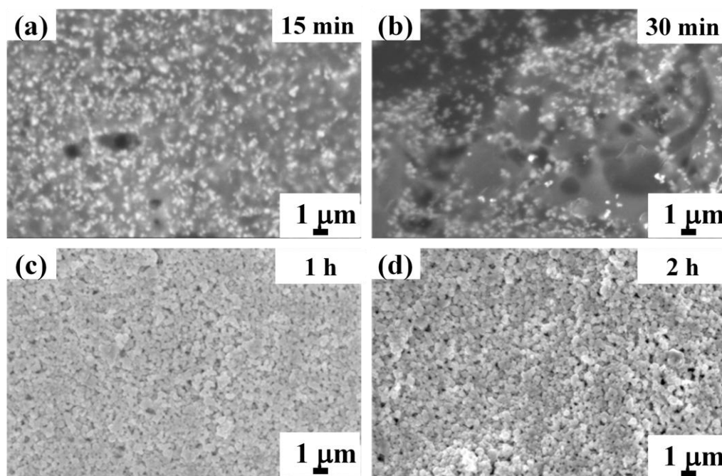
Fig. 4.14 Surface images of the copper films obtained using the PPC-Cu/CuF-IPA 2/1 ink after sintering process at 100 °C for (a) 15 min, (b) 30 min, (c) 1 h, and (d) 2 h.
