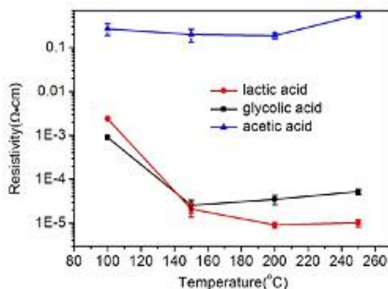
Fig. 1.2 Resistivity of the copper films obtained by sintering different capping agents stabilized copper particles at various temperatures under nitrogen. 21
