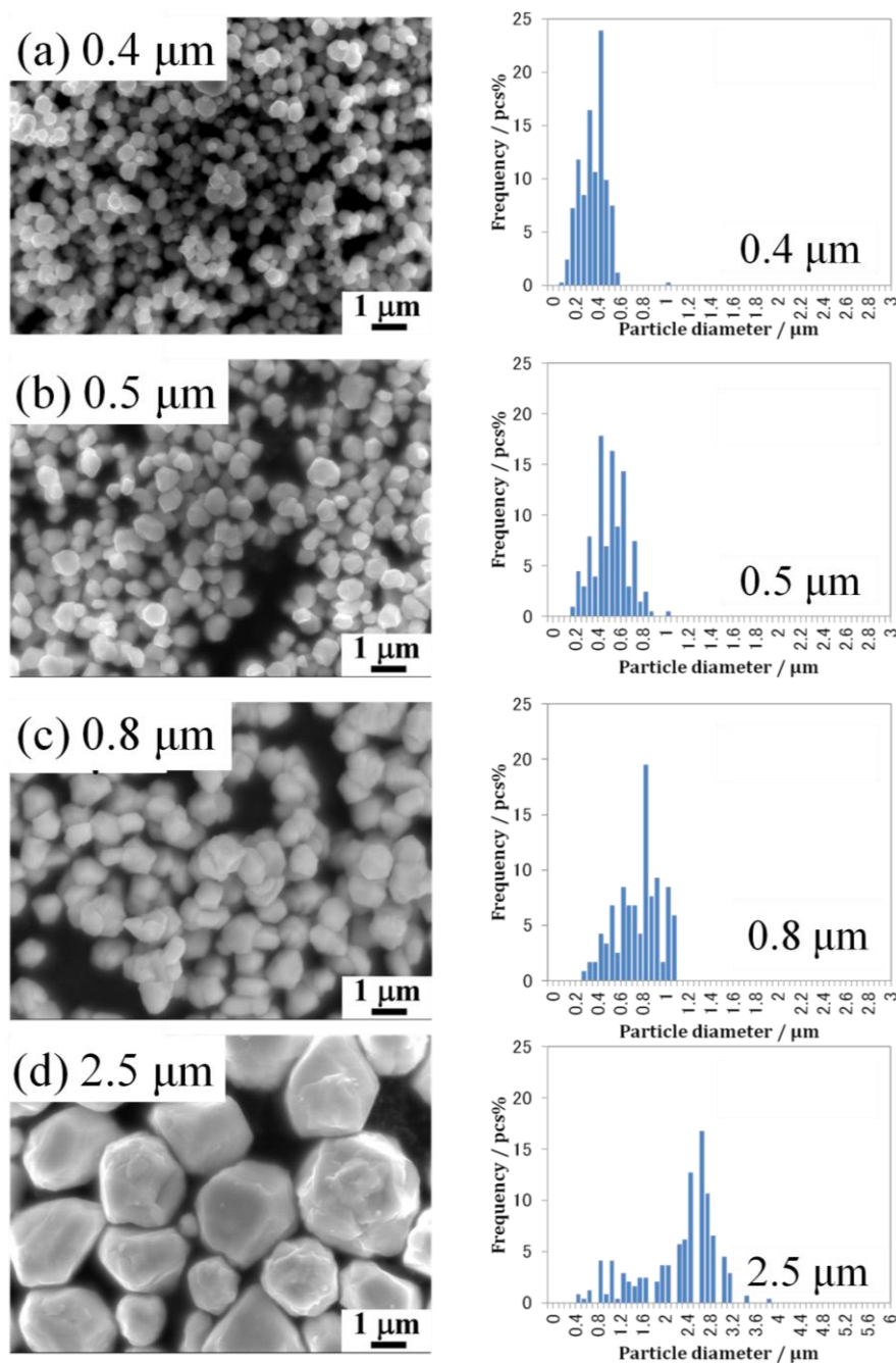
Fig. 3.1 SEM images and size distributions of added commercial copper fine particles. The average sizes of added copper particles were (a) 0.4 \mu\text{m} , (b) 0.5 \mu\text{m} , (c) 0.8 \mu\text{m} and (d) 2.5 \mu\text{m} .
