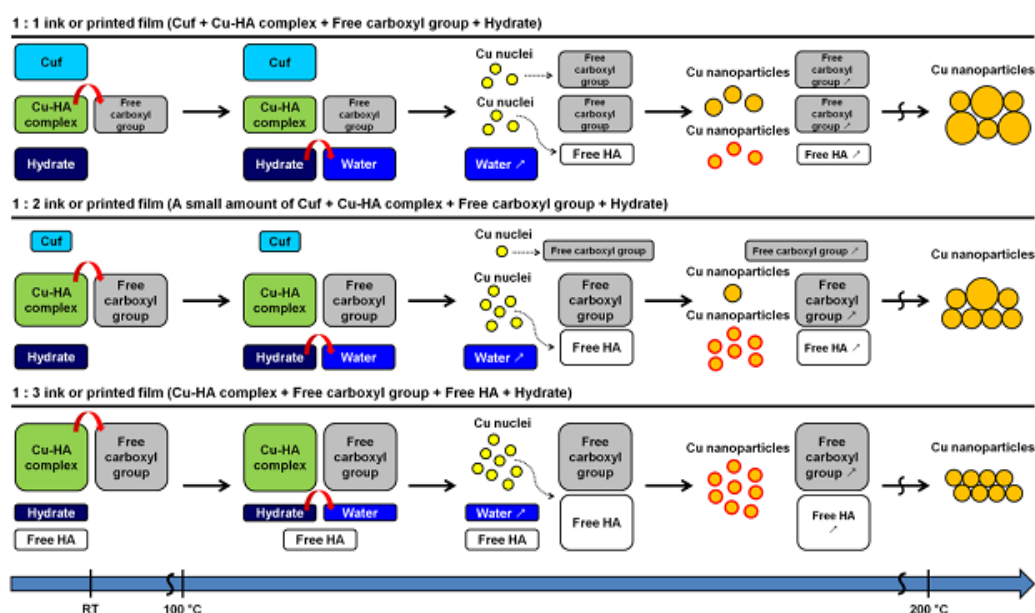
Fig. 1.8 Schematic diagram explaining microstructure formation during the thermal heating process with various amine concentrations in CuF-HA complex ink. 28
