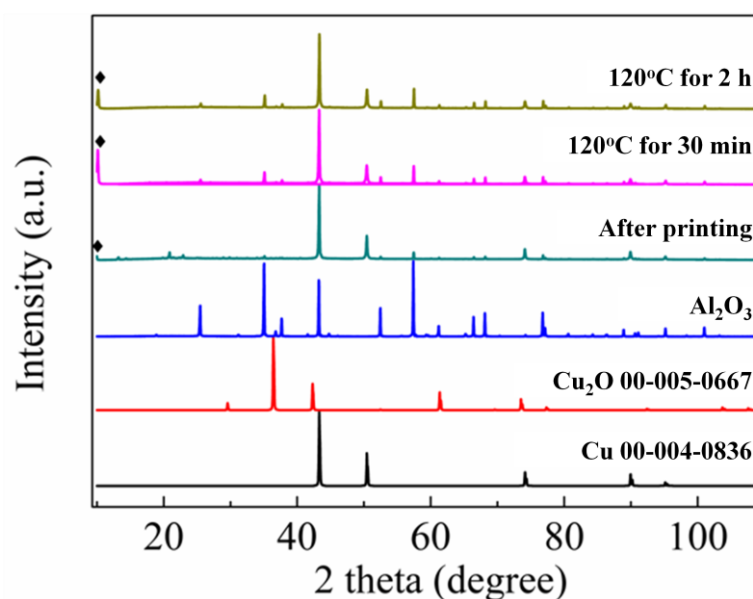
Fig. 3.3 XRD of the sintered copper films using Cu/CuA-IPA-EOH inks after printing and sintering under a N 2 flow at 120 °C for various periods.
