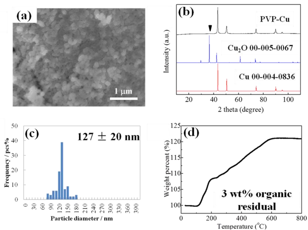
Fig. 3.9 Morphological image (a), XRD pattern (b), size distribution (c) and TG (d) of prepared PVP-Cu particles. The TG measurement was performed in air from room temperature to 800\ ^\circ\text{C} .
