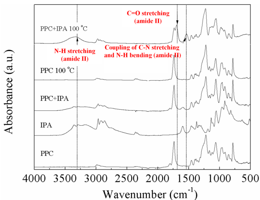
Fig. 4.15 FTIR spectra of PPC, IPA, and PPC+IPA (PPC:IPA=1:1, weight ratio) without heating, and PPC and PPC+IPA (PPC:IPA=1:1, weight ratio) after heating under a N 2 gas at 100 °C for 3 h.
