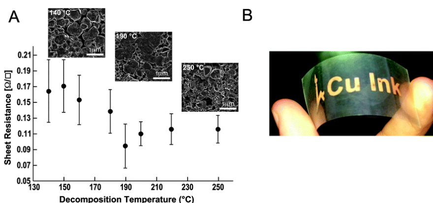
Fig. 1.6 (A) Sheet resistance of obtained conductive Cu films as a function of decomposition temperature. The inset SEM images are corresponding micrographs at various decomposition temperatures. (B) Copper patterns on PET film using the copper complex with ink-jet printing technique. 25
