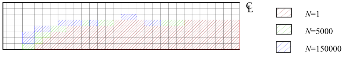
Fig. 3.10 Propagation of cracked elements due to fixed pulsating load equaling 80%
