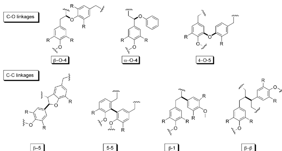
Figure 4. C-O and C-C linkages between monolignols
