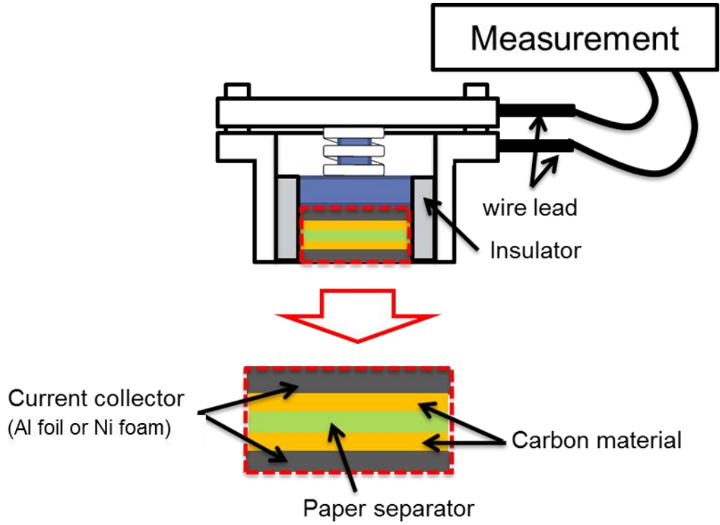
Figure 22. Structure of SC-EDLC
