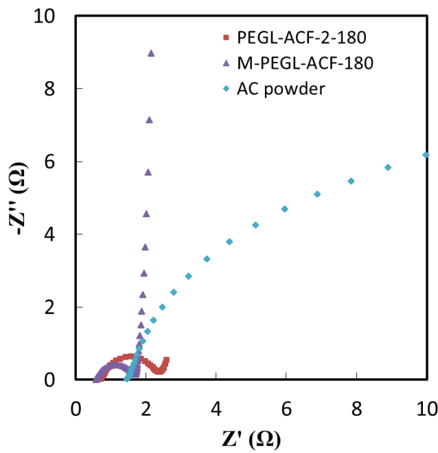
Figure 34. Nyquist plots of \text{EDLC}_{\text{E-PEGL-ACF-180}} , \text{EDLC}_{\text{M-PEGL-ACF-180}} and \text{EDLC}_{\text{AC powder}}
