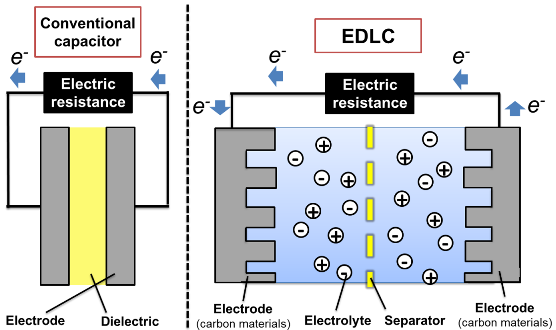
Figure 7. Formations of electric double layer in an EDLC and single layer in a conventional capacitor
