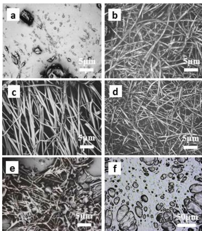
Figure 12. Microscopic images of electrospinning products at different concentrations of HAL/AcOH solution, a), 30 wt%; b), 35 wt%; c), 40 wt%, and thermostabilization products at different heating rates, d), 0.1^{\circ}\text{C min}^{-1} ; e), 0.3^{\circ}\text{C min}^{-1} ; f), 0.5^{\circ}\text{C min}^{-1} . (precursor, electrospun fiber derived from 35 wt% HAL/AcOH solution)
