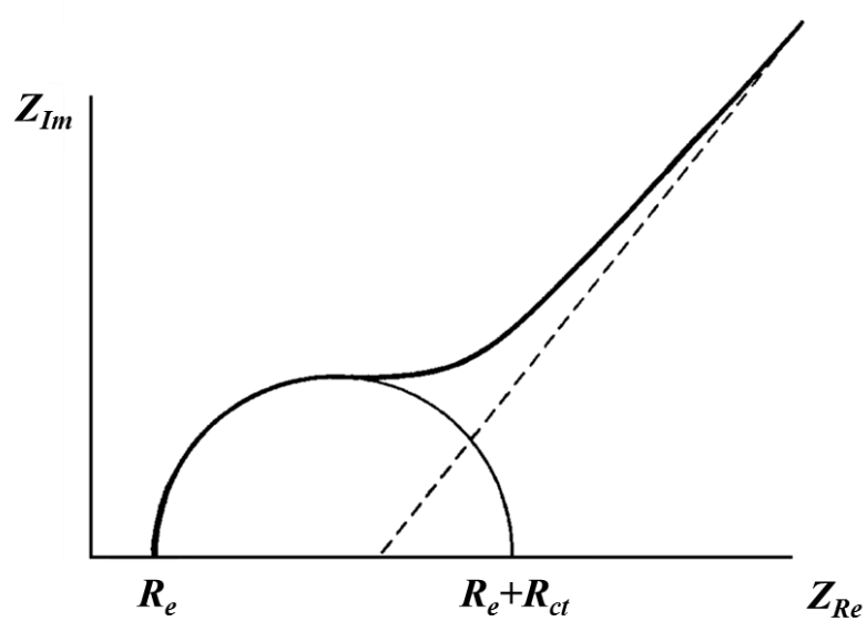
Figure 24 Nyquist diagram for randles equivalent circuit
