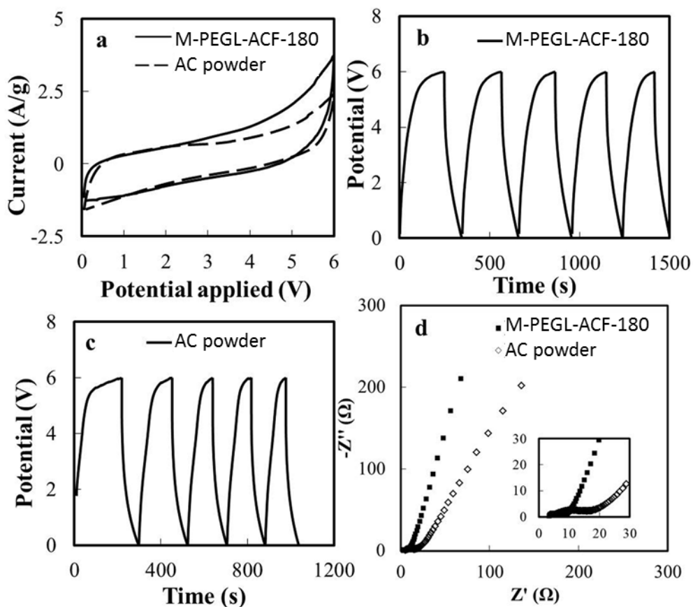
Figure 36. Electrochemical performance of IT-EDLC connected in series: (a) the CV curves of IT-EDLC M-PEGL-ACF-180 and IT-EDLC AC powder at a scan rate of 0.05 \text{ V s}^{-1} ; (b) the GCD profile of IT-EDLC M-PEGL-ACF-180 ; (c) the GCD profile of IT-EDLC AC powder at a current density of 1 \text{ A g}^{-1} ; and (d) the Nyquist plots of IT-EDLC M-PEGL-ACF-180 and IT-EDLC AC powder , where the inset shows magnified profiles of the high frequency range.
