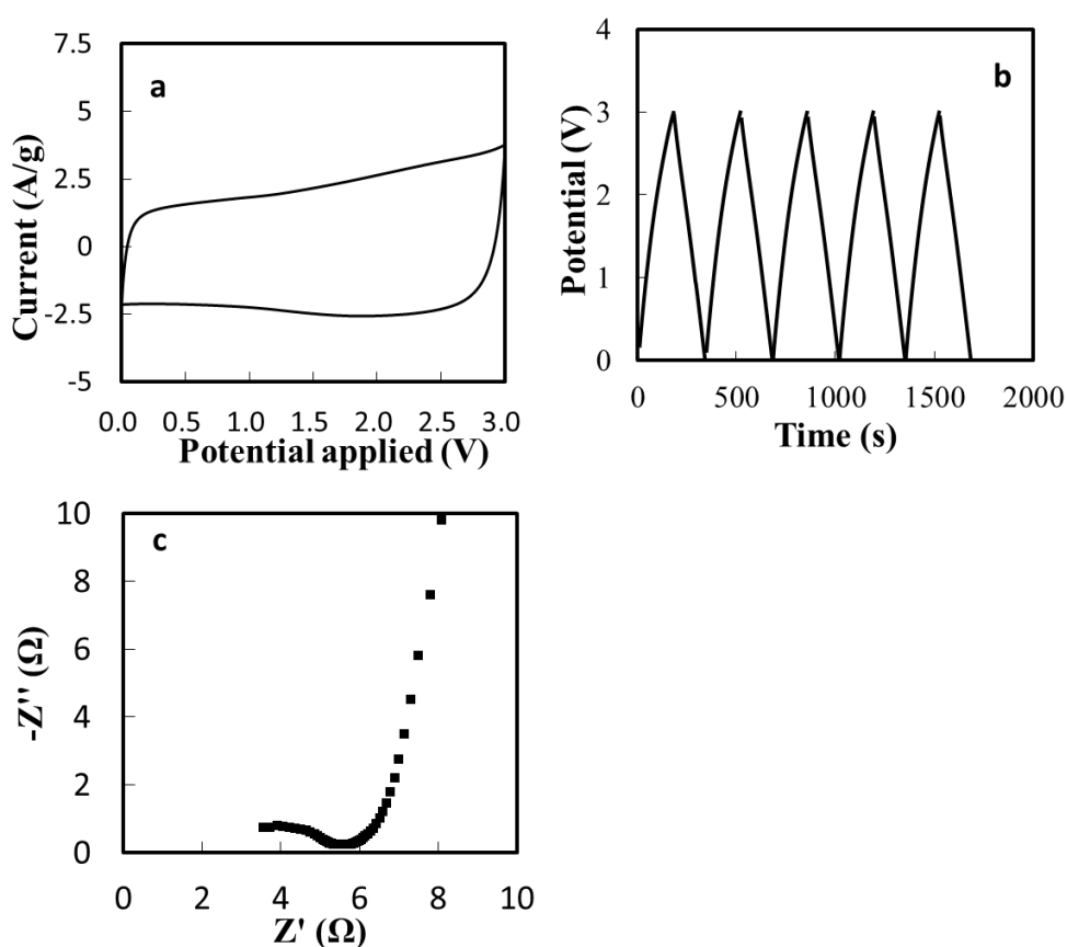
Figure 31. Electrochemical properties of \text{EDLC}_{\text{M-PEGL-ACF-180}} : (a) CV curves at a scan rate of 0.05 \text{ V s}^{-1} ; (b) GCD profiles, and (c) the Nyquist plot.
