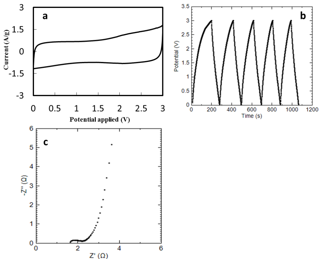
Figure 29. Electrochemical characterization of EDLC E-PEGL-ACF-180 . a) Cyclic voltammogram, b) GCD profile, and c) Nyquist plot.
