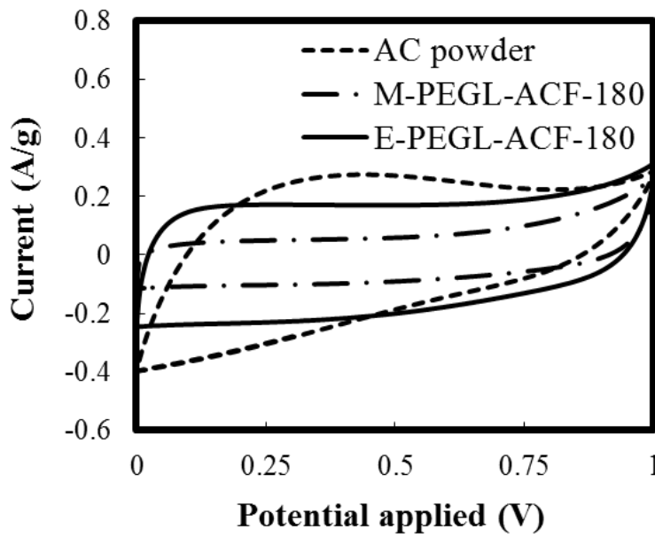
Figure 32. Cyclic voltammograms of \text{EDLC}_{\text{E-PEGL-ACF-180}} , \text{EDLC}_{\text{M-PEGL-ACF-180}} and \text{EDLC}_{\text{AC powder}} with aqueous electrolyte at the scan rate of 0.005 \text{ V s}^{-1} .
