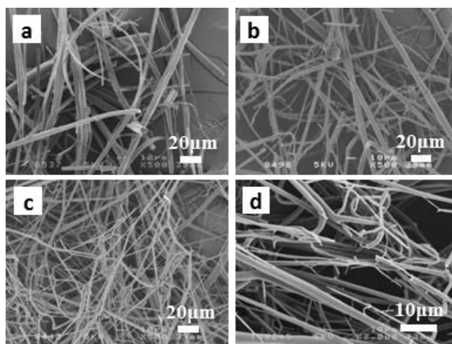
Figure 13. SEM images of lignin based fibrous products at 10 wt% of hexamine content, a), electrospun fibers; b), thermostabilized fibers; c), E-HAL-CF; and d) E-HAL-ACF-105.
