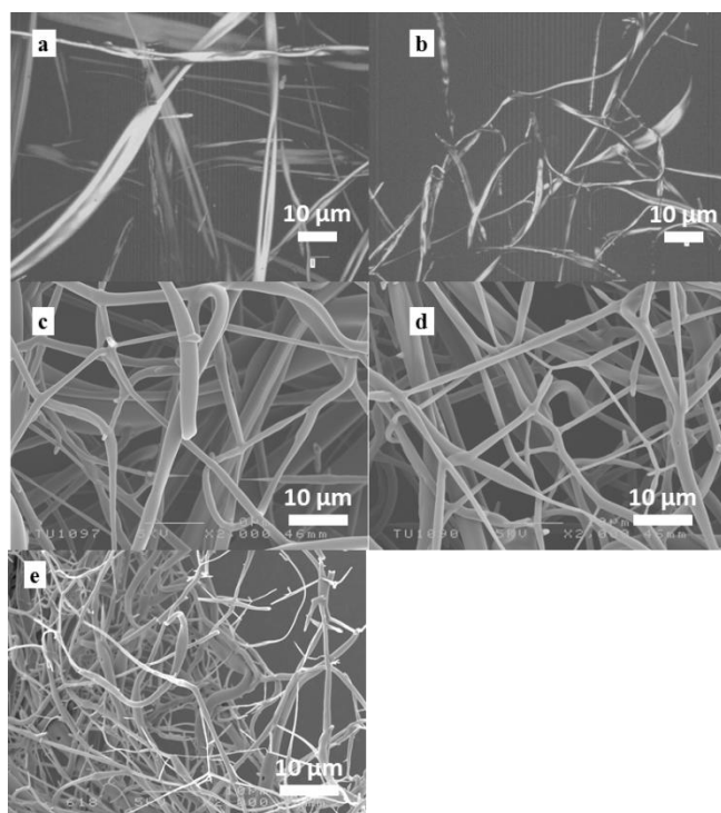
Figure 16. SEM images of PEGL based fibrous products with 10 wt% hexamine a) electrospun fibers; b) thermostabilized fibers c) CFs; d) E-PEGL-ACF-105; e) E-PEGL-ACF-180
