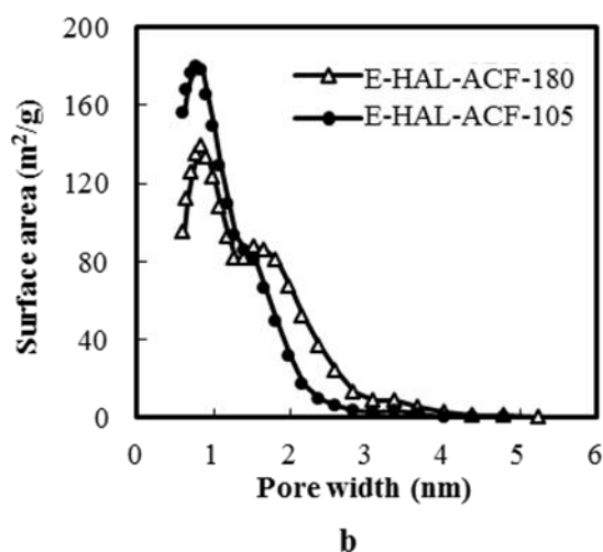
Figure 21. Surface area distribution of carbon materials in the pore range of 0.6-5.0 nm (calculated by using a slit pore QSDFT model)
