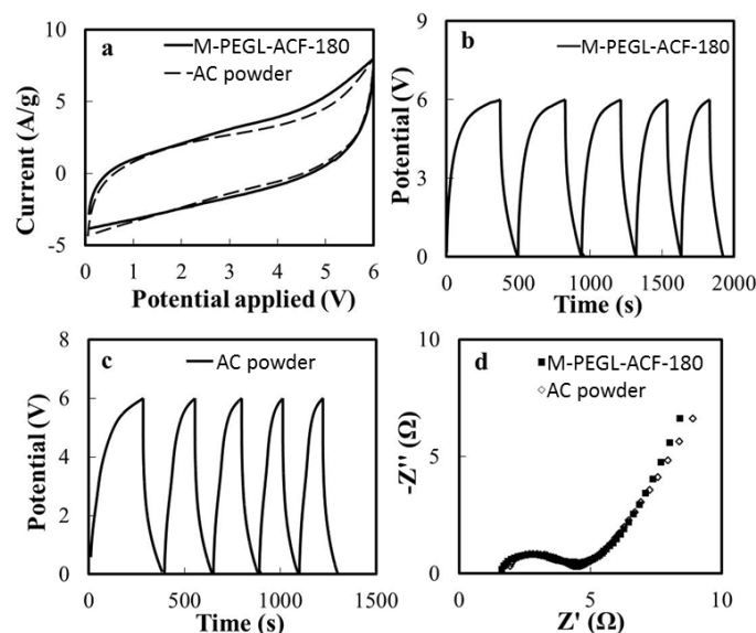
Figure 38. Electrochemical performance of IT-EDLC connected in the S/P comb.: (a) the CV curves of IT-EDLC M-PEGL-ACF-180 and IT-EDLC AC powder at a scan rate of 0.05 V s -1 ; (b) the GCD profile of IT-EDLC M-PEGL-ACF-180 ; (c) the GCD profile of IT-EDLC AC powder at a current density of 2 A g -1 ; and (d) the Nyquist plots of IT-EDLC M-PEGL-ACF-180 and IT-EDLC AC powder .
