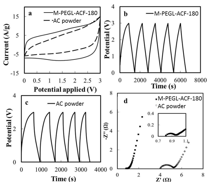
Figure 37. Electrochemical performance of IT-EDLC connected in parallel: (a) the CV curves of IT-EDLC M-PEGL-ACF-180 and IT-EDLC AC powder at a scan rate of 0.05 \text{ V s}^{-1} ; (b) the GCD profile of IT-EDLC M-PEGL-ACF-180 ; (c) the GCD profile of IT-EDLC AC powder at a current density of 1 \text{ A g}^{-1} ; and (d) the Nyquist plots of IT-EDLC M-PEGL-ACF-180 and IT-EDLC AC powder , where the inset shows the magnified profile of IT-EDLC M-PEGL-ACF-180 in the high frequency range.
