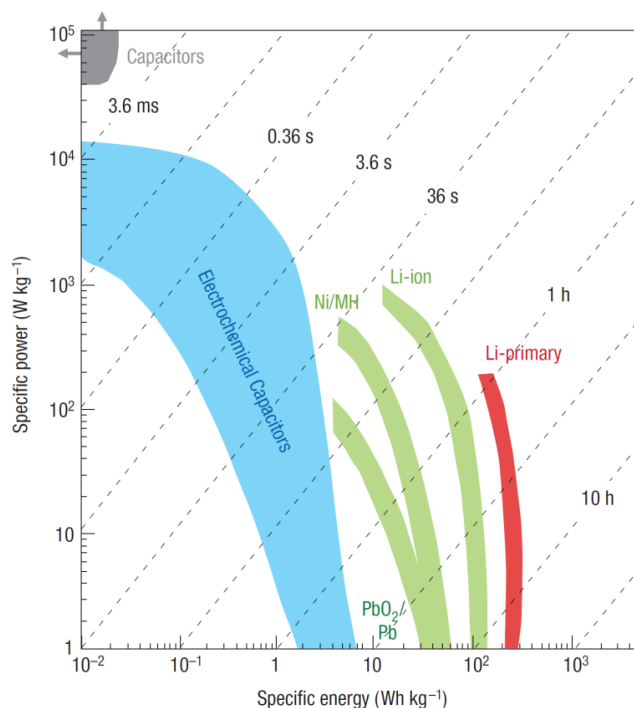
Figure 1. Ragone plot showing the specific power against specific energy for various electrical energy storage systems. If a supercapacitor is used in an electric vehicle, the specific power shows how fast one can go, and the specific energy shows how far one can go on a single charge. Times shown are the time constants of the devices, obtained by dividing the energy density by the power (Simon and Gogotsi, 2008)
