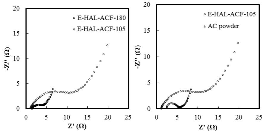
Figure 27. Nyquist plots of E-HAL-ACF-180, E-HAL-ACF-105 and AC powder based EDLCs
