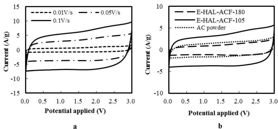
Figure 25. Cyclic voltammograms of \text{EDLC}_{\text{E-HAL-ACFs}} and \text{EDLC}_{\text{AC powder}} . a) \text{EDLC}_{\text{E-HAL-ACF-105}} at different scan rates and b) comparison of \text{EDLC}_{\text{E-HAL-ACF-180}} , \text{EDLC}_{\text{E-HAL-ACF-105}} and \text{EDLC}_{\text{AC powder}} at 0.05 \text{ V s}^{-1} .
