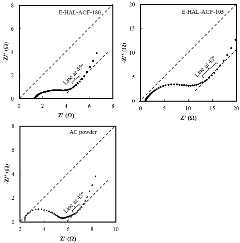
Figure 28. Diffusion resistance of E-HAL-ACFs and AC powder represented in the Nyquist plots.
