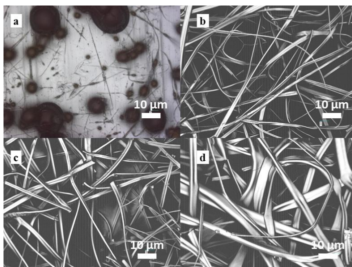
Figure 15. Microscopic images of electrospinning products with different HAL/AcOH/ \text{CCl}_4 solution concentration, a), 25wt %; b), 30 wt%; c),35 wt%; d),40 wt%.
