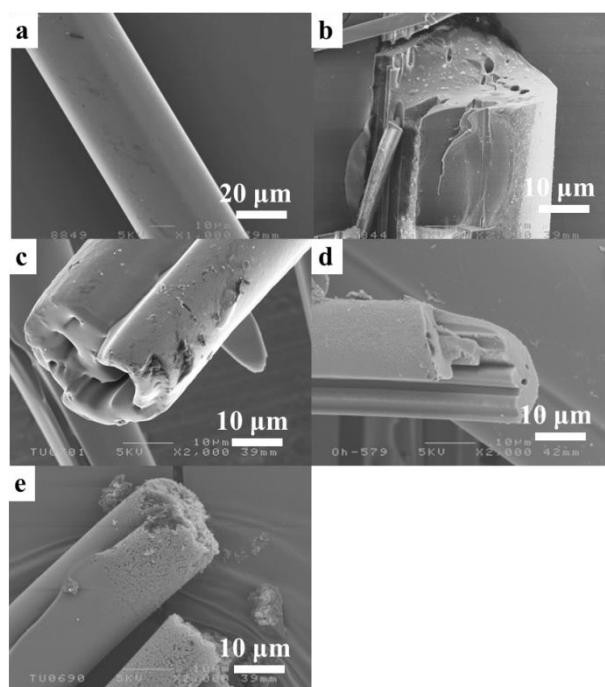
Figure 20. SEM images of PEGL based fibrous products: (a) melt-spun fibers; (b) chemical thermostabilized fibers; (c) carbon fibers; (d) M-PEGL-ACF-105; and (e) M-PEGL-ACF-180.
