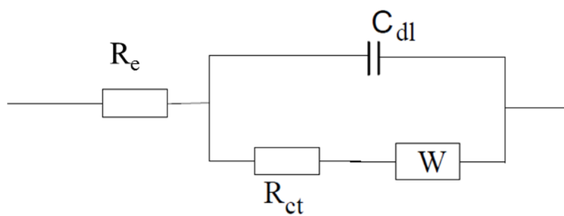
Figure 23 Randles equivalent circuit
