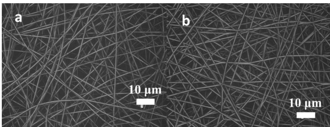
Figure 17. Microscopic images of electrospun SL fibers a) before thermostabilization; b) after thermostabilization at 5 °C min -1
