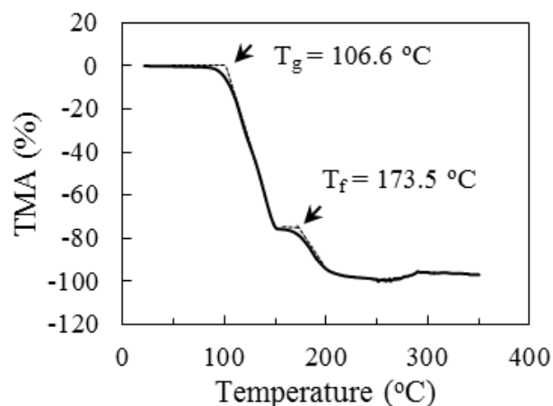
Figure 19. TMA of PEGL powder
