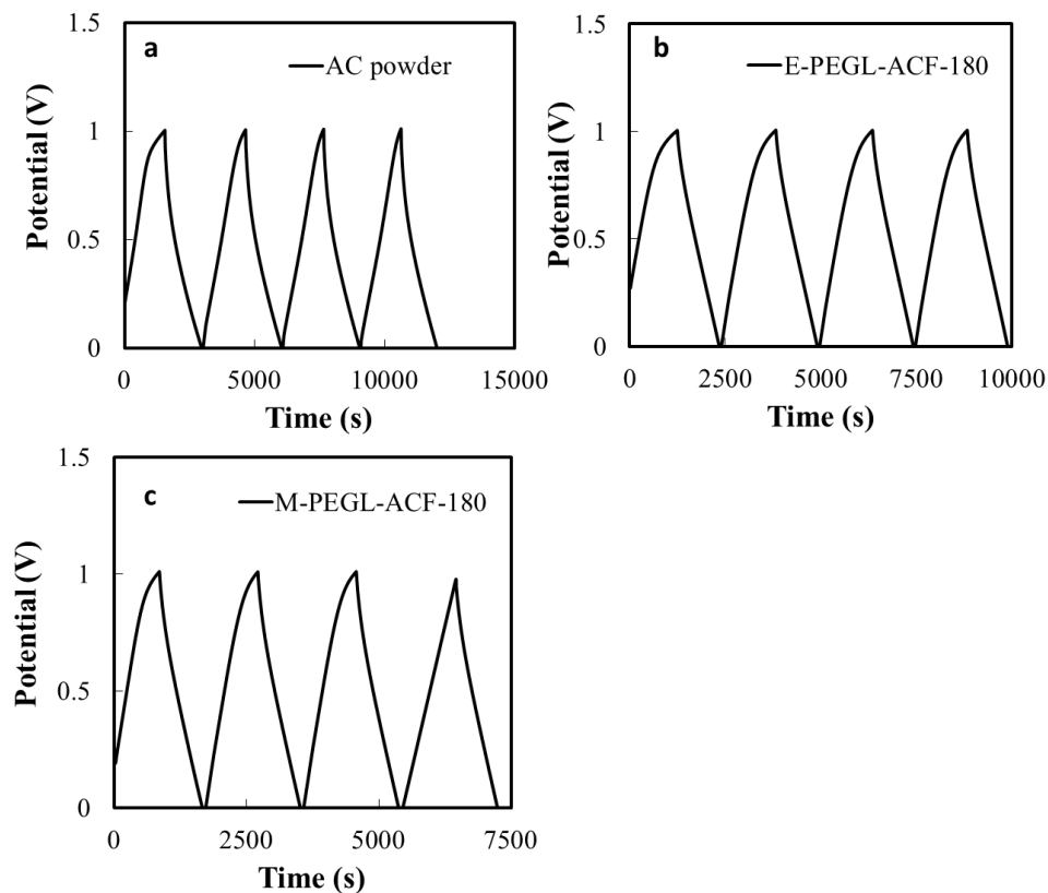
Figure 33. GCD profiles of a) \text{EDLC}_{\text{AC powder}} , b) \text{EDLC}_{\text{E-PEGL-ACF-180}} and c) \text{EDLC}_{\text{M-PEGL-ACF-180}} under a current density of 0.05 \text{ A g}^{-1}
