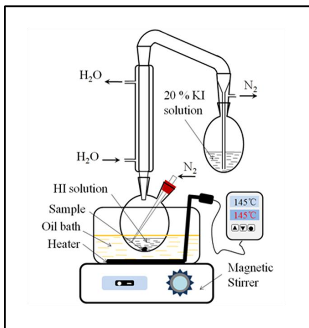
Figure 11. Scheme for PEG content measurement
