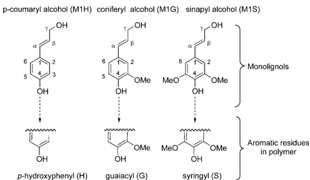
Figure 3. Monolignol carbon nomenclature and residues
