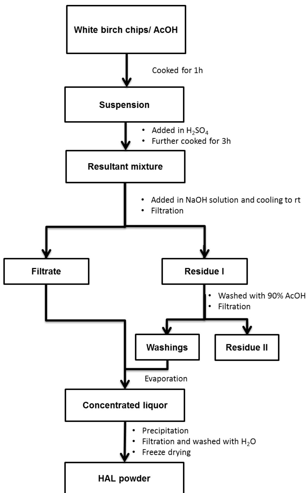
Figure 9. Preparation scheme of HAL
