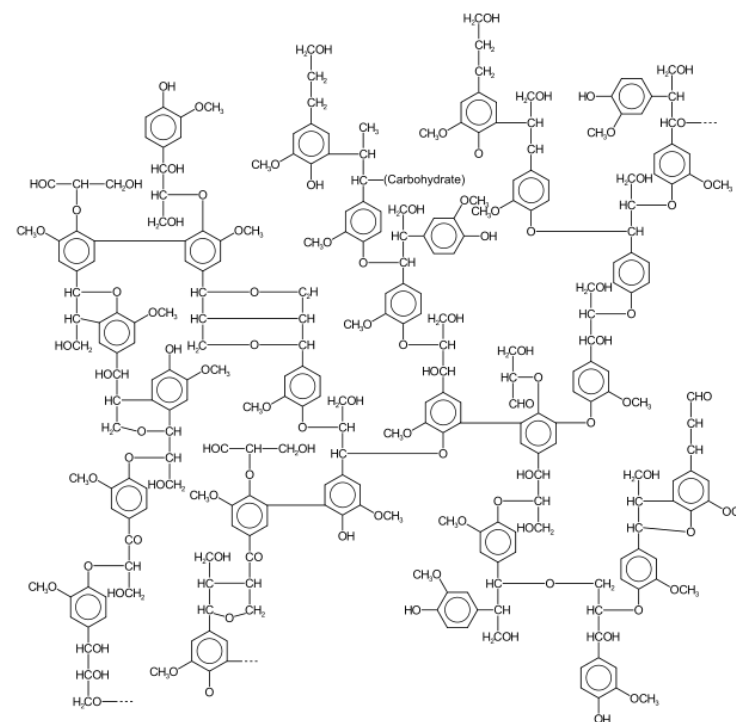
Figure 2. A suggested structure of lignin (Wikipedia contributors, 2016b)
