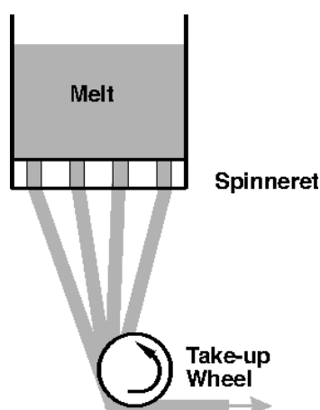
Figure 6. A Schematic image of melt spinning process
