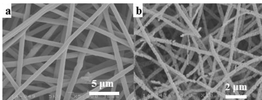
Figure 18. SEM image of (a) E-SL-CF and (b)E-SL-ACF-180
