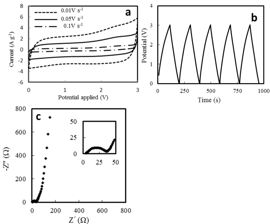
Figure 30. Electrochemical characterization of EDLC E-PEGL-ACF-180 . a) Cyclic voltammograms at different scan rates, b) GCD profile, and c) Nyquist plot (The inset is a magnification of the high-frequency region).
