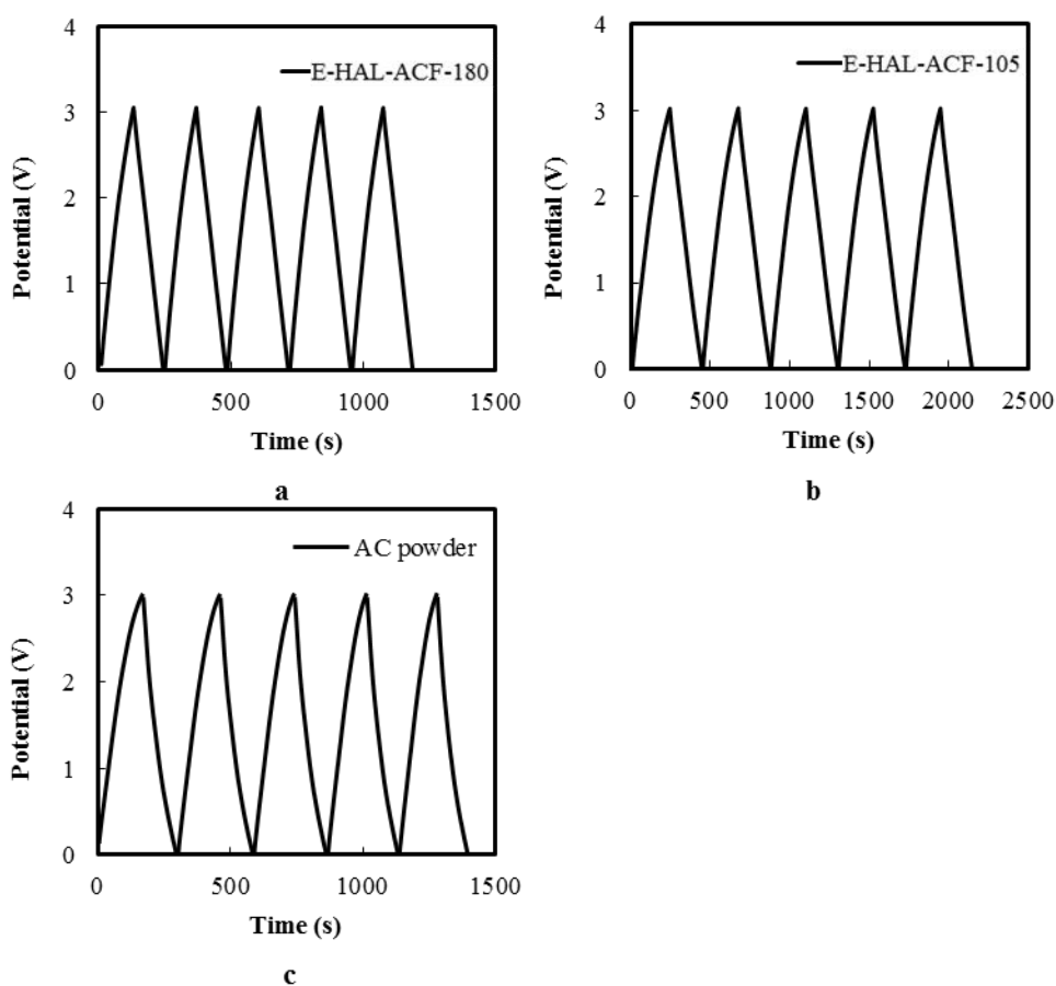
Figure 26. GCD profiles of a) EDLC E-HAL-ACF-180 , b) EDLC E-HAL-ACF-105 and c) EDLC AC powder under a current density of 1 A g -1
