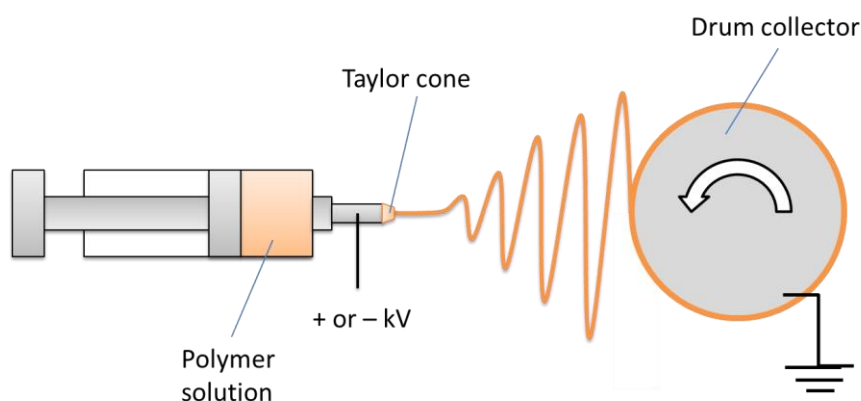
Figure 5. Diagram of fibers formation by electrospinning
