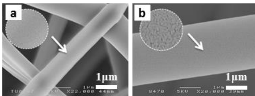
Figure 14. Magnified SEM images of CF derived from a) a single solvent system and b) a binary solvent system (E-HAL-CF)
