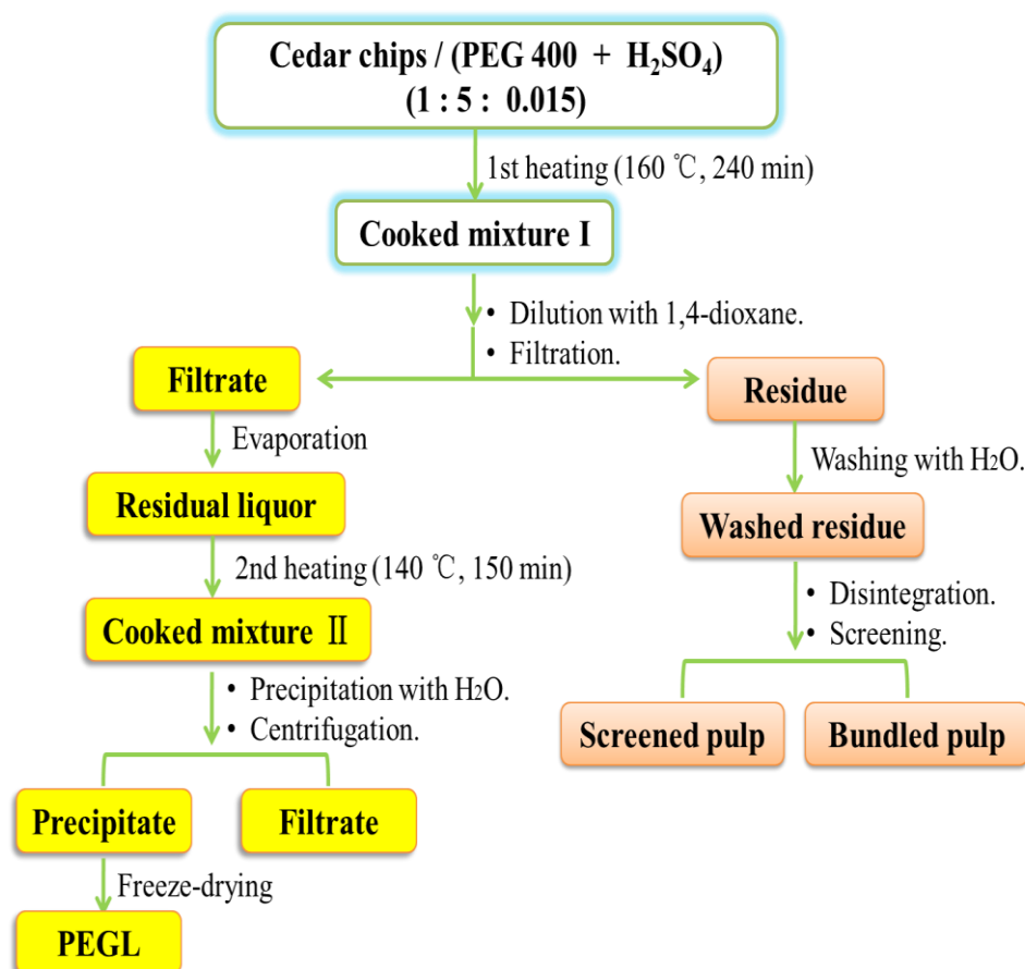
Figure 10. Experimental Scheme for preparation of PEGL
