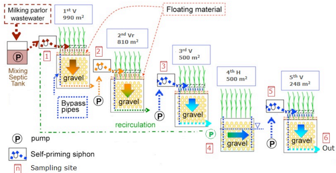
Fig. 2-4 Schematic diagram of Dairy-G hybrid system.
