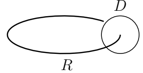
Figure 1: Infinitesimally thin ring R .
