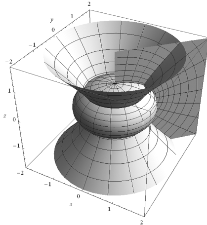
Figure 2: The coordinate surfaces for the oblate spheroidal coordinates.
