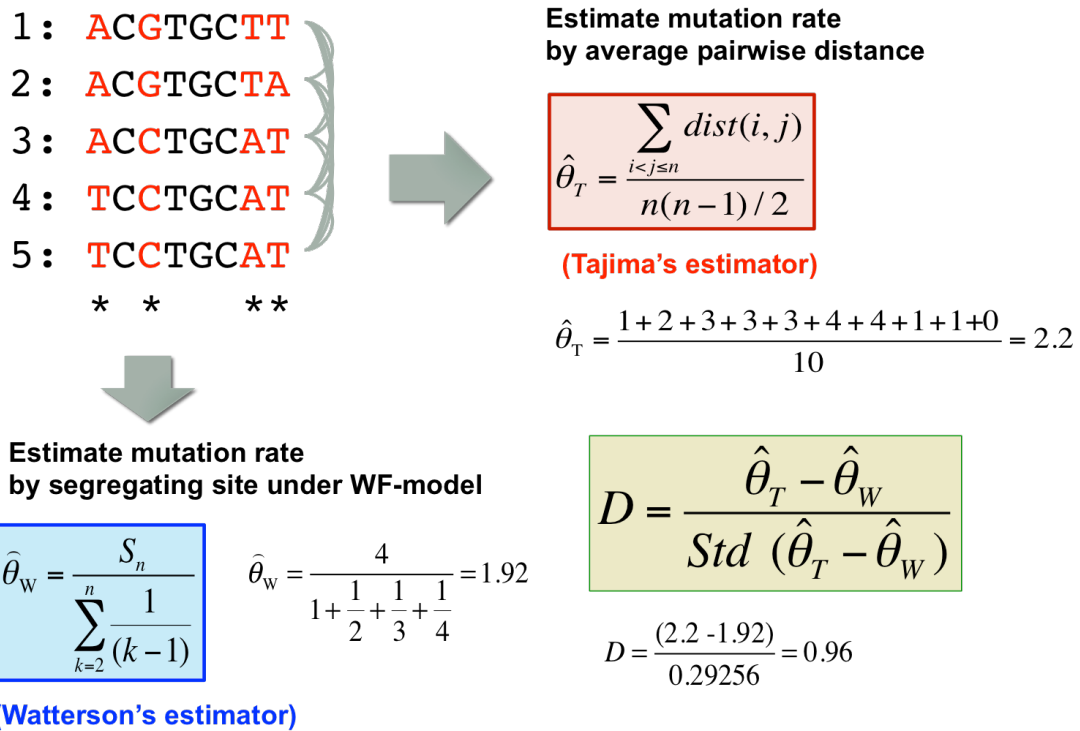
Figure 1. Simple example of calculation of Tajima's estimator, Watterson's estimator, and Tajima's D
