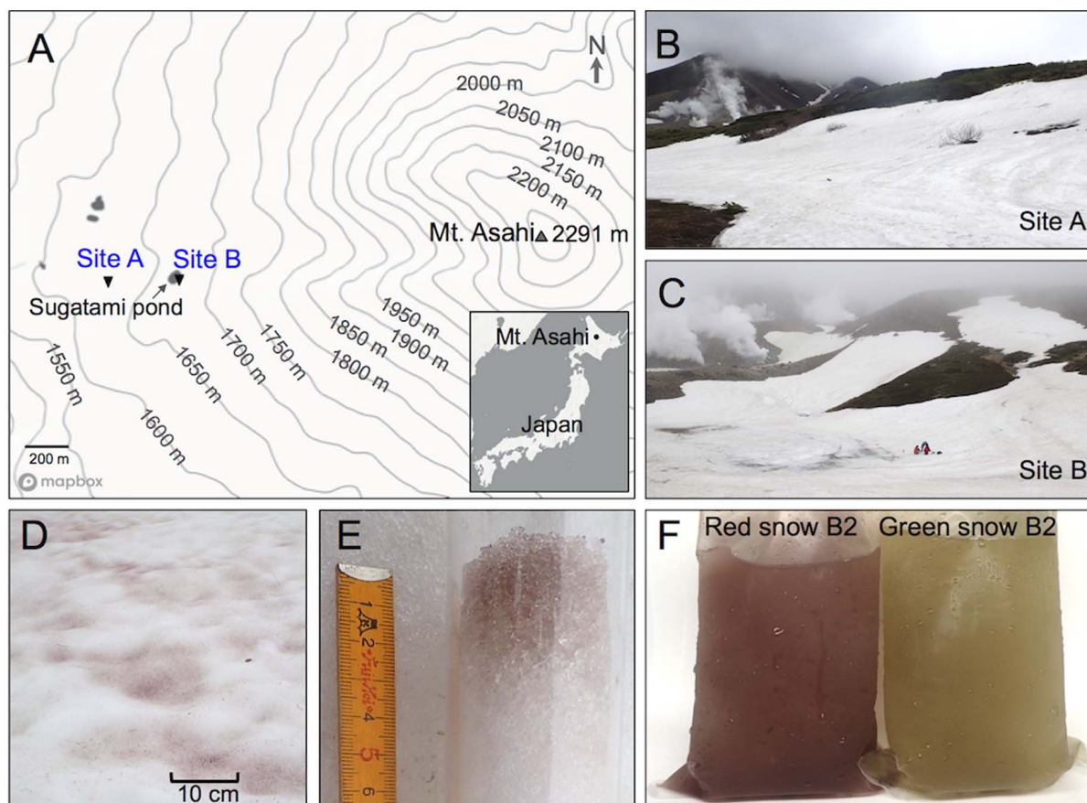
FIGURE 1 | (A) Sampling sites of Mount Asahidake. (B) Sampling site A snowfield. (C) Sampling site B snowfield. (D) Red snow surface of sampling site A snowfield. (E) Removing a core from the snow (sample red snow B2) shows coloration from the algae in the top 3 cm of the snow. (F) Melted green and red snow samples from B2 sampling. (Map generated by © Mapbox, © OpenStreetMap, modified and annotated).
