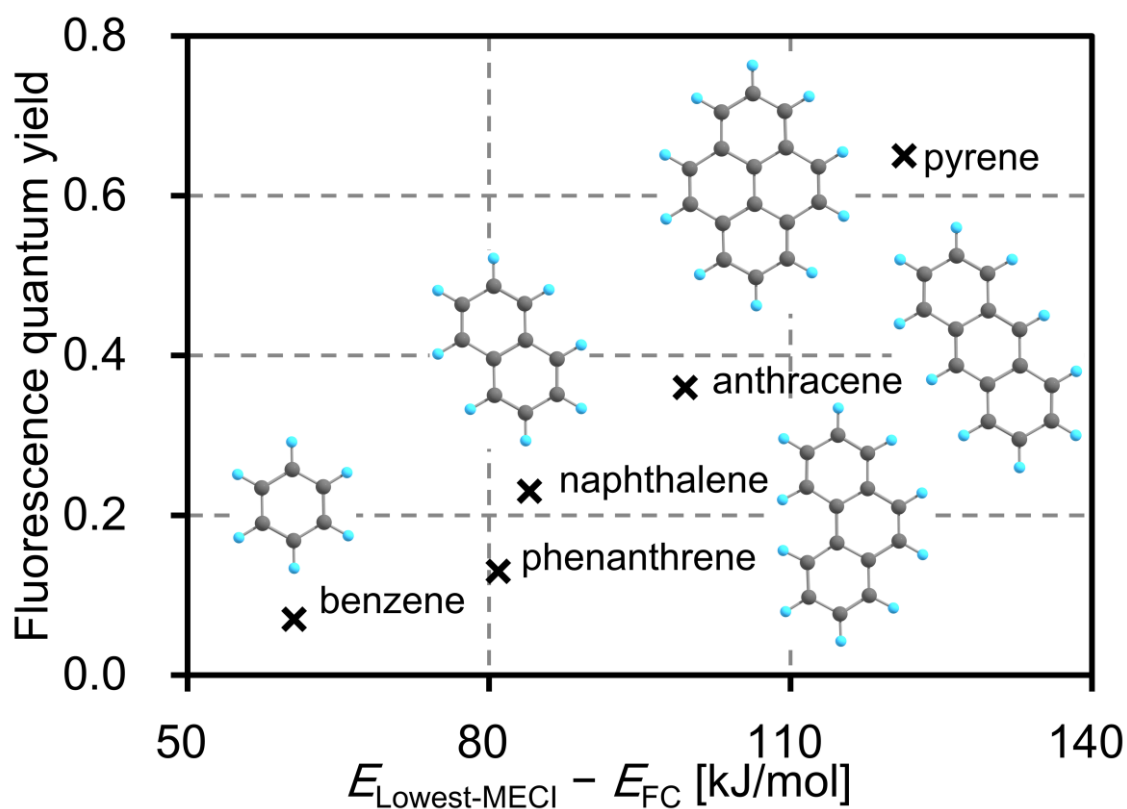
Fig. 9. The correlation between the fluorescence quantum yields measured in cyclohexane, 121 and the energy difference, E_{\text{Lowest-MECI}} - E_{\text{FC}} (cross marks). Each PAH is indicated with the structure and name of the PAH. Reproduced from Ref. 74 with permission from the Royal Society of Chemistry.
