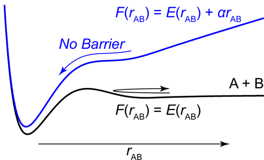
Fig. 1. A diatomic potential curve E(r_{AB}) between atoms A and B (see the black curve) and the corresponding AFIR function E(r_{AB}) + \alpha r_{AB} (see the blue curve). r_{AB} is the distance between A and B, and \alpha is a constant parameter.
