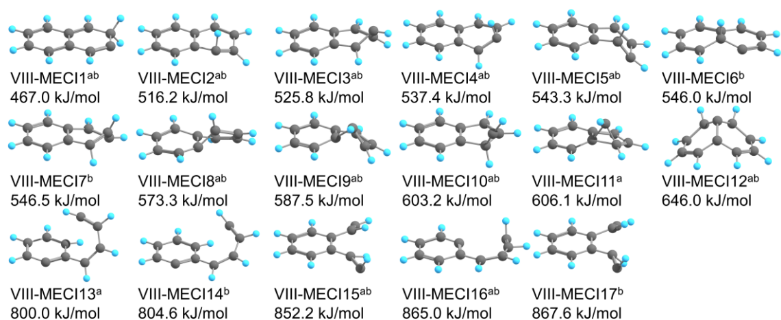
Fig. 8. Minimum energy conical intersection (MECI) structures of naphthalene between its singlet first excited electronic state ( S_1 ) and the singlet ground electronic state ( S_0 ), obtained by the SMF/SC-AFIR search starting from the Franck-Condon (FC) geometry. Electronic energy relative to the S_0 energy of the FC point are shown. The energy gap between the two target states are smaller than 0.1 kJ/mol, and only single value is shown. Structures obtained by the searches with \gamma = 100 and 200 kJ/mol, respectively, are indicated by a and b.
