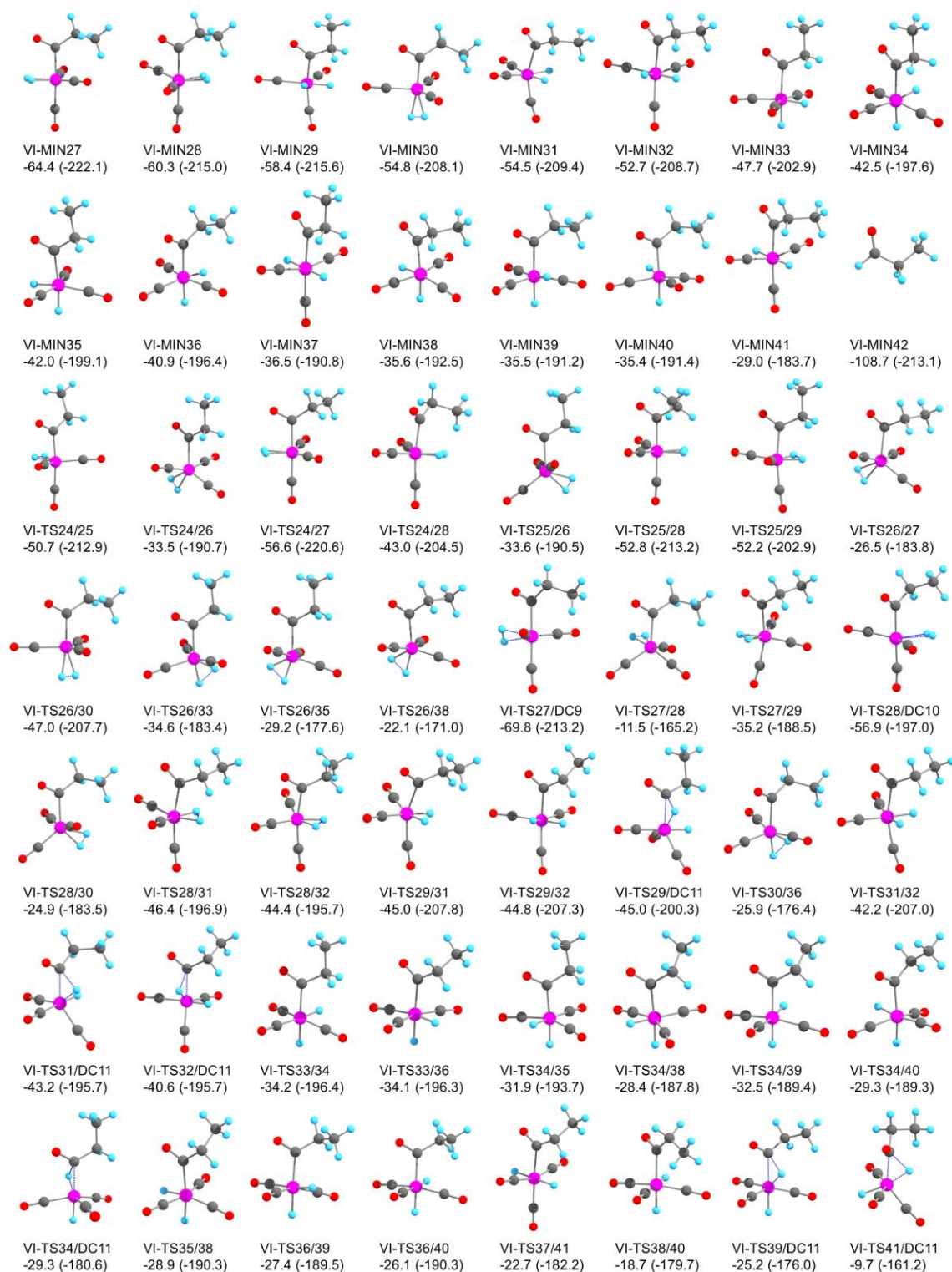
Fig. 6. Reaction pathways obtained by MC- and SC-AFIR for the last part of Co-catalyzed hydroformylation. TS x/y is a transition state connecting MIN x and MIN y
