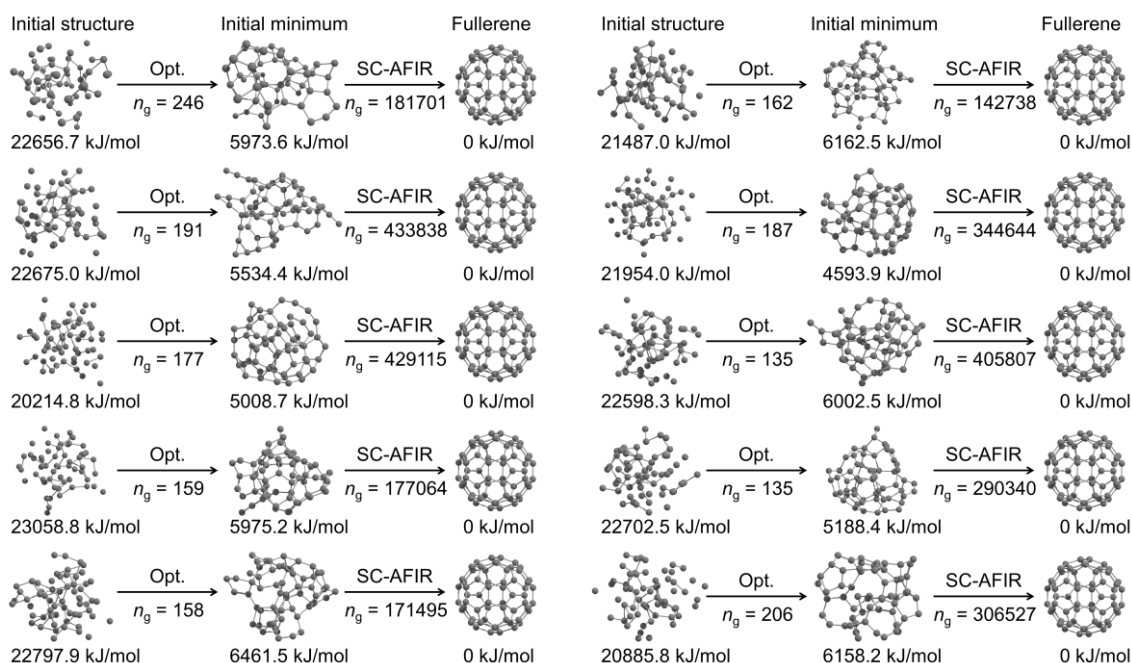
Fig. 7. Initial random structure, initial local minimum structure obtained by optimization of the random structure, and the final structure seen in the 10 independent stochastic SC-AFIR searches. The number of gradients computed in each step n_g is shown below arrows. Electronic energy relative to Buckminsterfullerene is shown below each structure.
