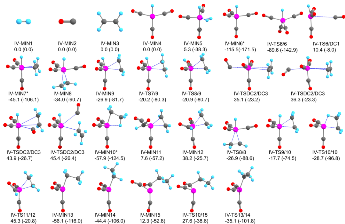
Fig. 4. Reaction pathways obtained by MC- and SC-AFIR for the initial part of Co-catalyzed hydroformylation. TS x/y is a transition state connecting MIN x and MIN y in this figure. Gibbs free energy and electronic energy in parentheses relative to separately optimized reactants are shown in kJ/mol. DC stands for dissociation channel: DC1 is HCo(CO) 3 + CO at 0.0 (0.0) kJ/mol, DC2 is MIN7 + CO at -45.1 (-106.1) kJ/mol, and DC3 is MIN6 + C 2 H 4 at -115.5 (-171.5) kJ/mol.
