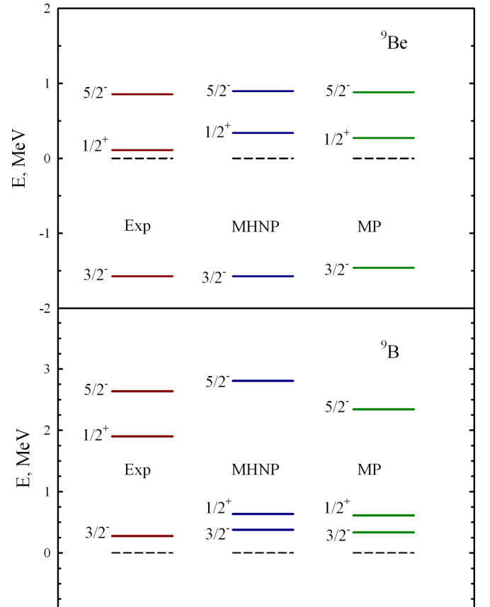
FIG. 4. Comparison of some resonance states in {}^9\text{Be} and {}^9\text{B} calculated with the MHNP and MP potentials and with experimental data.
