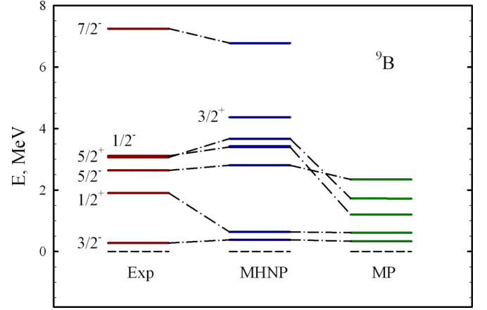
FIG. 3. Experimental and calculated spectra of {}^9\text{B} .
