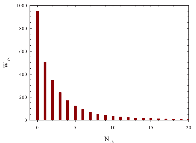
FIG. 12. Structure of the wave function of the 5/2^- resonance state in {}^9\text{B} . The result is obtained with the MHNP.
