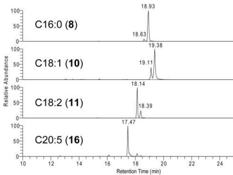
Figure 4. Positional preferences of C16:0 ( 8 ), C18:1 ( 10 ), C18:2 ( 11 ) and C20:5 ( 16 )
