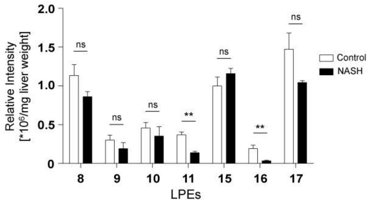
Figure 5. Comparison of NASH and control liver tissues. C18:3 (12-14) were excluded for clarity. N = 5, ns: not significant, **: P < 0.01
