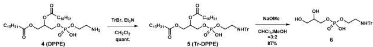
Scheme 1. Synthesis of common intermediate 6
