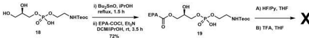
Scheme 3. Protecting the amino functionality with a Teoc group
