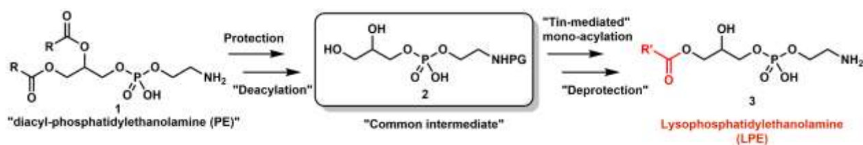
Figure 2. Synthetic strategy towards LPEs in this study; R, R' = fatty acid chains ; PG = protecting group
