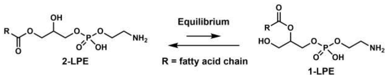
Figure 1. 1,2- O -acyl migration in LPEs
