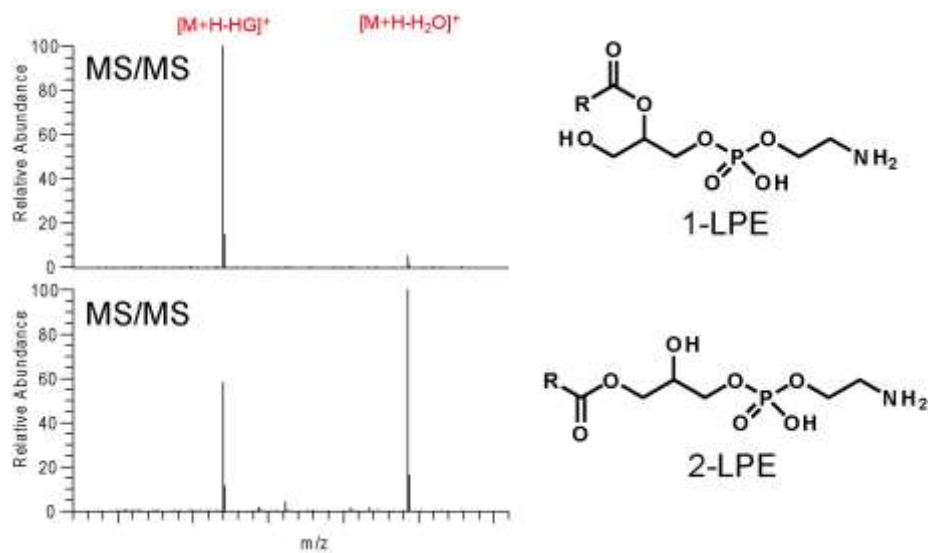
Figure 3. Representative product ion pattern for 1- (top) and 2-LPEs (bottom).
