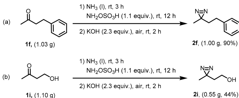
Scheme 4. Gram-scale synthesis of 2f (a) and 2i (b).
