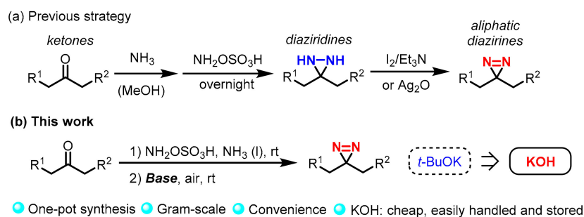
Scheme 1. Previous (a) and base-mediated one-pot (b) synthesis of aliphatic diazirines.
