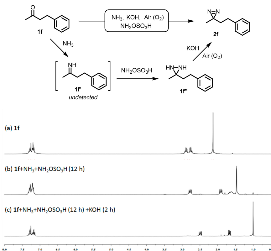
Scheme 3. One-pot synthesis of aliphatic diazirine 2f . The reaction stages were monitored using ^1\text{H-NMR} with \text{CDCl}_3 . (a) starting material 1f ; (b) 1f was treated with \text{NH}_2\text{OSO}_3\text{H} in liquid ammonia for 12 h; (c) The residue was further treated with KOH in liquid ammonia under air for 2 h.
