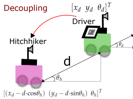
Figure 6. Decoupling process.
