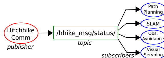
Figure 8. Simplified view of ROS topic (green), publisher (red) and subscriber (blue) nodes for module on/off.
