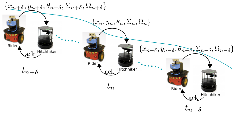
Figure 5. Intermittent information transfer from driver every \delta time-steps to recover from ‘driver-lost’ scenario.
