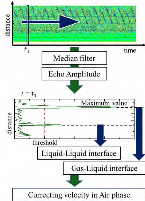
FIGURE 9. Flow chart of UVP-data processing with interface detection to classify the domain into gas, oil, and water phases.
