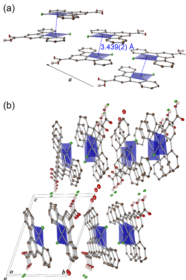
Fig. 2. (a) Stacking and (b) packing structures of (a) [1\text{H}]\text{Cl} \cdot \text{H}_2\text{O} . The coordination plane of the Pt(II) ion is shown in blue. The blue, green, brown, light-blue, and red ellipsoids represent Pt, Cl, C, N, and O atoms, respectively. The H atoms bonded to the O atoms of the carboxy groups are shown as pink balls, and the others are omitted for clarity. Displacement parameters are drawn at a 50% probability level.
