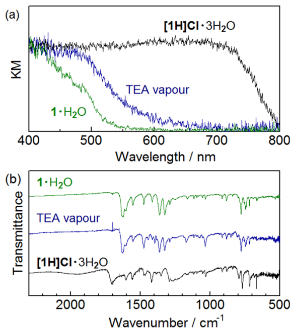
Fig. 7. Changes in the (a) UV-vis diffuse reflectance and (b) IR spectra of [\text{1H}]\text{Cl} \cdot 3\text{H}_2\text{O} (black) upon exposure to basic triethylamine (TEA) vapor at room temperature. The green line in each panel shows the spectrum of 1 \cdot \text{H}_2\text{O} .
