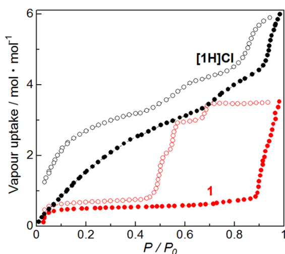
Fig. 5. Water-vapour isotherms of 1 (red) and [\text{1H}]\text{Cl} (black) at 298 K. Closed and open symbols indicate adsorption and desorption, respectively.
