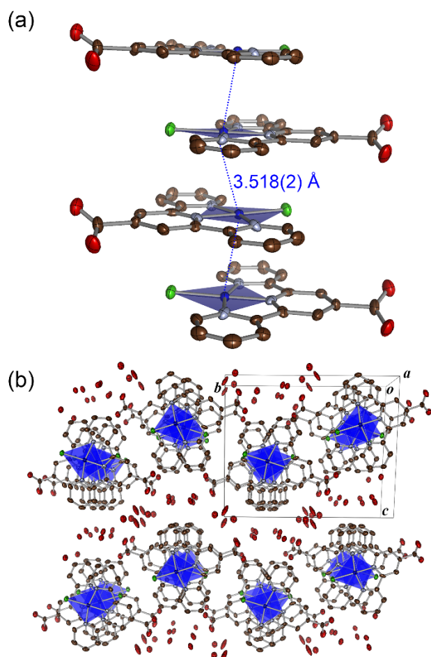
Fig. 1. (a) One-dimensional stacking and (b) packing structures of 1 \cdot 3.5\text{H}_2\text{O} . The coordination plane of the Pt(II) ion is shown in blue. The blue, green, brown, light-blue, and red ellipsoids represent Pt, Cl, C, N, and O atoms, respectively. The H atoms are omitted for clarity. Displacement parameters are drawn at a 50% probability level.
