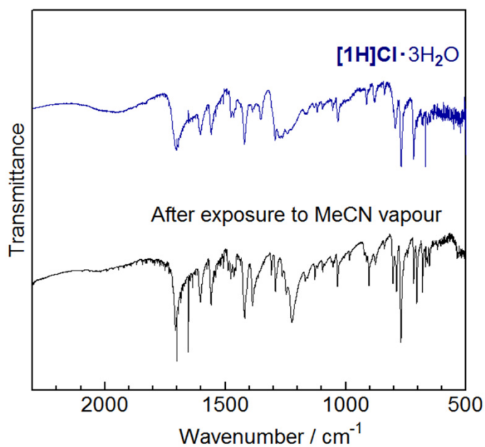
Figure S2. IR spectra of [1\text{H}]\text{Cl} \cdot 3\text{H}_2\text{O} before and after exposure to MeCN vapour for 3 days at room temperature.
