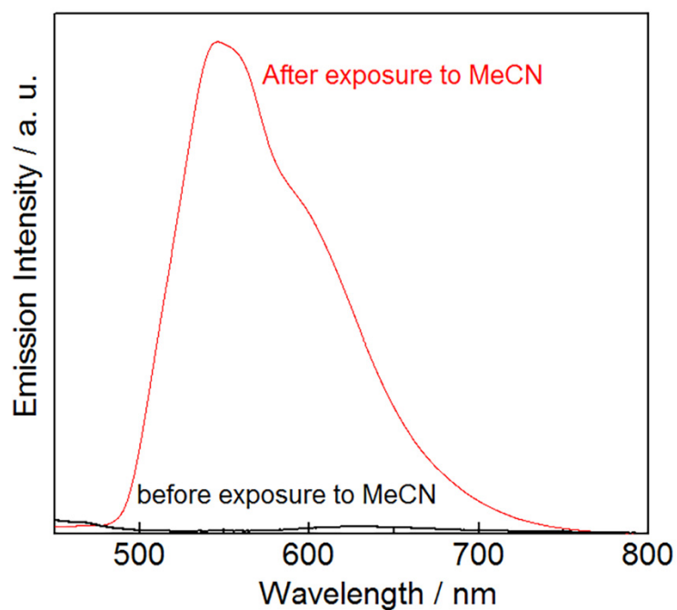
Figure S5. Change of luminescence spectrum of [1\text{H}]\text{Cl}\cdot 3\text{H}_2\text{O} before (black) and after (red) exposure to MeCN vapour for 3 days at room temperature.
