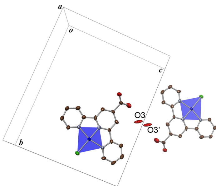
Figure S1. The positions of disordered water molecules between the adjacent two complex molecules in 1 \cdot 3.5\text{H}_2\text{O} .
