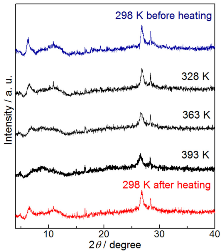
Figure S9. Temperature-dependence of PXRD pattern of [1H]Cl \cdot 3H_2O .
