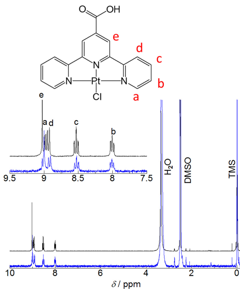
Figure S4. ^1\text{H} NMR spectra (DMSO- d_6 ) of as-synthesized [1H]Cl ·3H 2 O (blue) and after exposure to MeCN vapour for 3 days at room temperature (black). The inset shows the magnification of the aromatic region from 7.5 to 9.5 ppm. The signal of OH proton of carboxylic acid group was not observed probably due to the rapid exchange with protons of water molecules.
