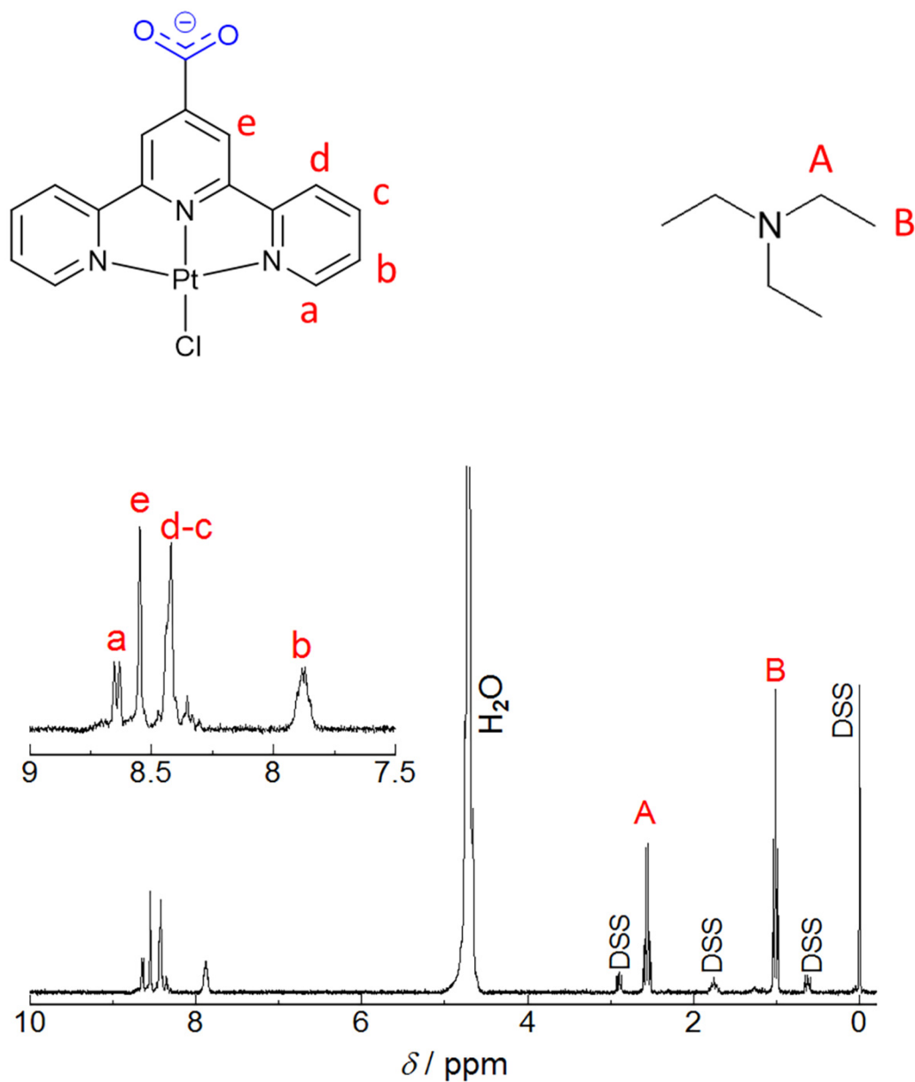
Figure S12. ^1\text{H} NMR spectrum of [1H]Cl ·3H 2 O after exposing it to triethylamine vapour (4%ND 3 in D 2 O). The inset shows the magnification of the aromatic region from 7.5 to 9.0 ppm. The ratio of integral intensities of the signals B to b is 9 : 2, indicating the formation of the equimolar amount of the complex 1 and [TEA-H] + Cl - .
