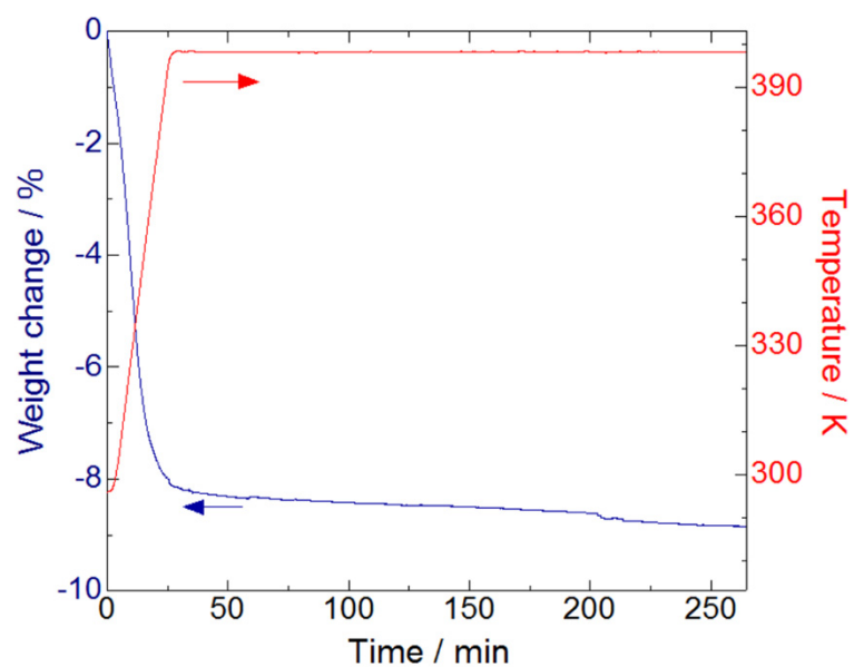
Figure S3. Thermogravimetric analysis for [1\text{H}]\text{Cl}\cdot 3\text{H}_2\text{O} in \text{N}_2 atmosphere. Observed weight loss (8.8 % at 250 min heating) is quantitatively agreed with the amount of the three hydrated water molecules (9.0 %) in the [1\text{H}]\text{Cl}\cdot 3\text{H}_2\text{O} .
