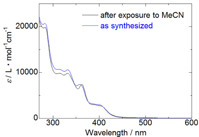
Figure S6. UV-Vis absorption spectra in DMSO of as-synthesized [1\text{H}]\text{Cl}\cdot 3\text{H}_2\text{O} (blue) and after exposure to MeCN vapour for 3 days at room temperature (black).
