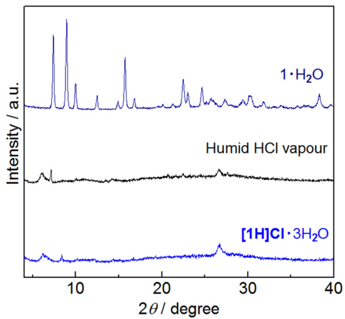
Figure S11. Changes of PXRD pattern of 1 \cdot \text{H}_2\text{O} by exposing it to humid HCl vapour for 3 days at 30 °C. The bottom blue line shows the PXRD pattern of [\text{1H}]\text{Cl} \cdot 3\text{H}_2\text{O} .
