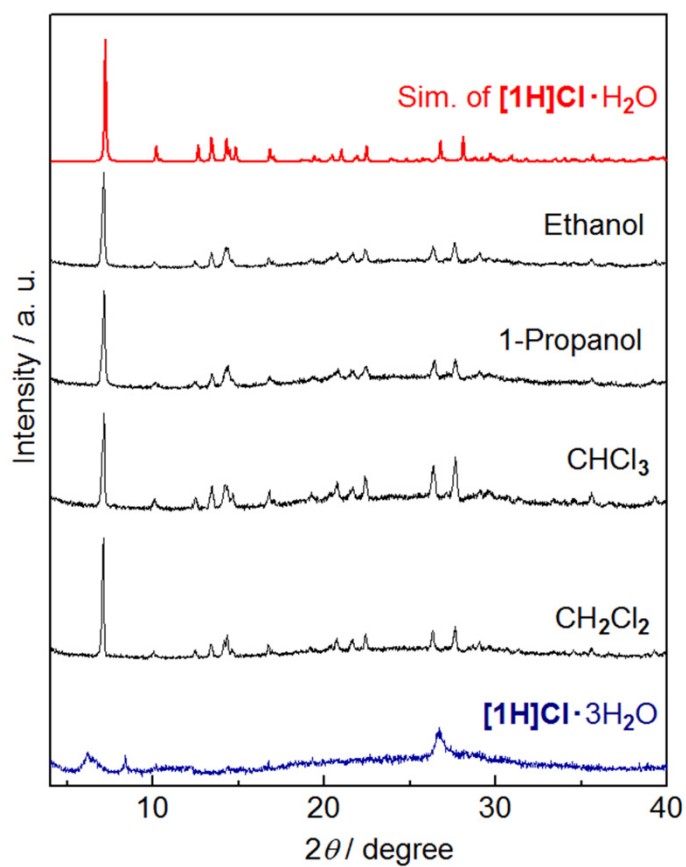
Figure S7. Changes of PXRD pattern of [1H]Cl \cdot 3H_2O under exposing to various organic solvent vapours for 3 days at 30 °C. The top red line shows the simulation pattern calculated from the crystal structure of the protonated monohydrate [1H]Cl \cdot H_2O .
