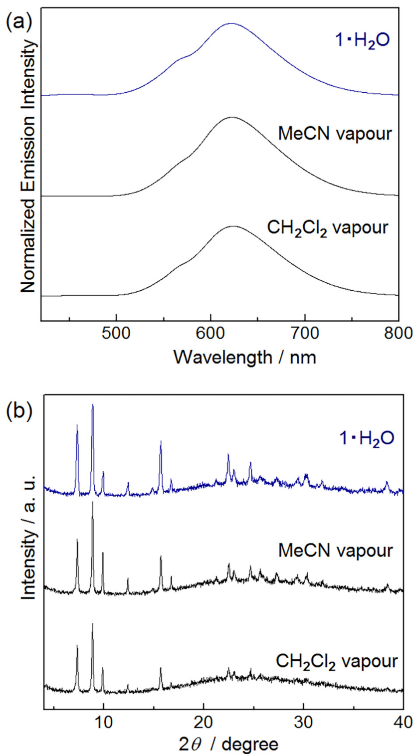
Figure S10. Changes of (a) luminescence spectrum and (b) PXRD pattern of 1 \cdot \text{H}_2\text{O} by exposing it to MeCN or \text{CH}_2\text{Cl}_2 vapour for 3 days at 30 °C.
