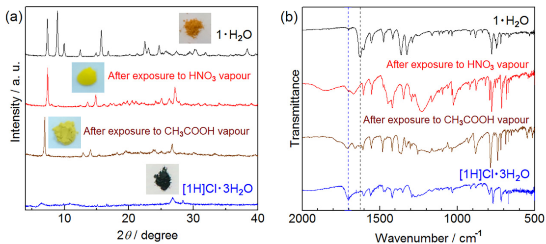
Figure S13. Changes of (a) PXRD pattern and (b) IR spectrum of 1 \cdot \text{H}_2\text{O} under exposure to humid \text{HNO}_3 or \text{CH}_3\text{COOH} vapour at room temperature. The bottom blues lines show the pattern and spectrum of the dark-blue protonated form [\text{1H}]\text{Cl} \cdot 3\text{H}_2\text{O} . The blue and black dotted lines in (b) indicate the positions of the \nu(\text{C}=\text{O}) modes of carboxy groups of protonated [\text{1H}]\text{Cl} \cdot 3\text{H}_2\text{O} and deprotonated 1 \cdot \text{H}_2\text{O} , respectively.
