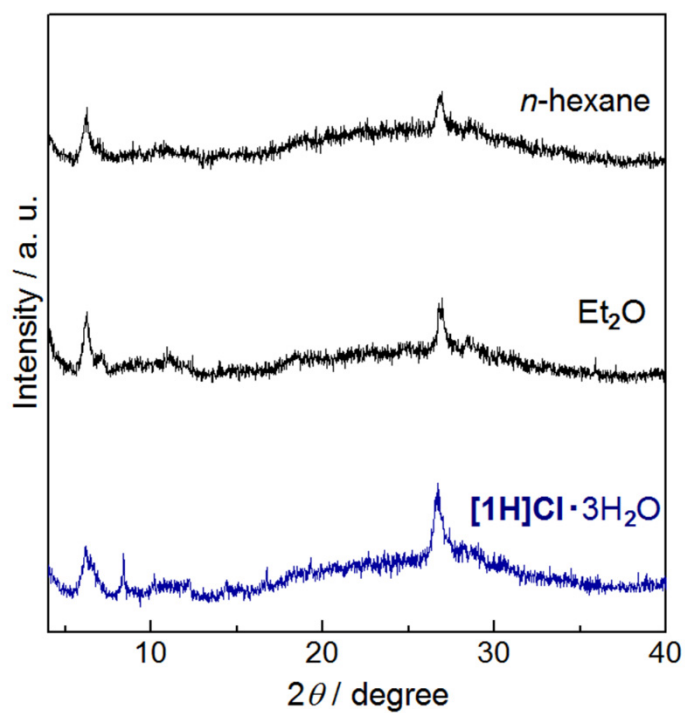
Figure S8. Changes of PXRD pattern of [\text{1H}]\text{Cl} \cdot 3\text{H}_2\text{O} after exposure to \text{Et}_2\text{O} or hexane vapour for 3 days at 30 °C.
