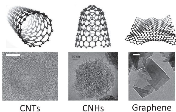
Fig. 1 Schematic models and TEM observation of carbon nanomaterials.
