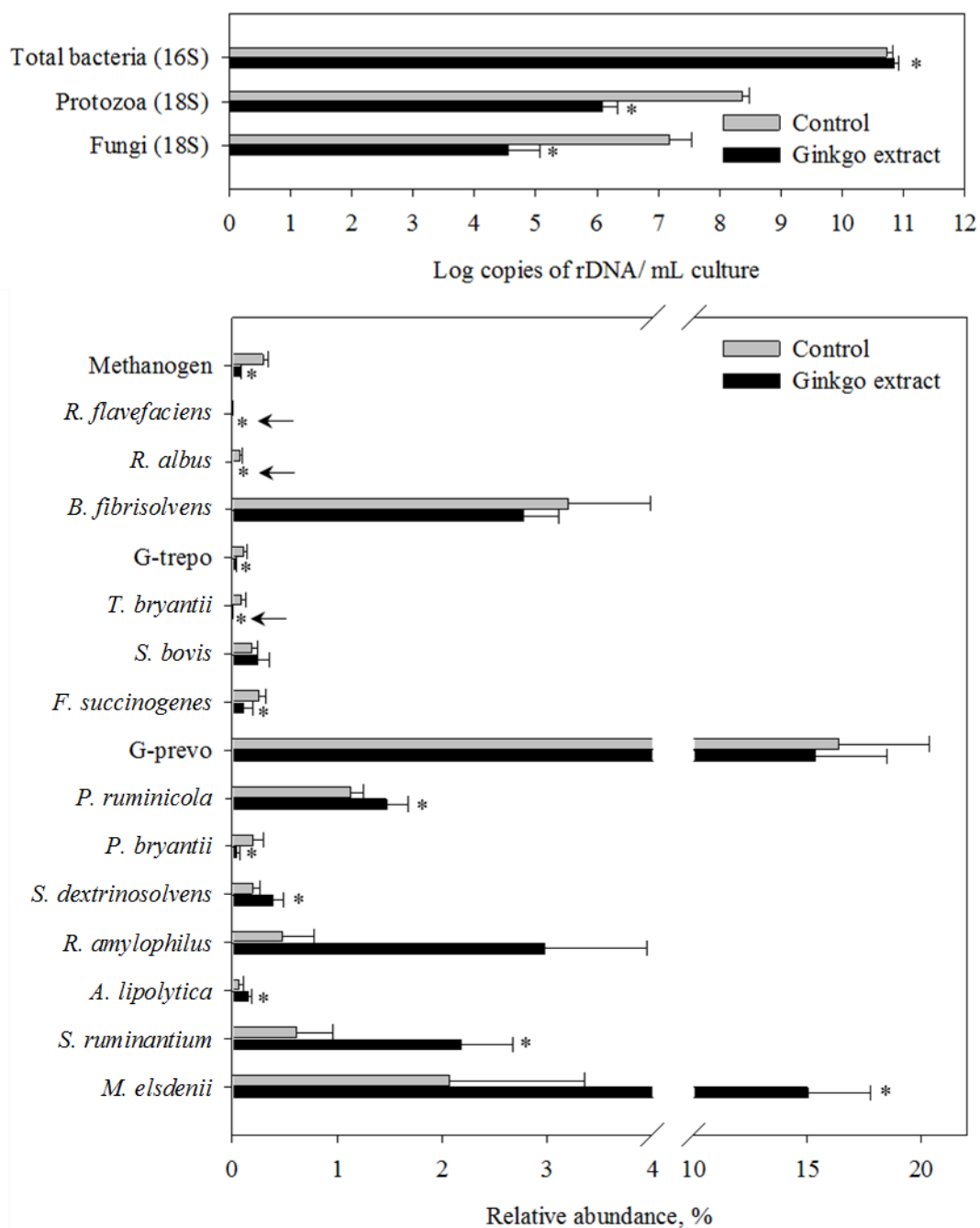
Figure 1. Relative abundance of rumen representative bacterial species and groups in RUSITEC (rumen simulation technique). Ginkgo extract was supplemented at 1.6% in fruit equivalent. G-trepo = genus Treponema , G-prevo = genus Prevotella ; species include Ruminococcus flavefaciens , Ruminococcus albus , Butyrivibrio fibrisolvens , Treponema bryantii , Streptococcus bovis ,
