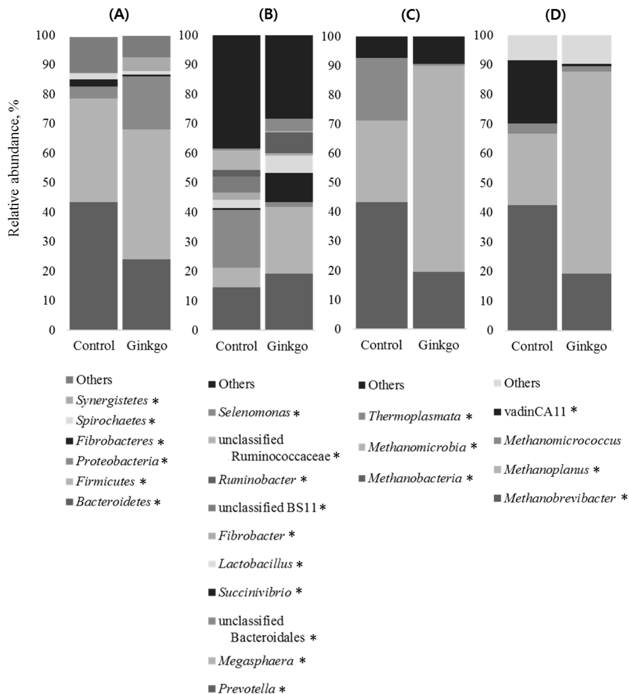
Figure 2. Effect of ginkgo extract supplementation on rumen microbiota in RUSITEC (rumen simulation technique) evaluated by MiSeq (Illumina Inc., San Diego, CA) at bacterial phylum level (A), at bacterial genus level (B), at archaeal class level (C), and at archaeal genus level (D). Asterisk (*) indicates statistical significance between control and treatment ( P < 0.05 ).
