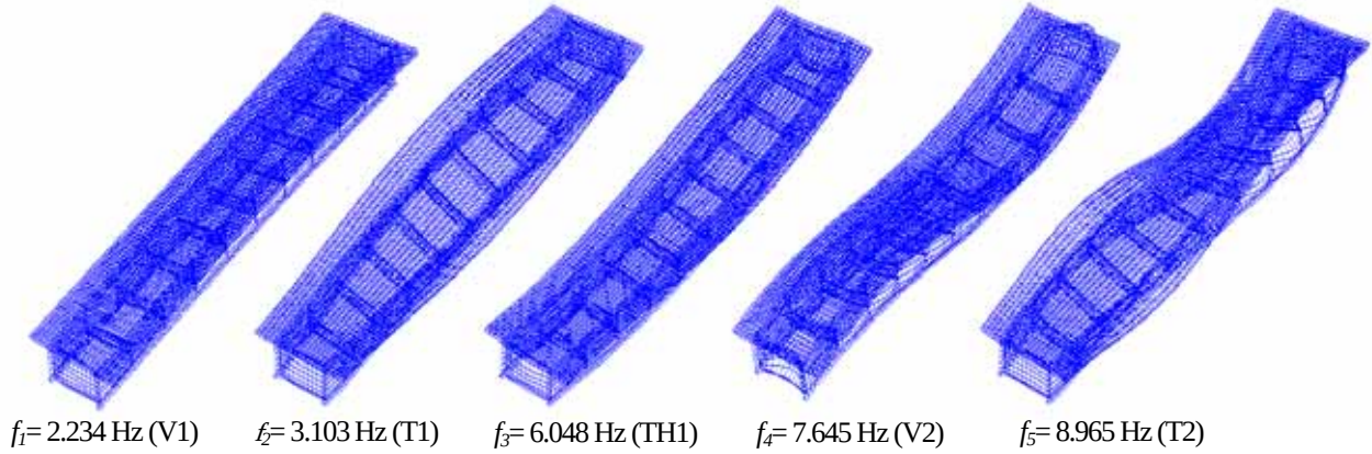
Fig.5 Several mode shapes of the studied bridge ( R = 400 m and e = 3\% )
