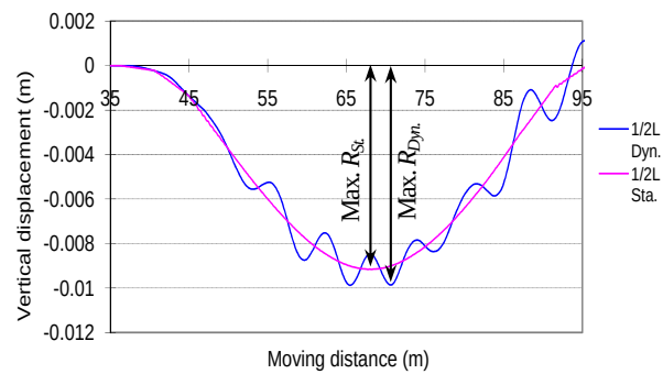
Fig.8 Mid-span deflection history
