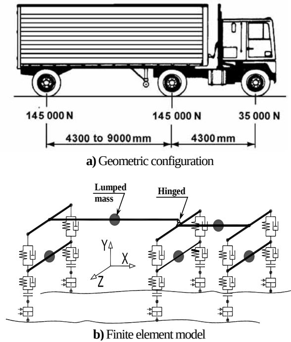
Fig. 3 HS20-44 design truck
