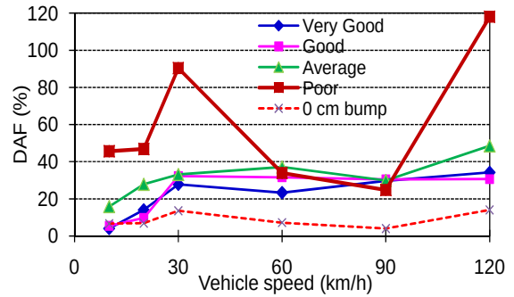
b) Different roughness classes at 4cm bump height
