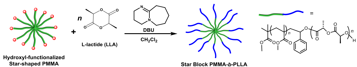
Figure 1.3. Synthesis of star block copolymers with arms consisting of blocks of PMMA and PLLA
