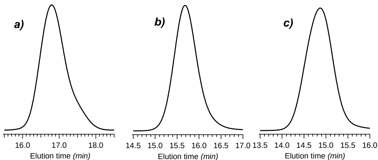
Figure 3.5. SEC traces of (a) (PMMA _{30} -OH) _3 (run 1) (b) (PMMA _{30} -OH) _6 (run 2) (c) (PMMA _{30} -OH) _{12} (run 3)
