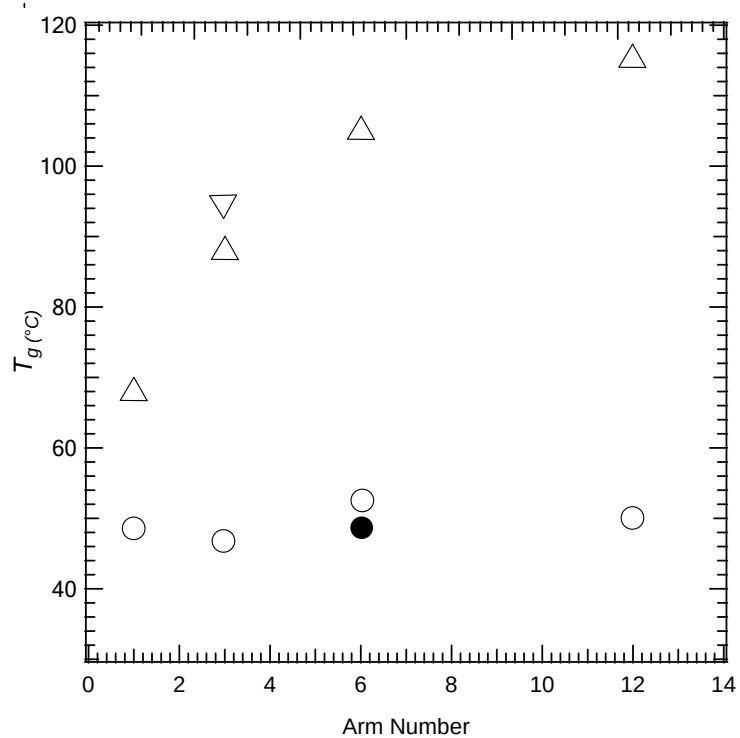
Figure 4.11 Relation between T_g versus arm numbers for core-first synthesized hydroxyl-functionalized PMMAs ( \Delta ), arm-first synthesized hydroxyl-functionalized PMMA ( \nabla ), linear and star block copolymers ( \circ ) and miktoarm star polymer ( \bullet ).
