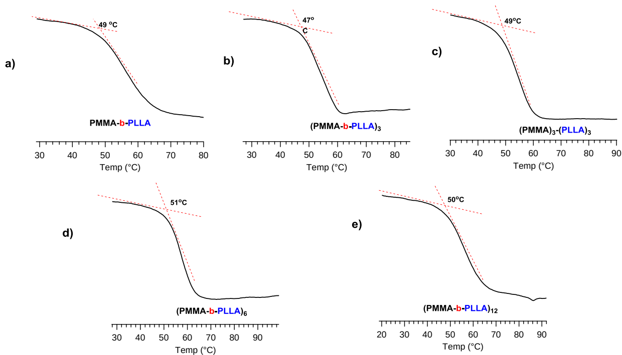
Figure 4.10 DSC thermograms of linear, star block copolymers and miktoarm star polymers.
