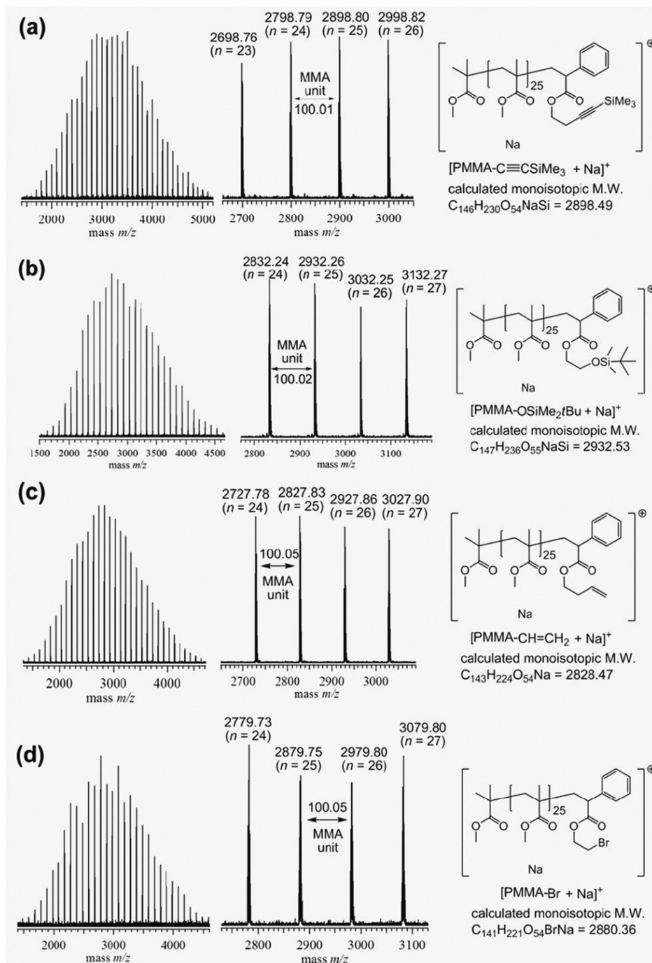
Figure.2.11. MALDI-TOF MS spectra of (a) PMMA-C \equiv CSiMe 3 (Run 26, M_{n,SEC} = 3460 ; M_w/M_n = 1.07 ), (b) PMMA-OSiMe 2 tBu (Run 27, M_{n,SEC} = 3250 ; M_w/M_n = 1.06 ), (c) PMMA-CH=CH 2 (Run 28, M_{n,SEC} = 3730 ; M_w/M_n = 1.07 ), and (d) PMMA-Br (Run 29, M_{n,SEC} = 3690 ; M_w/M_n = 1.07 ).
