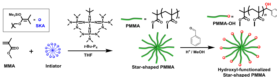
Figure 1.2 Star-shaped of PMMAs functionalized with hydroxyl groups by core-first t\text{-Bu-P}_4 catalyzed GTP
