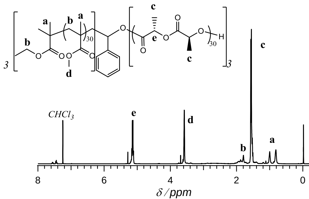
Figure 4.3 ^1\text{H} NMR spectrum of PMMA 3 -PLLA 3 miktoarm star polymer in \text{CDCl}_3 (400 MHz).
