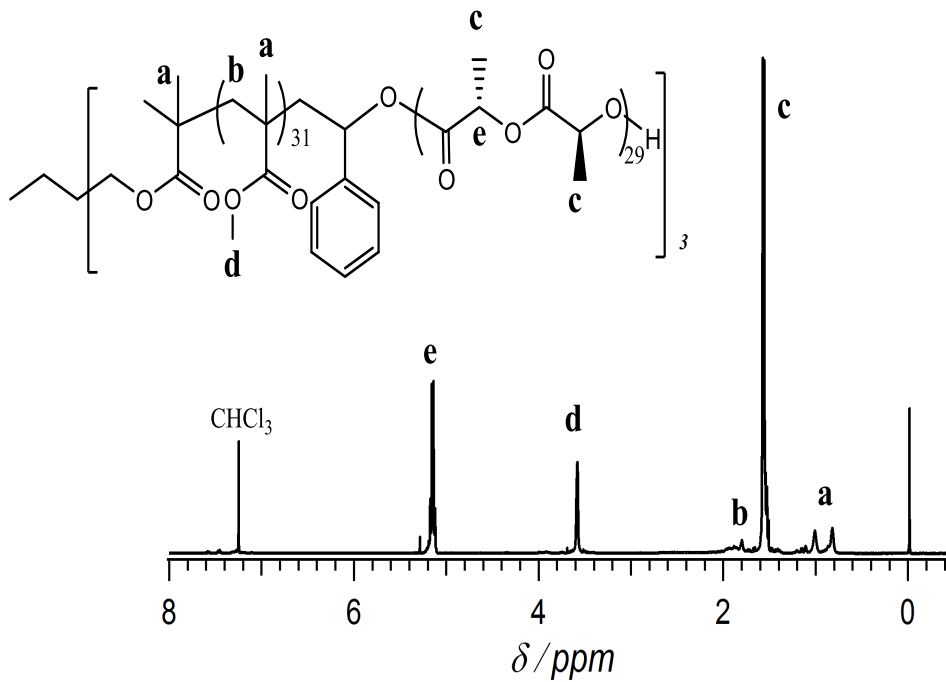
Figure 4.6 1 H NMR spectrum of (PMMA 31 - b -PLLA 29 ) 3 in CDCl 3 (400 MHz).
