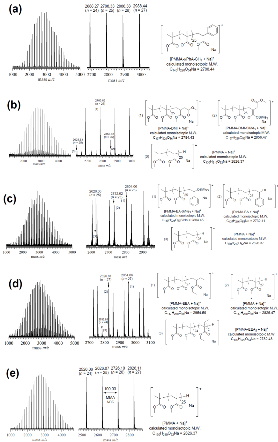
Figure 2.9. MALDI-TOF MS spectra of PMMAs terminated by (a) \alpha -PhA-Me, (b) DMI, (c) BA, (d) EEA, and (e) DMMAm.
