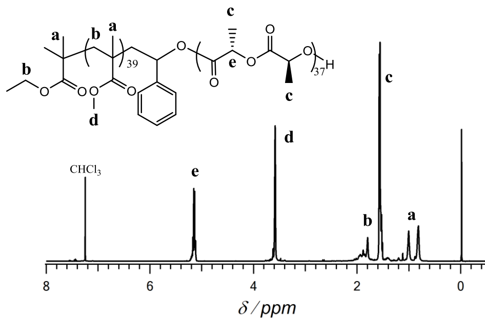
Figure 4.5 1 H NMR spectrum of PMMA 39 - b -PLLA 37 in CDCl 3 (400 MHz).
