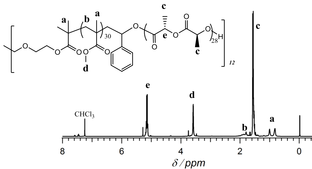
Figure 4.8 ^1\text{H} NMR spectrum of (\text{PMMA}_{30}\text{-}b\text{-PLLA}_{30})_{12} in \text{CDCl}_3 (400 MHz).
