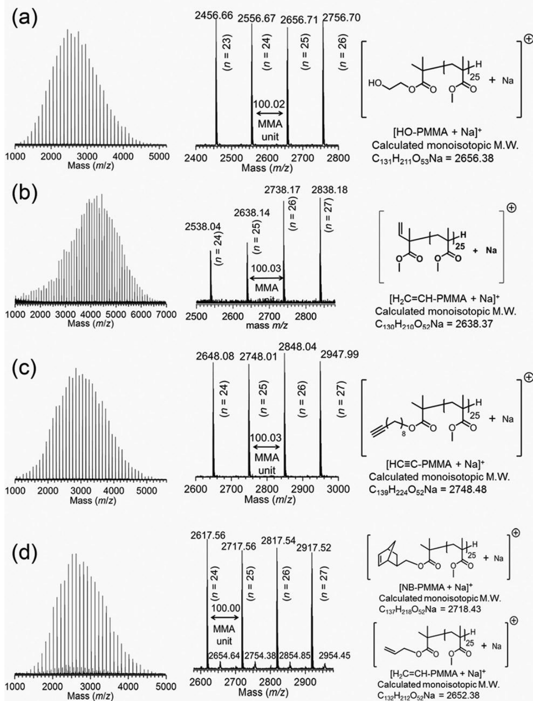
Figure. 2.8. MALDI-TOF MS spectra of (a) HO-PMMA (Run 1, M_{n,\text{SEC}} = 3300 \text{ g mol}^{-1} , M_w/M_n = 1.08 ), (b) \text{H}_2\text{C}=\text{CH} -PMMA, (Run 11, M_{n,\text{SEC}} = 4500 \text{ g mol}^{-1} , M_w/M_n = 1.08 ) (c) \text{HC}\equiv\text{C} -PMMA (Run 6, M_{n,\text{SEC}} = 3800 \text{ g mol}^{-1} , M_w/M_n = 1.07 ), and (d) NB-PMMA, (Run 16, M_{n,\text{SEC}} = 3400 \text{ g mol}^{-1} , M_w/M_n = 1.08 ).
