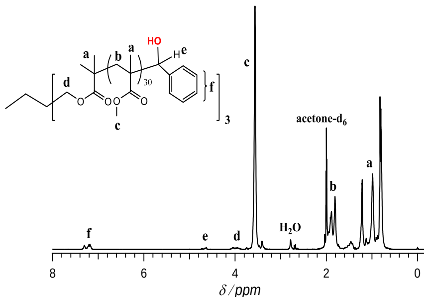
Figure 3.2. 1 H NMR spectrum of the hydroxyl end-functionalized 3-arm star-shaped PMMA in acetone- d 6 (400 MHz).
