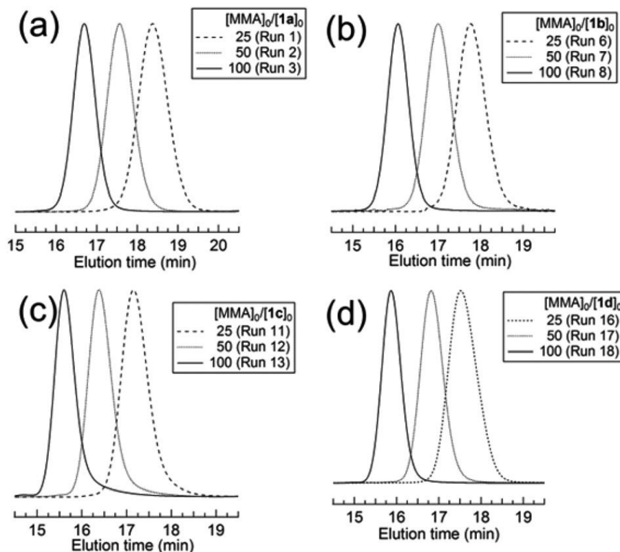
Figure 2.6. SEC traces of (a) HO-PMMA (Runs 1–3), (b) \text{HC}\equiv\text{C} -PMMA (Runs 6–8), (c) \text{H}_2\text{C}=\text{CH} -PMMA (Runs 11–13), and (d) NB-PMMA (Runs 16–18) synthesized by \text{Me}_3\text{SiNTf}_2 -catalyzed GTP.
