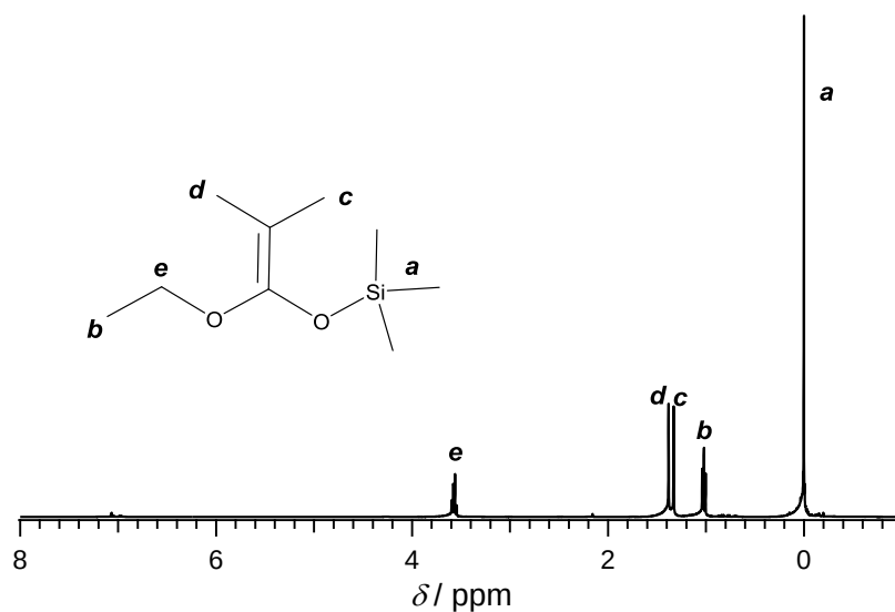
Figure 2.3. 1 H NMR spectra of 1-ethoxy-1-(trimethylsiloxy)-2-methylprop-1-ene (SKA Et ) in CDCl 3
