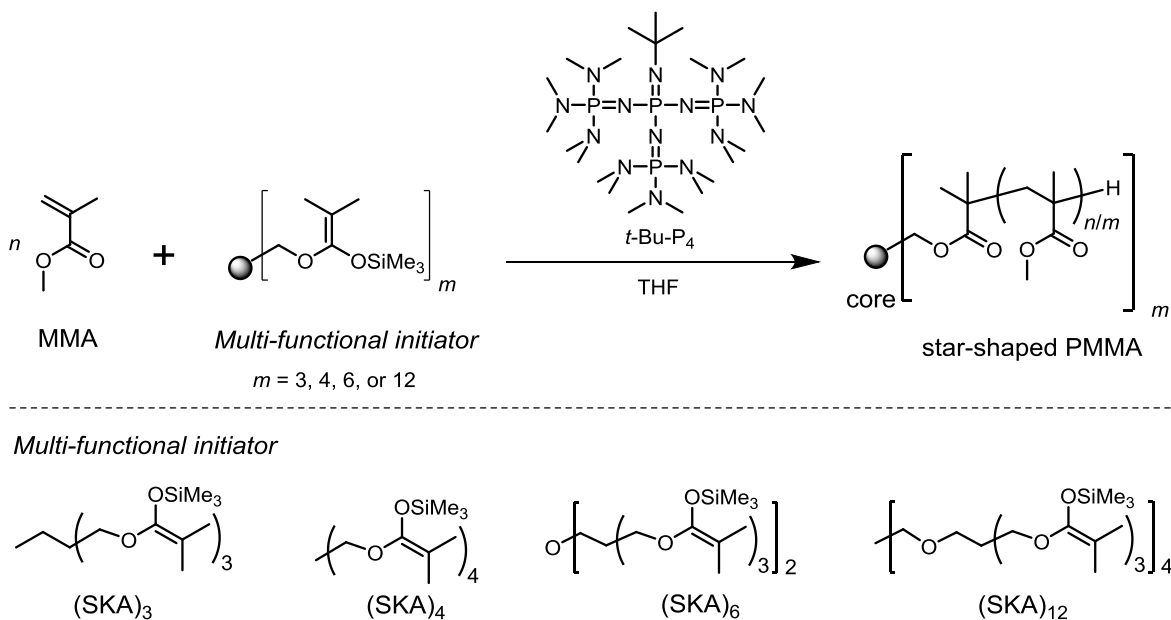
Scheme 1.7 Synthesis of star-shaped PMMA by GTP using multi-functional initiators
