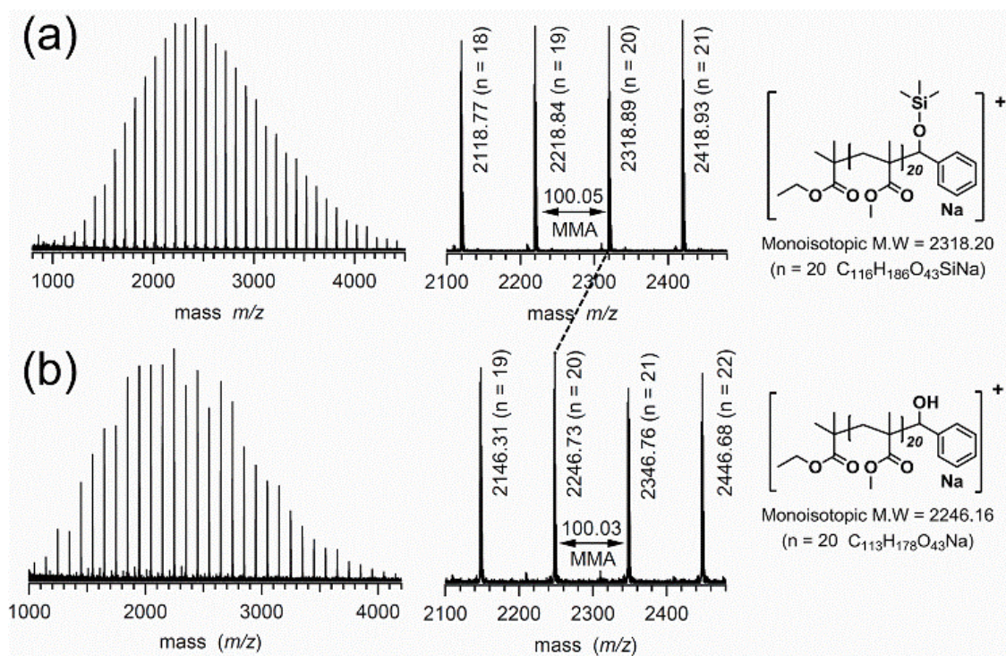
Figure 2.13. MALDI-TOF MS spectra in reflector mode of (a) PMMA-OSiMe 3 obtained from Run 35 and (b) PMMA-OH obtained from Run 35.
