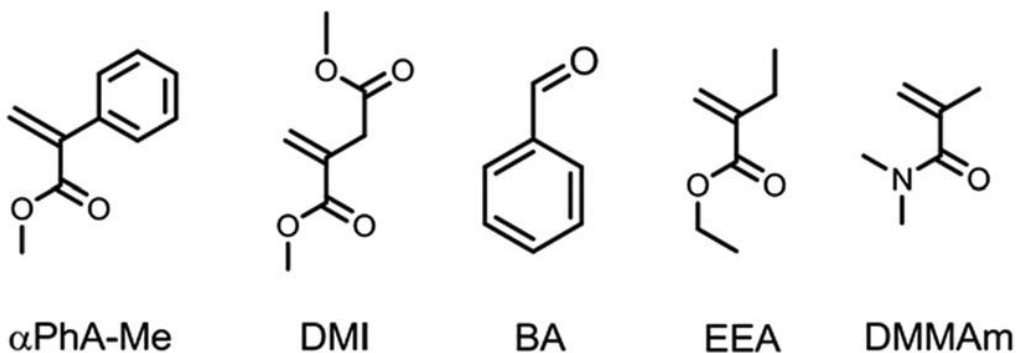
Scheme 2.6 Potential Terminators for \text{Me}_3\text{SiNTf}_2 -catalyzed GTP of MMA
