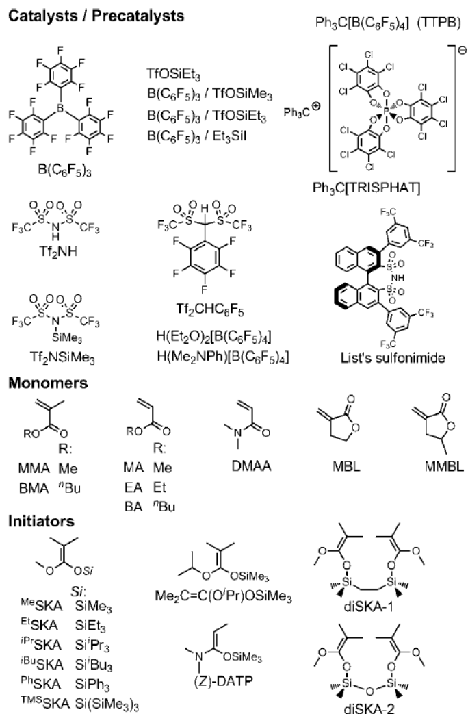
Scheme 1.3 Catalysts, monomers, and initiators employed in GTP catalyzed by Lewis acid organocatalysts.
