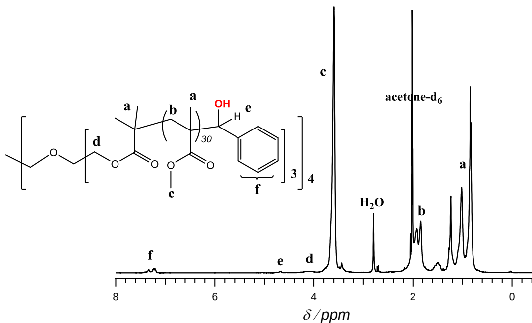
Figure 3.4. ^1\text{H} NMR spectrum of hydroxyl end-functionalized 12-arm star-shaped PMMA in acetone- d_6 (400 MHz).
