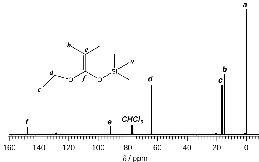
Figure 2.4. 13 C NMR spectra of 1-ethoxy-1-(trimethylsiloxy)-2-methylprop-1-ene (SKA Et ) in CDCl 3
