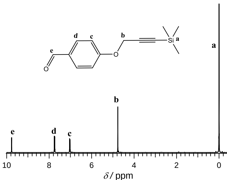
Figure 2.5. ^1\text{H} NMR spectrum of 4-(3-(Trimethylsilyl)prop-2-ynoxy)benzaldehyde terminator in Acetone- d_6 (400 MHz)
