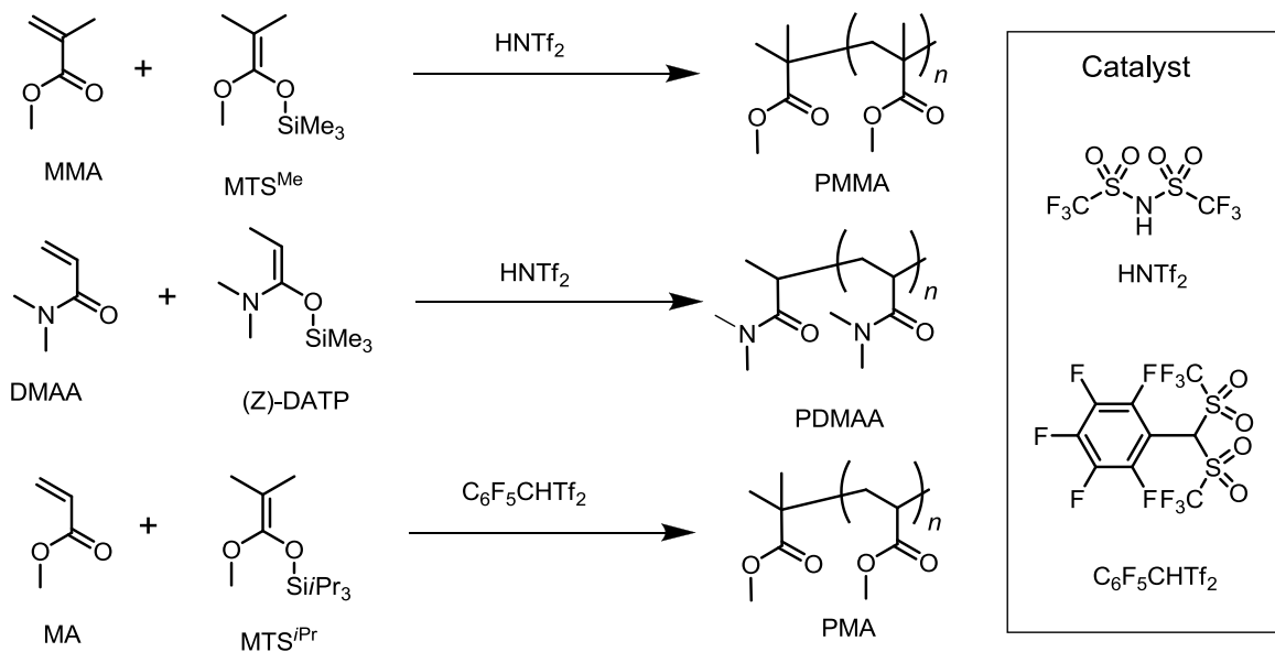
Scheme 1.5 Organoacid catalyzed-GTP of MMA, MA, and DMAA using designed initiators
