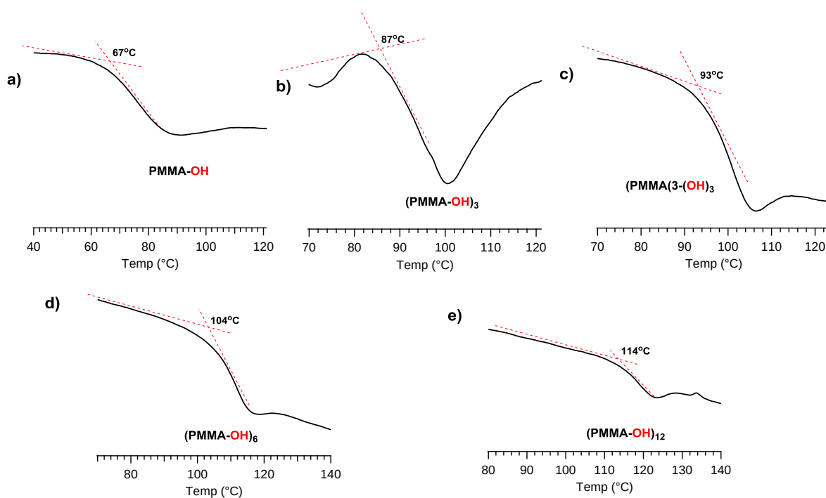
Figure 4.9 DSC thermograms of linear and star-shaped hydroxyl-functionalized PMMA
