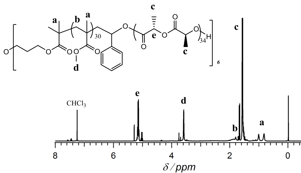
Figure 4.7 ^1\text{H} NMR spectrum of (\text{PMMA}_{30}\text{-}b\text{-PLLA}_{34})_6 in \text{CDCl}_3 (400 MHz).
