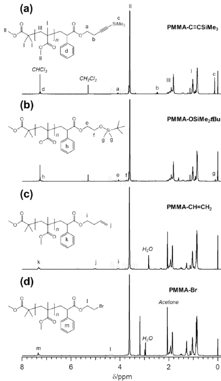
Figure 2.10. ^1\text{H} NMR spectra of (a) PMMA-C \equiv CSiMe _3 (Run 26, M_{n,\text{SEC}} = 3,460 ; M_w/M_n = 1.07 ) in CDCl _3 , (b) PMMA-OSiMe _2 tBu (Run 27, M_{n,\text{SEC}} = 3,250 ; M_w/M_n = 1.06 ) in CDCl _3 , (c) PMMA-CH=CH _2 (Run 28, M_{n,\text{SEC}} = 3,730 ; M_w/M_n = 1.07 ) in acetone- d_6 , and (d) PMMA-Br (Run 29, M_{n,\text{SEC}} = 3,690 ; M_w/M_n = 1.07 ) in acetone- d_6 .
