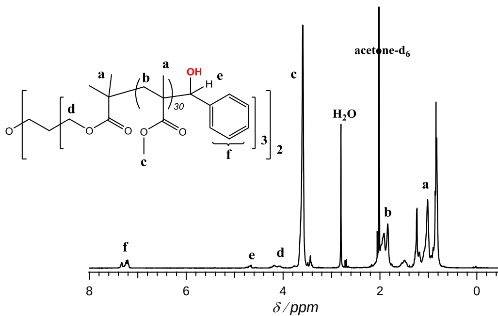
Figure 3.3. ^1\text{H} NMR spectrum of hydroxyl end-functionalized 6-arm star-shaped PMMA in acetone- d_6 (400 MHz).
