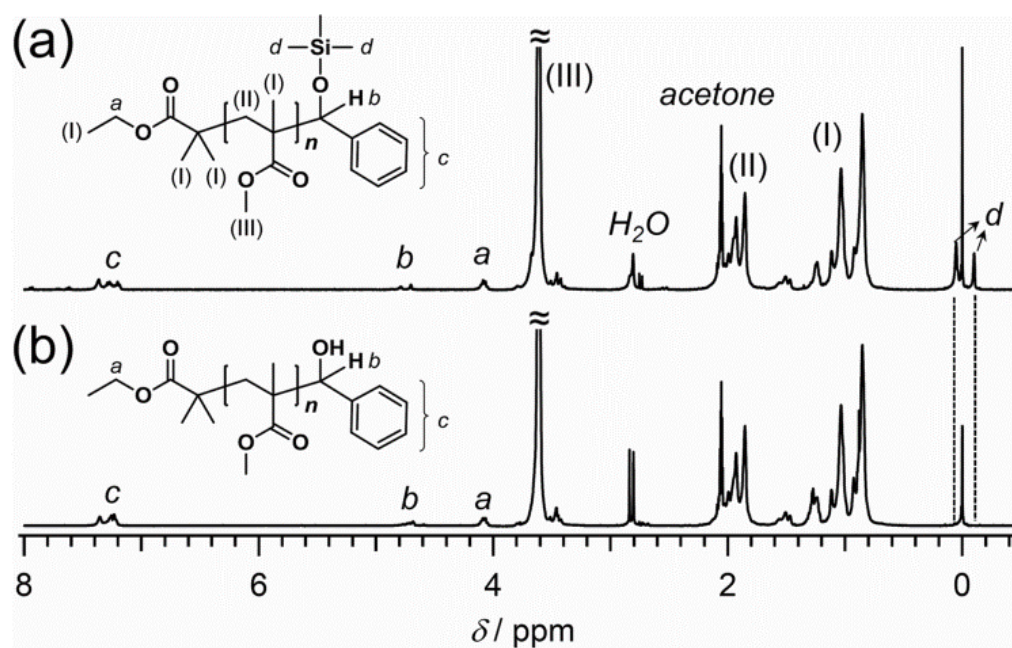
Figure 2.12. 1 H NMR spectra of (a) PMMA-OSiMe 3 obtained from Run 35 and (b) PMMA-OH obtained from Run 35 in acetone- d 6 .
