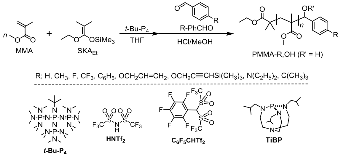
Scheme 2.2 Synthesis of \omega -end-functionalized poly (methyl methacrylate) by organocatalytic GTP using benzaldehyde terminators.
