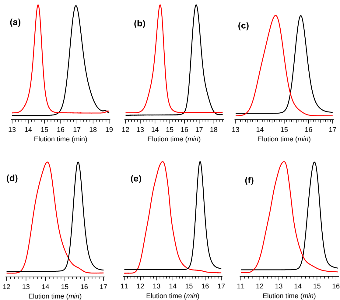
Figure 4.4 SEC traces of (a) PMMA 30 -b-PLLA 30 (black line) and its precursor of PMMA 30 -OH (red line), (b) (PMMA 30 -b-PLLA 30 ) 3 (black line) and its precursors of (PMMA 30 -OH) 3 (red line), (c) (PMMA 30 -b-PLLA 15 ) 6 (black line) and its precursors of (PMMA 30 -OH) 6 (red line), (d) (PMMA 30 -b-PLLA 30 ) 6 (black line) and its precursors of (PMMA 30 -OH) 6 (red line), (e) (PMMA 30 -b-PLLA 60 ) 6 (black line) and its precursors of (PMMA 30 -OH) 6 (red line) and (f) (PMMA 30 -b-PLLA 30 ) 12 (black line) and its precursors of (PMMA 30 -OH) 12 (red line)
