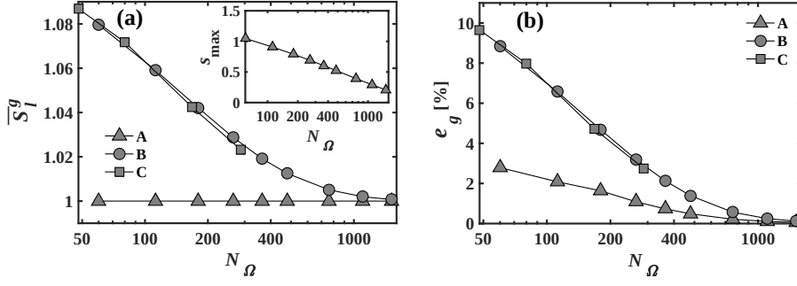
Fig. 3 (a) Mean values of S_l^g , \bar{S}_l^g , for Methods A, B, and C as listed in Table 1 with g = 0.9 at different values of N_\Omega in a logarithmic scale and s_{max} (Eq. (11)) is plotted in the inset. (b) Mean absolute percentage error, e_g of S_l^g for the three methods with g = 0.9 .
