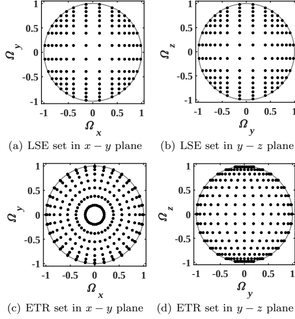
Fig. 1 Discrete angular directions in x-y and y-z planes for the LSE set ( N_\Omega = 288 ) ((a) and (b)) and ETR set ( N_\Omega = 480 ) ((c) and (d)). Dots are the discrete angular directions, and circles are boundaries of the unit sphere
