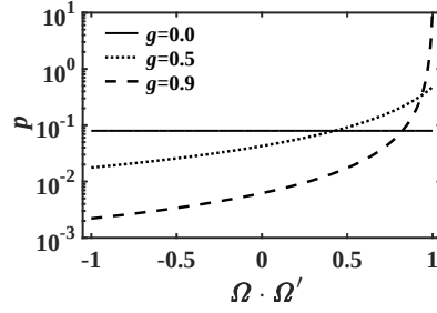
Fig. 2 Henyey-Greenstein phase function as a function of \Omega \cdot \Omega' for isotropic scattering ( g = 0.0 ), moderately forward-peaked scattering ( g = 0.5 ), and high forward-peaked scattering ( g = 0.9 ), in logarithmic scale
