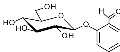
Helicin
