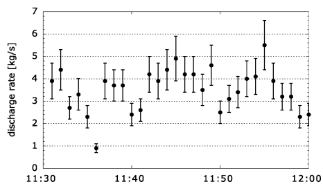
Fig. 6. Discharge rate of \text{SO}_2 gas obtained from the snapshots shown in Fig. 5. Ascent velocity is assumed to be 10–15 m/s. Error range corresponds to that of the ascent velocity.
