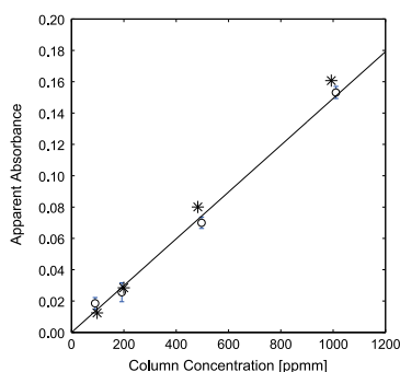
Fig. 2. Apparent absorbance with respect to the column concentration of calibration cells. Error range indicates 1\sigma of 100 \times 100 pixels. Asterisks indicate the values from Mori and Burton (2006).
