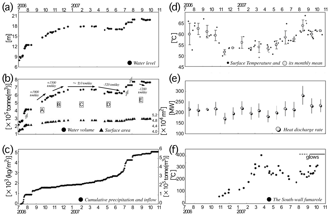
Fig. 3. (a) Water level and (b) water mass (volume) and surface area of Yudamari crater lake. (c) Cumulative precipitation and cumulative income due to precipitation, the equivalent catchment area of 1.1 \times 10^5 \text{ m}^2 is taken into account (see text for details). (d) Temperature of the lake surface measured by JMA's IR thermometry. Small dots represent each measurement, whereas the gray circles represent monthly means with the square root of the standard deviations. (e) Computed monthly mean heat discharge rate from the lake surface. (f) Temperature of the south-wall fumaroles measured by JMA's IR thermometry.
