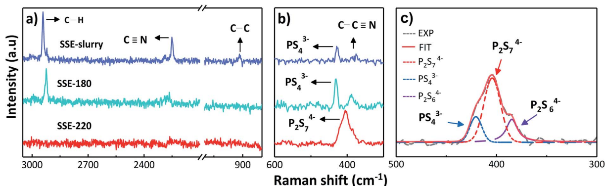
Fig. 3 Raman spectra of the 74\text{Li}_2\text{S} \cdot 26\text{P}_2\text{S}_5 sulfide electrolyte in the range of (a) 3050–850 \text{cm}^{-1} and (b) 600–300 \text{cm}^{-1} . Blue, green and red lines represent SSE-slurry, SSE-180 and SSE-220 samples, correspondingly. (c) Spectral decomposition of Raman spectrum for the SSE-220 sample. Dashed grey line, experimental data; continuous orange line, the fitting result for all \text{PS}_x polyhedral; dashed red, blue and violet lines, \text{P}_2\text{S}_7^{4-} , \text{PS}_4^{3-} and \text{P}_2\text{S}_6^{4-} units, correspondingly.
