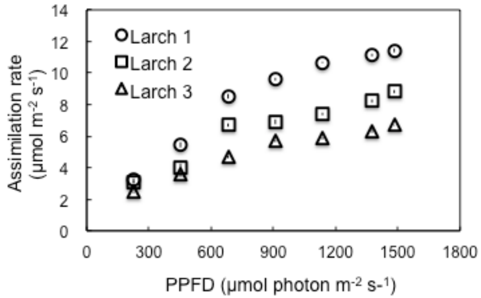
Fig. 2.2. Relationship between the assimilation rate and photosynthetic photon flux density (PPFD) for three larch trees. This measurement was made as preparatory measurement with different trees from those used in the present experiments.
