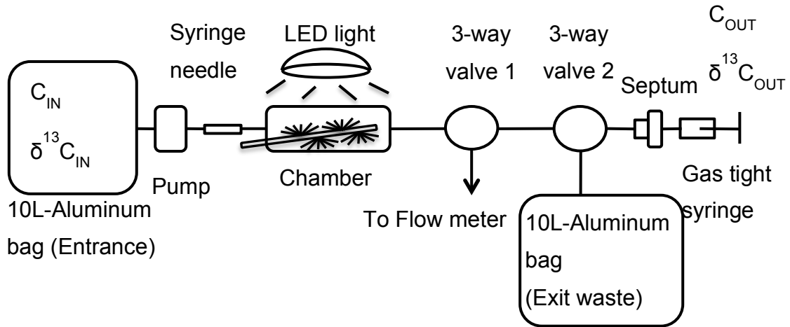
Figure 2.1. Chamber system used for assimilation and discrimination measurements in the waterlogging experiment. Air was pumped from a 10-L entrance aluminum bag to an exit waste bag through a chamber in which the larch stem was enclosed. Air samples were taken 3–5 times every 15 minutes at the exit using a gas-tight syringe. Flow rate was controlled at around 5.0 \times 10^{-4} \text{ L s}^{-1} using a pump coupled with syringe needles. Photosynthetic photon flux density (PPFD) of light from an LED source was set at 1500 \mu\text{mol m}^{-2} \text{s}^{-1} .
